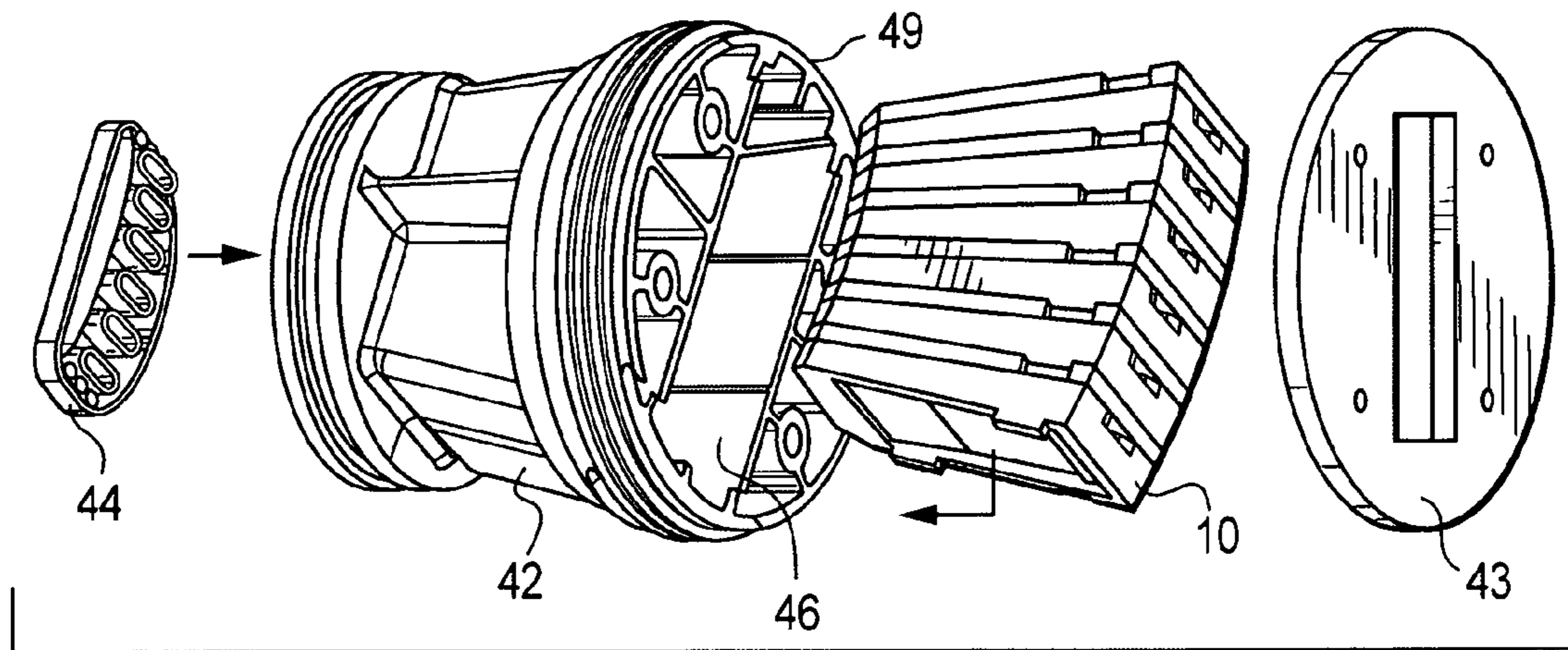
FIG. 5 (PRIOR ART)
