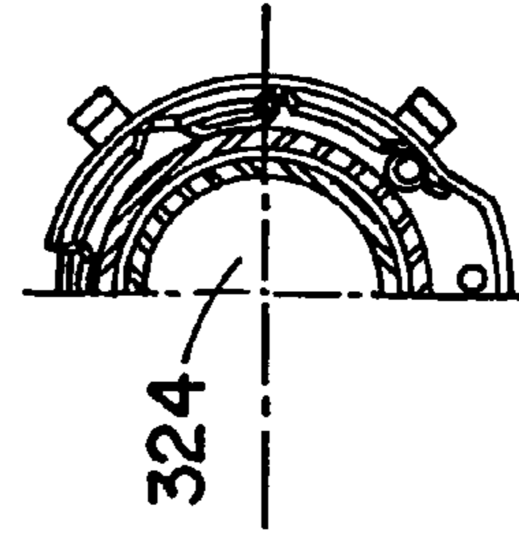
SECTION B-B
