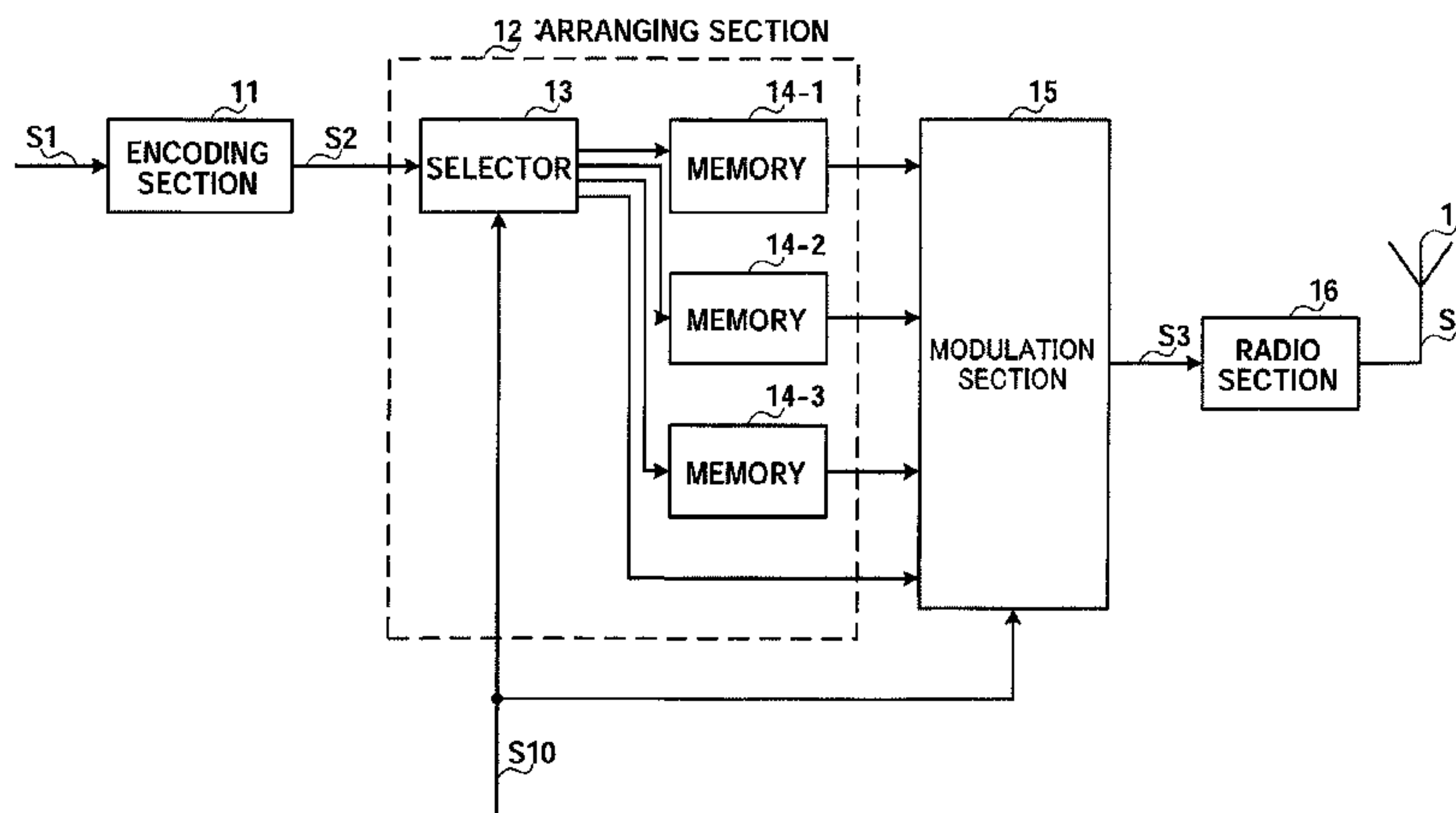
10 TRANSMITTING APPARATUS
