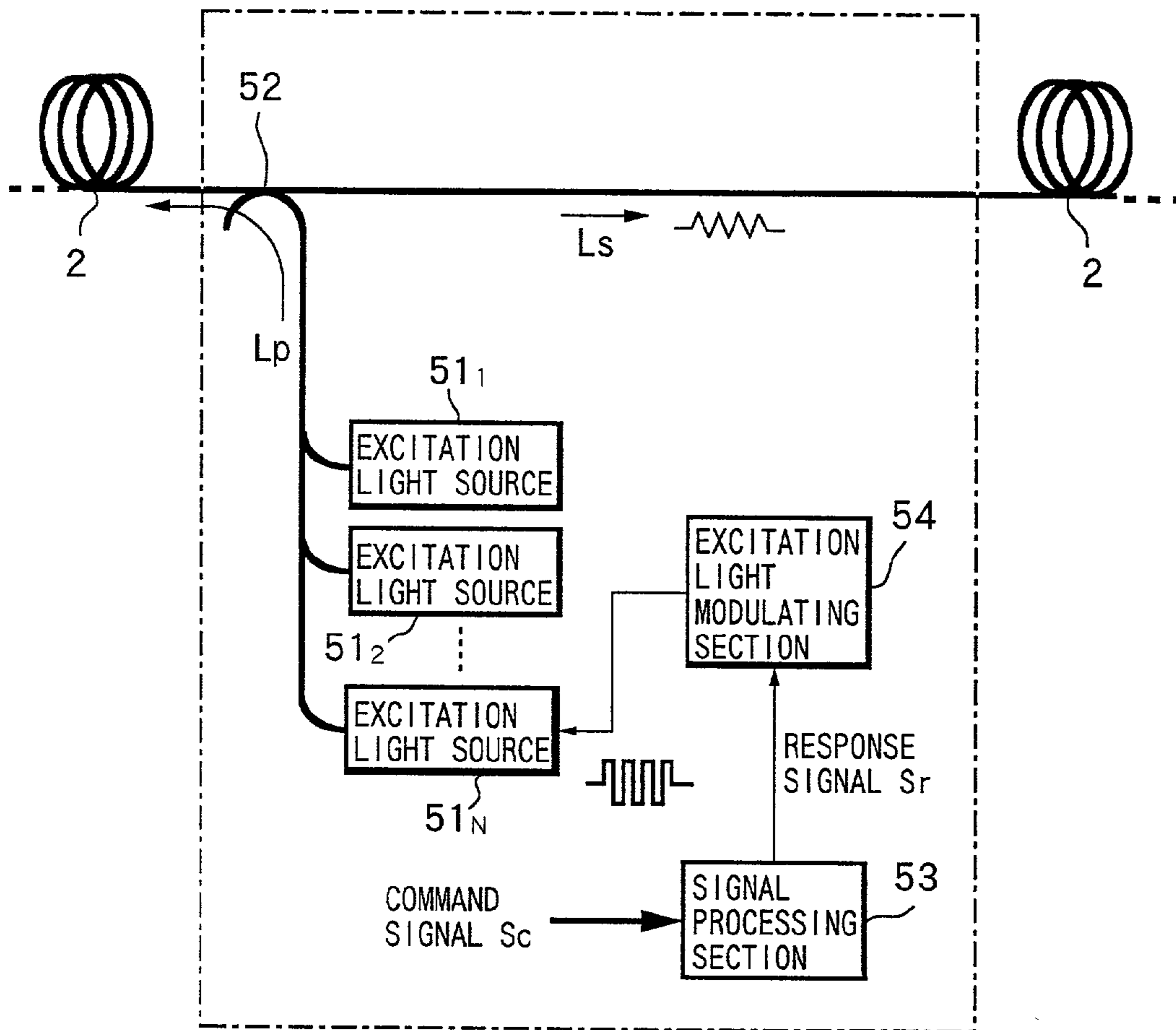
OPTICAL REPEATER 5
