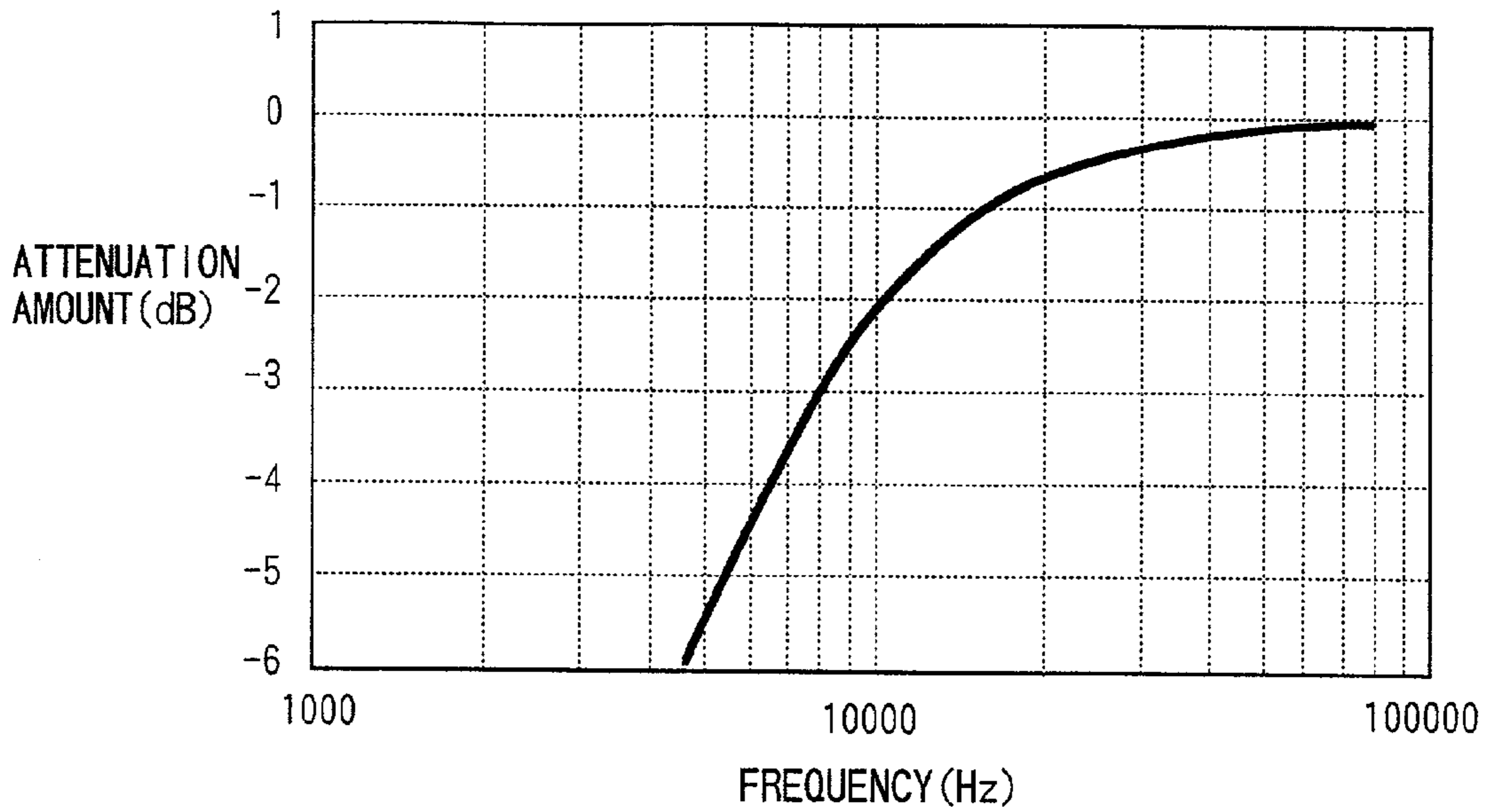
FREQUENCY CHARACTERISTIC OF TYPICAL EDFA
