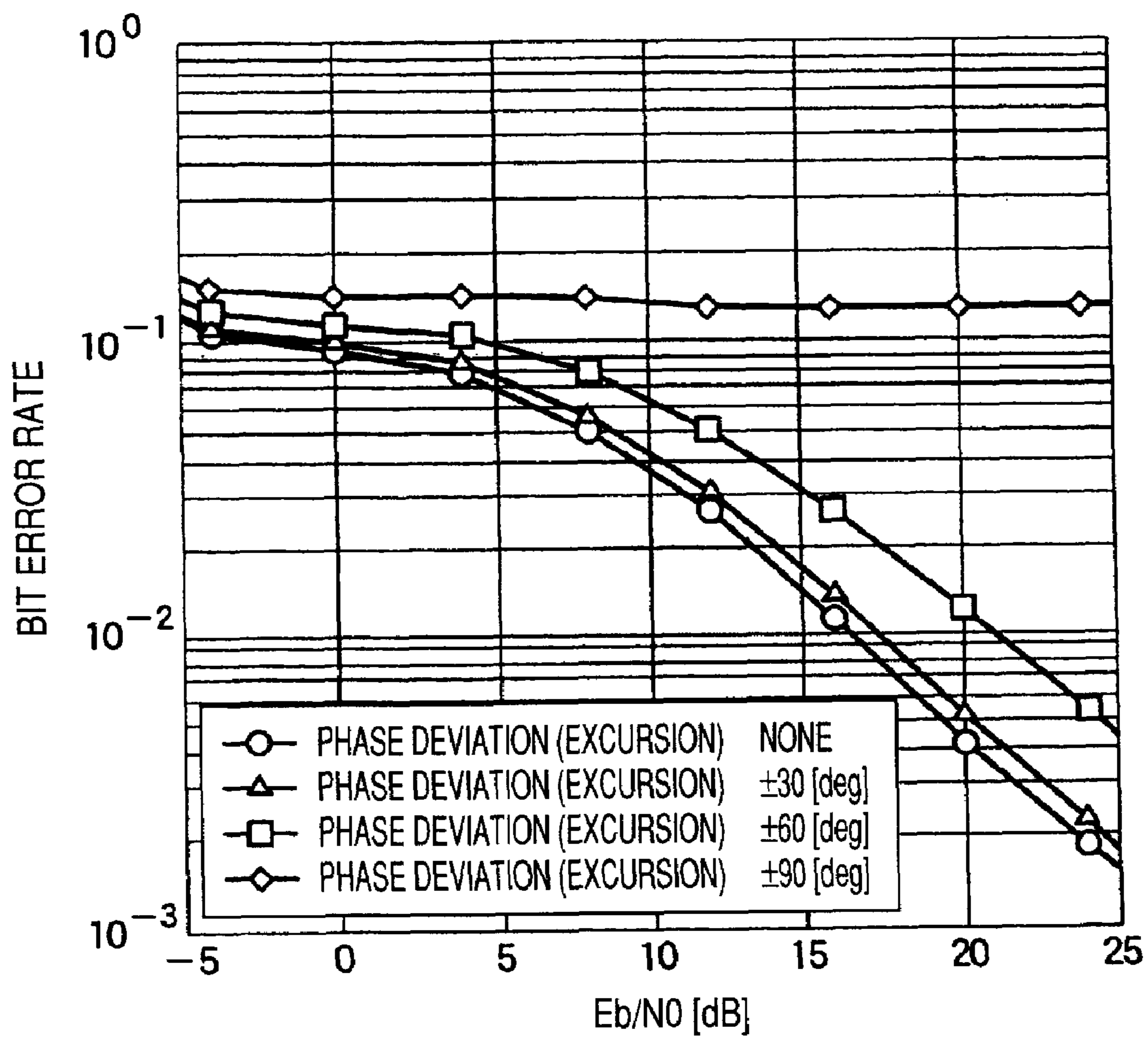
RECEPTION CHARACTERISTIC FOR E_b/N_0
