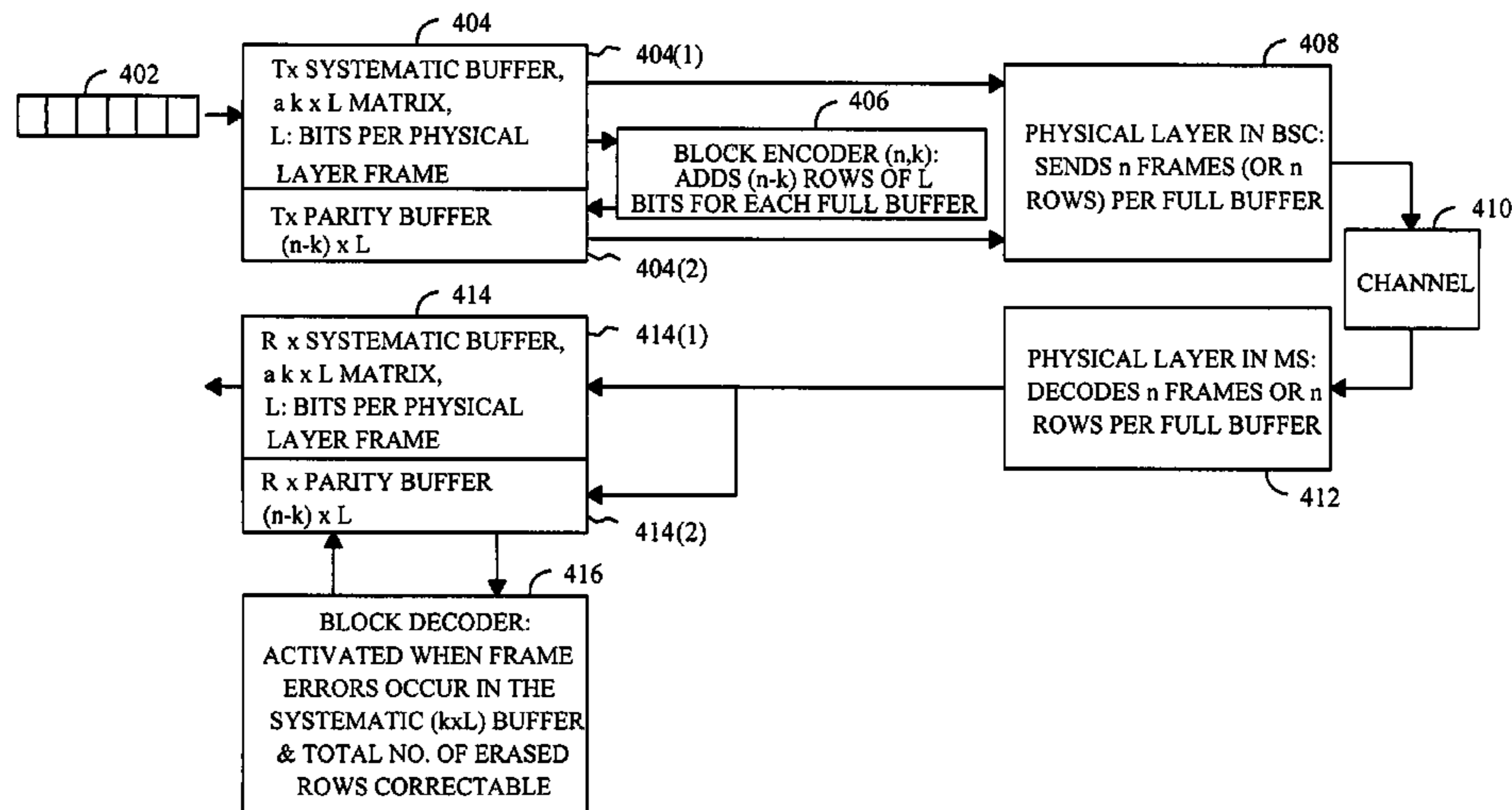
REED-SOLOMAN OUTER CODE BLOCK DIAGRAM
