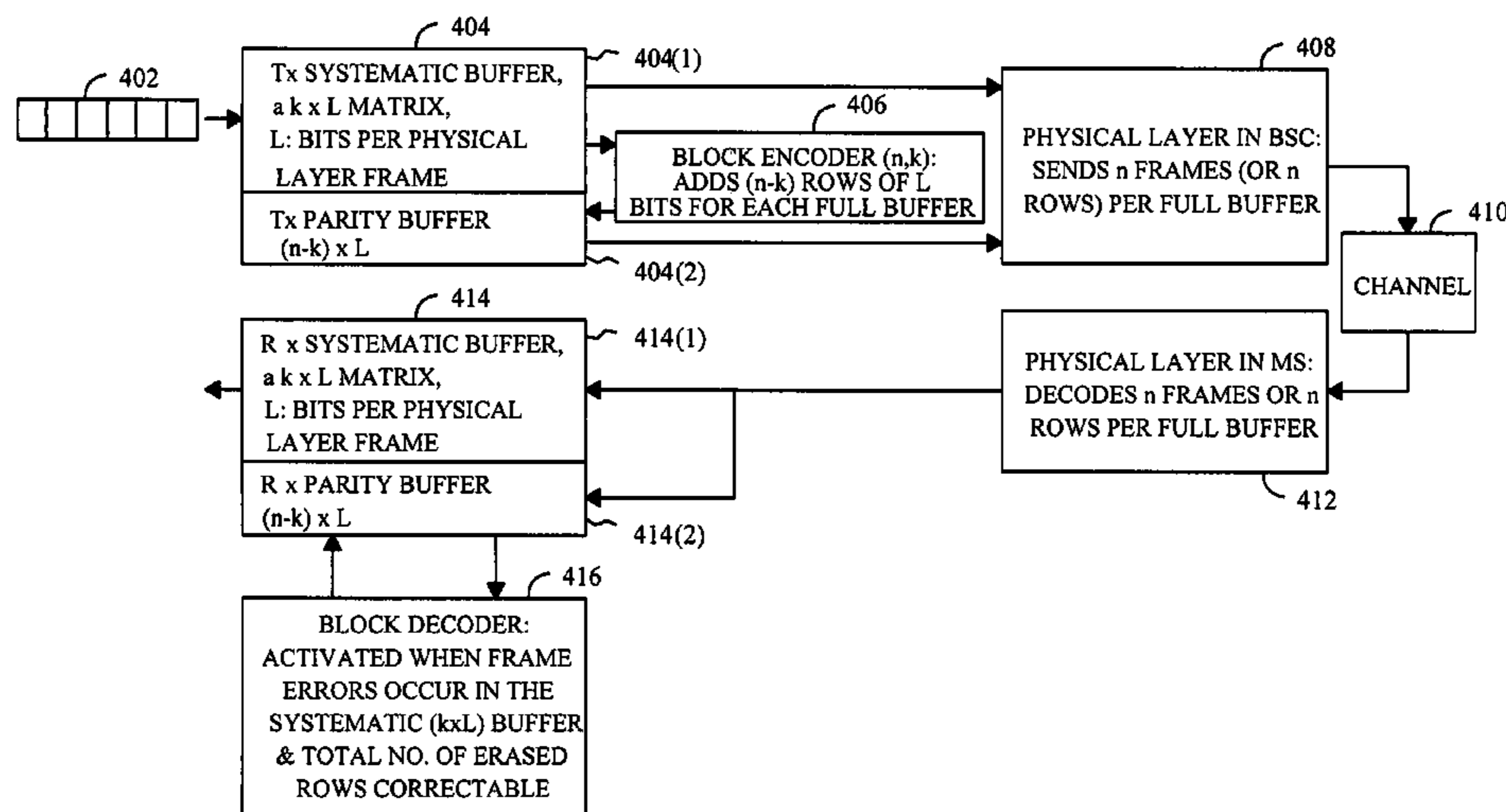
REED-SOLOMAN OUTER CODE BLOCK DIAGRAM
