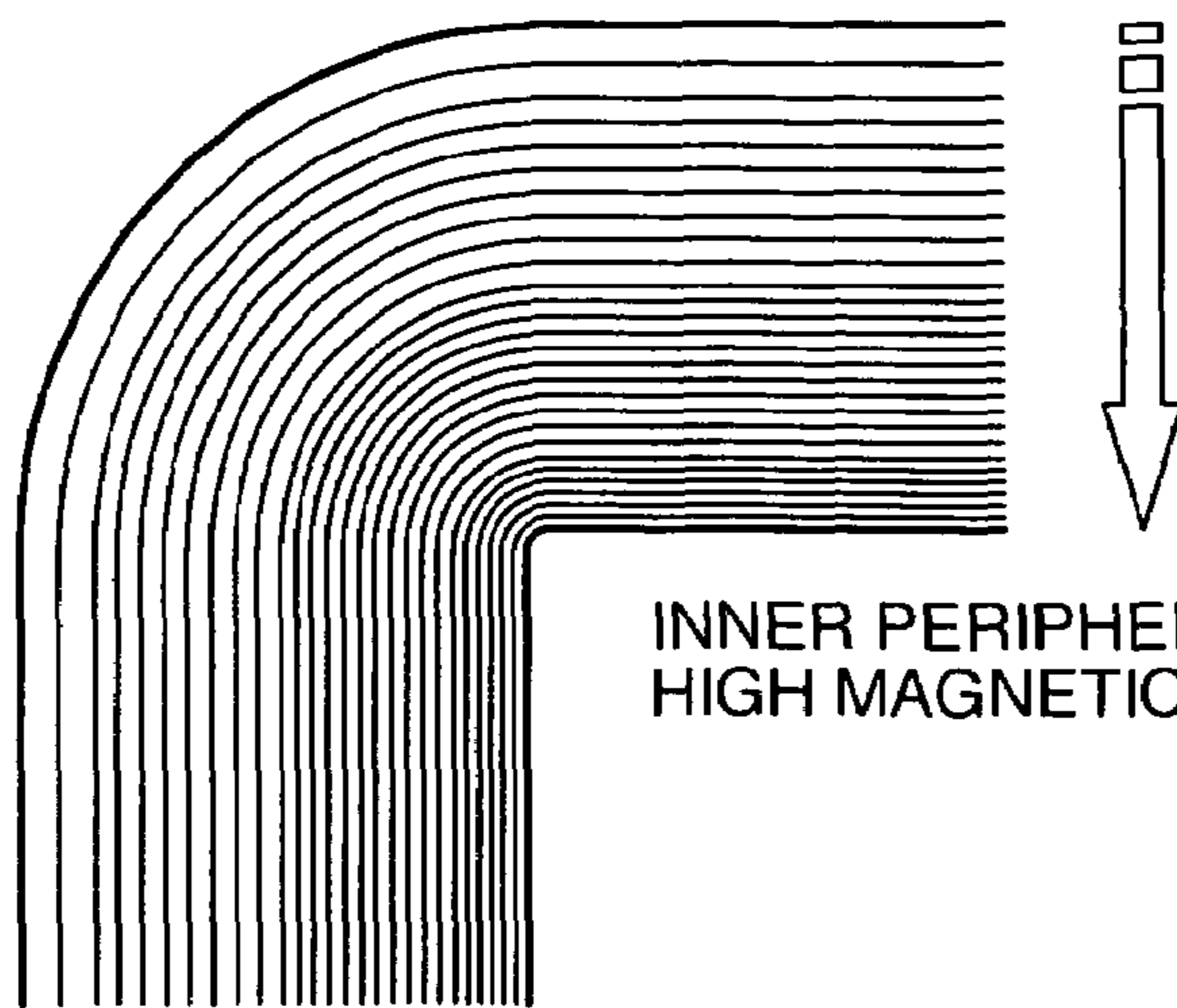
DETAILED DRAWING OF PART A (DRAWING OF WOUND IRON CORE MAGNETIC FLUX DISTRIBUTION)
