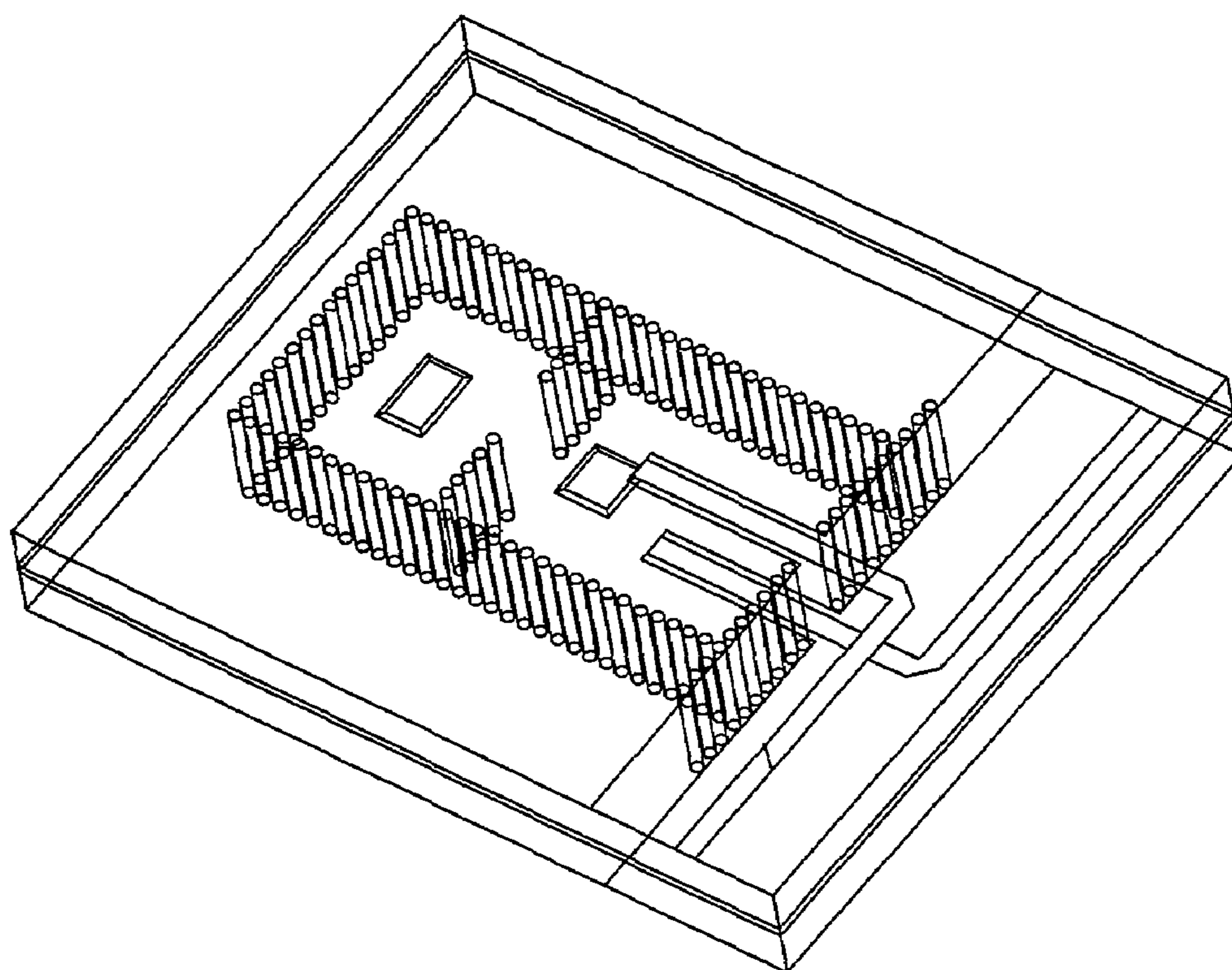
FIG. 4 (PRIOR ART)
