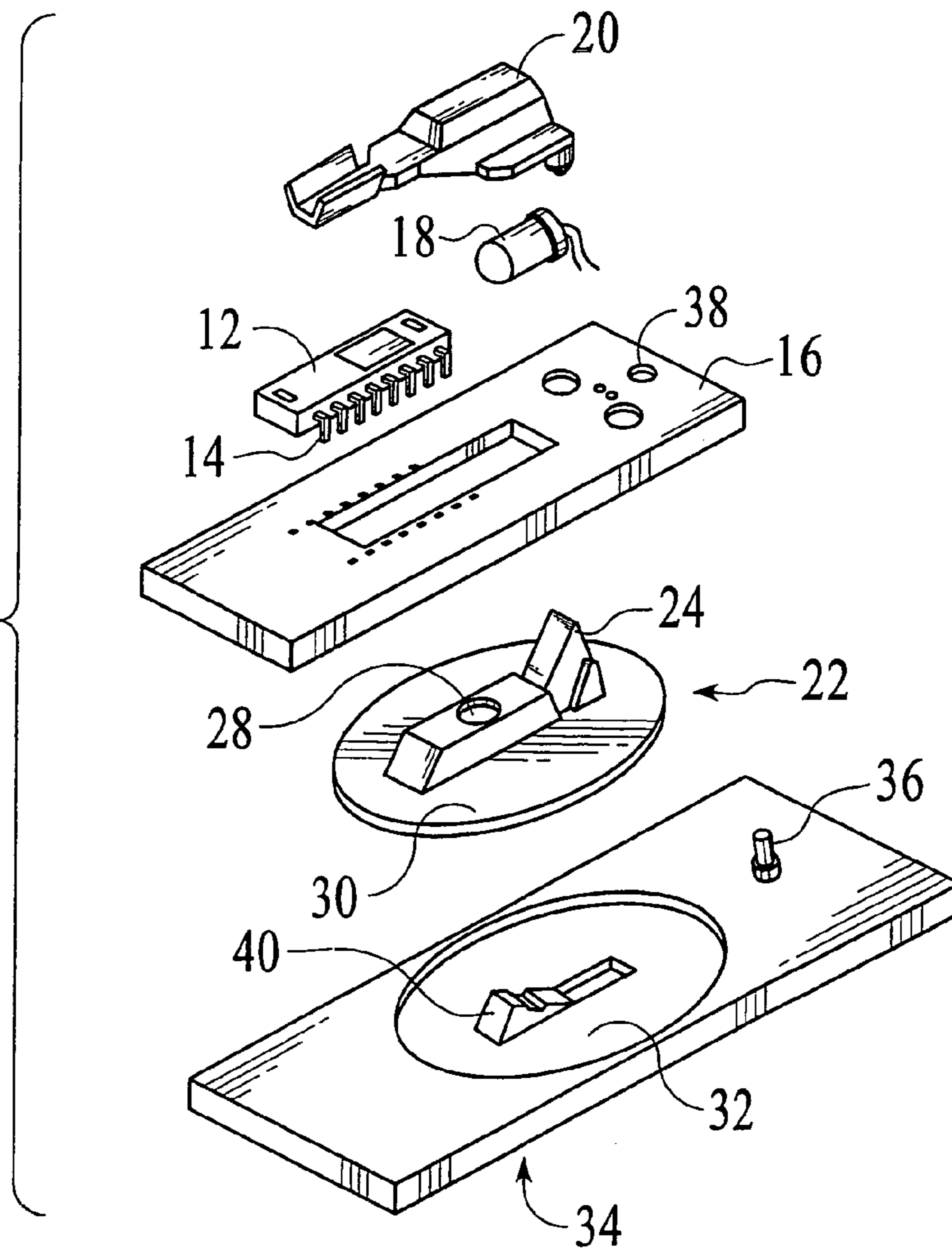
FIG.2 (PRIOR ART)
