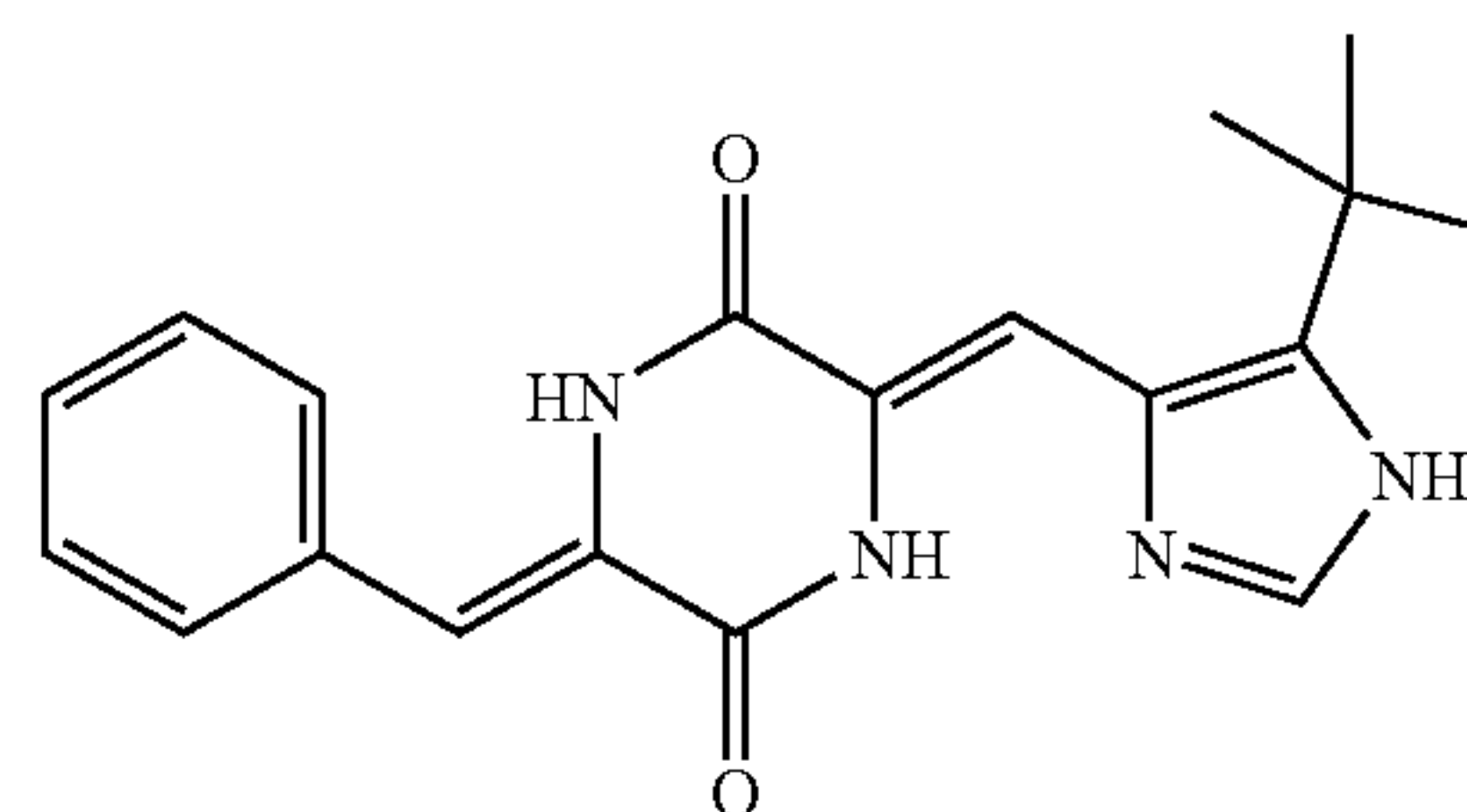
tBu-dehydrophenylahistin
