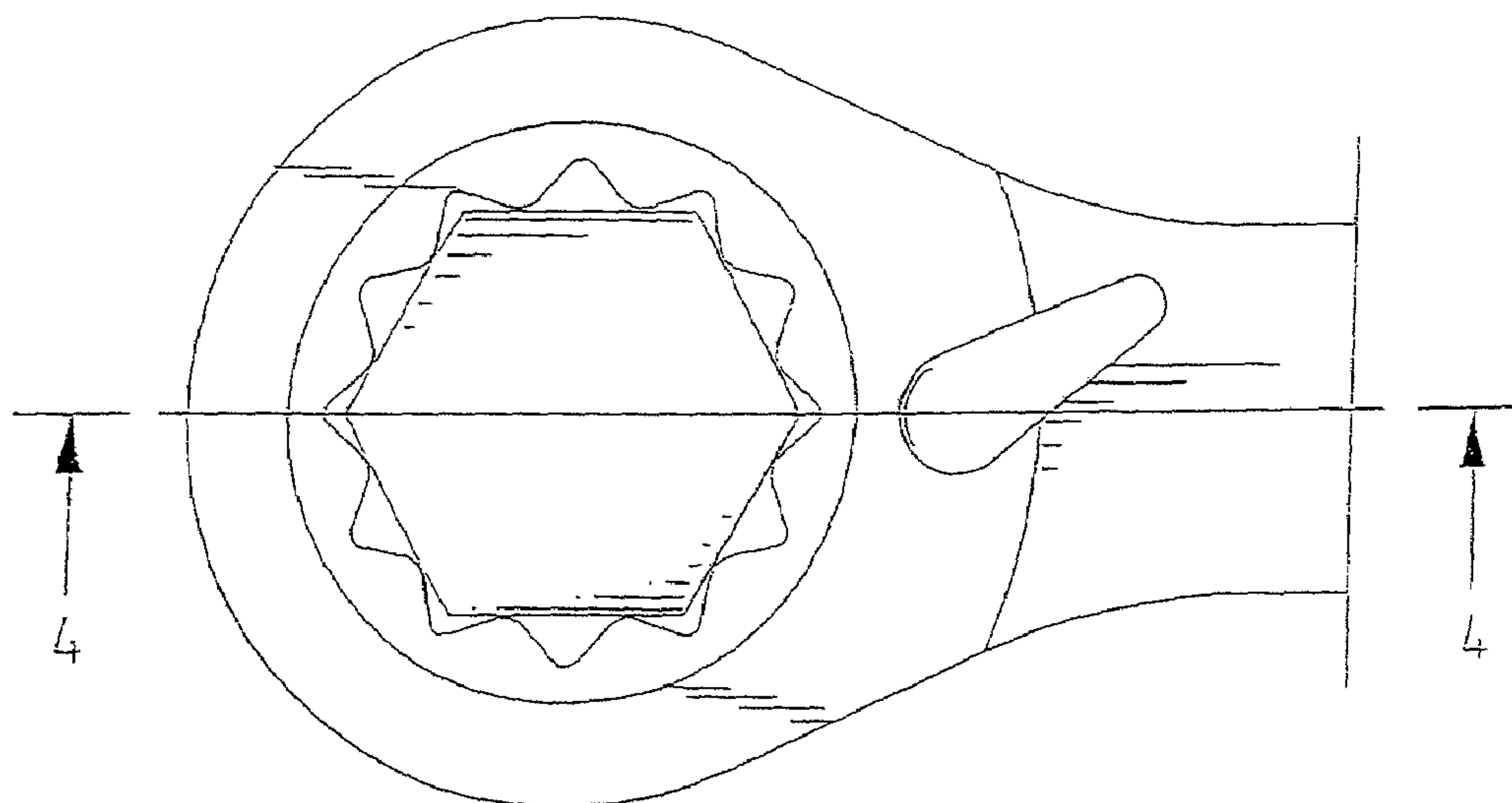
Fig. 3 PRIOR ART
