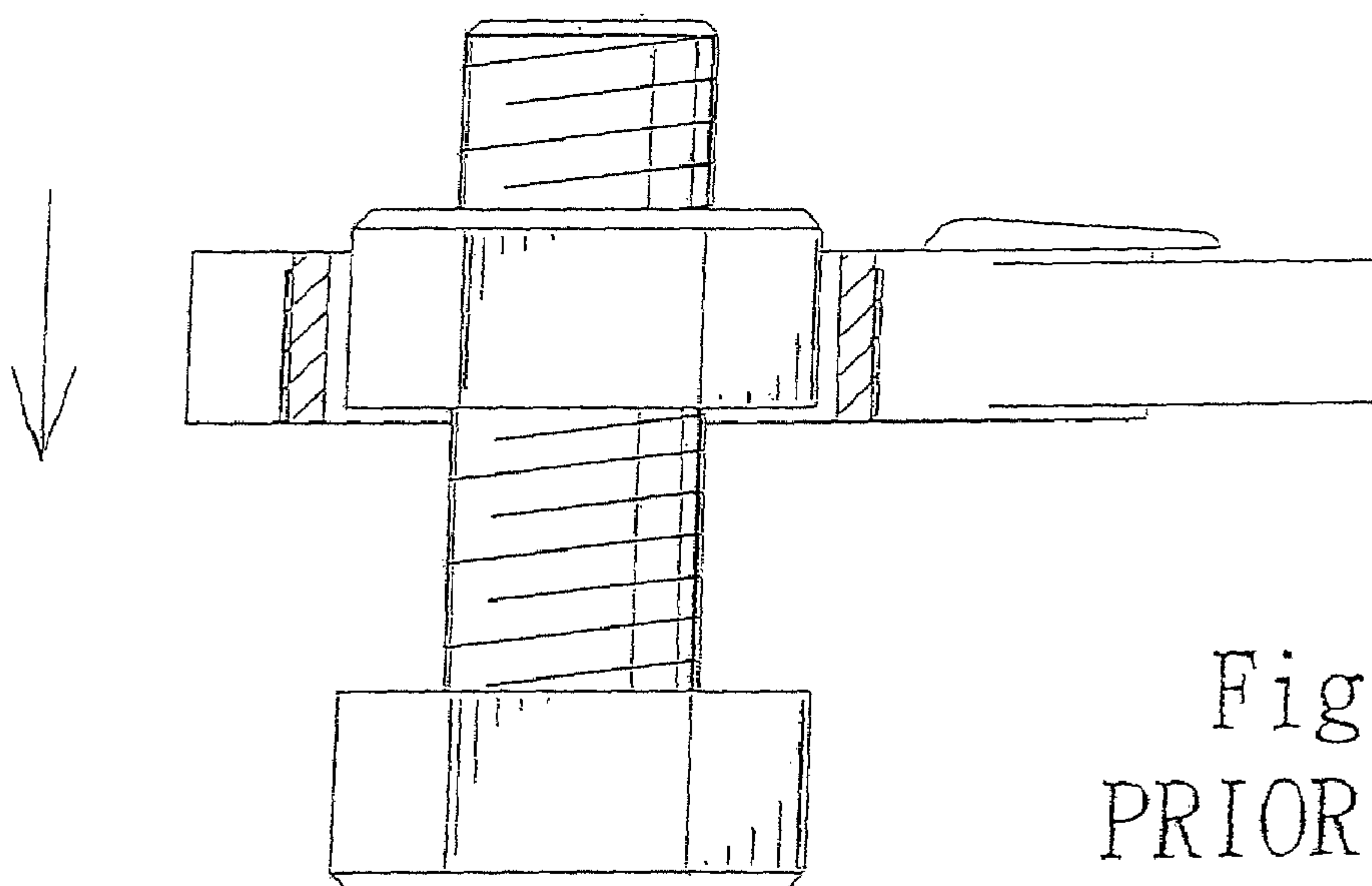
Fig. 3 PRIOR ART
