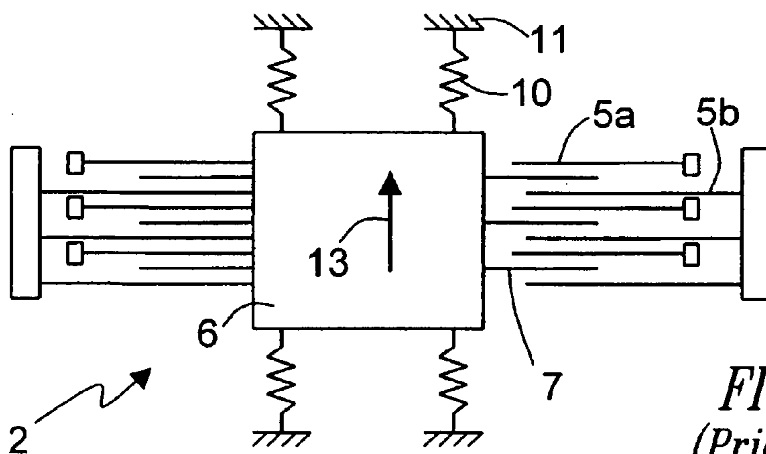
FIG. 1 (Prior Art)
