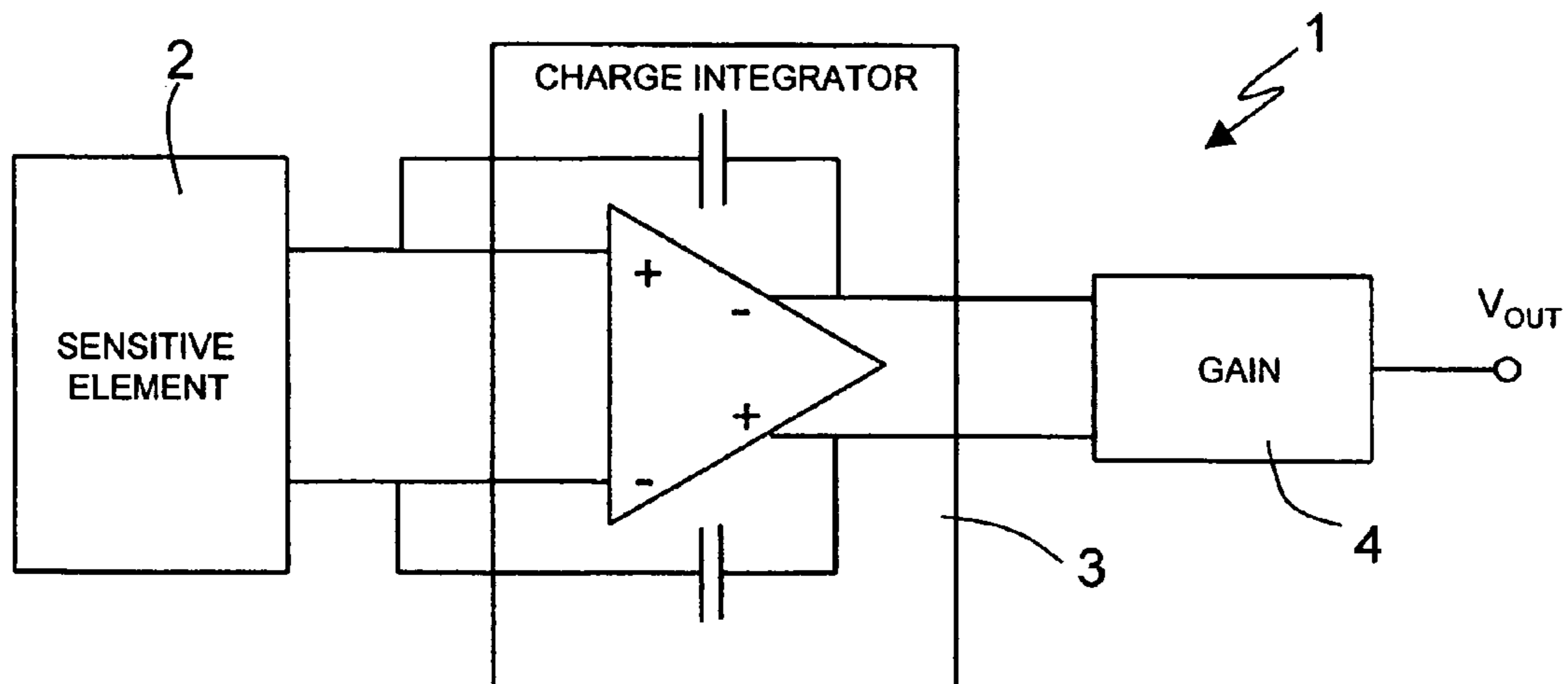
FIG. 1 (Prior Art)
