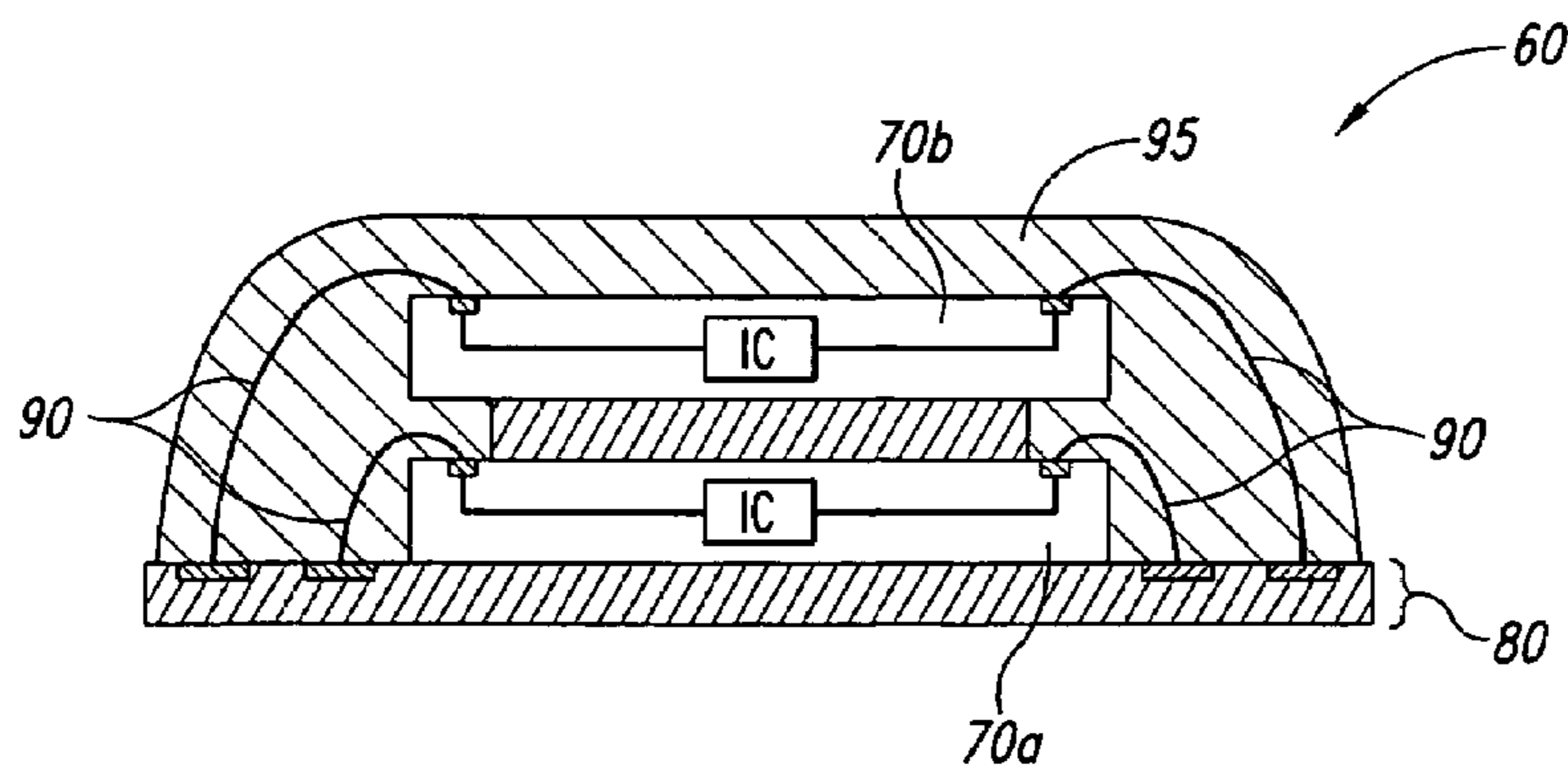
Fig. 2 (Prior Art)
