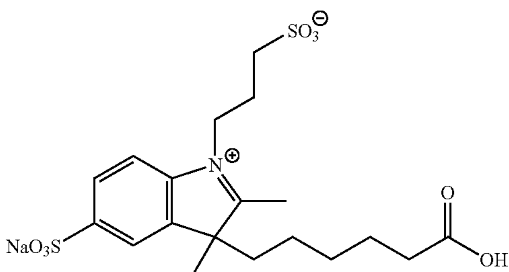
Compound 2
