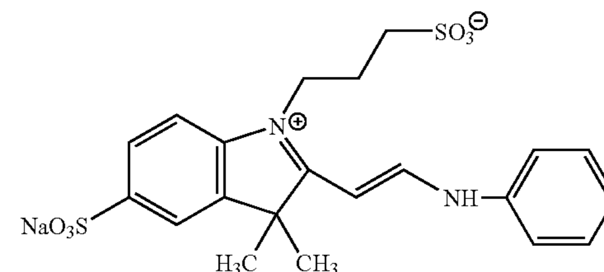
Compound 5
