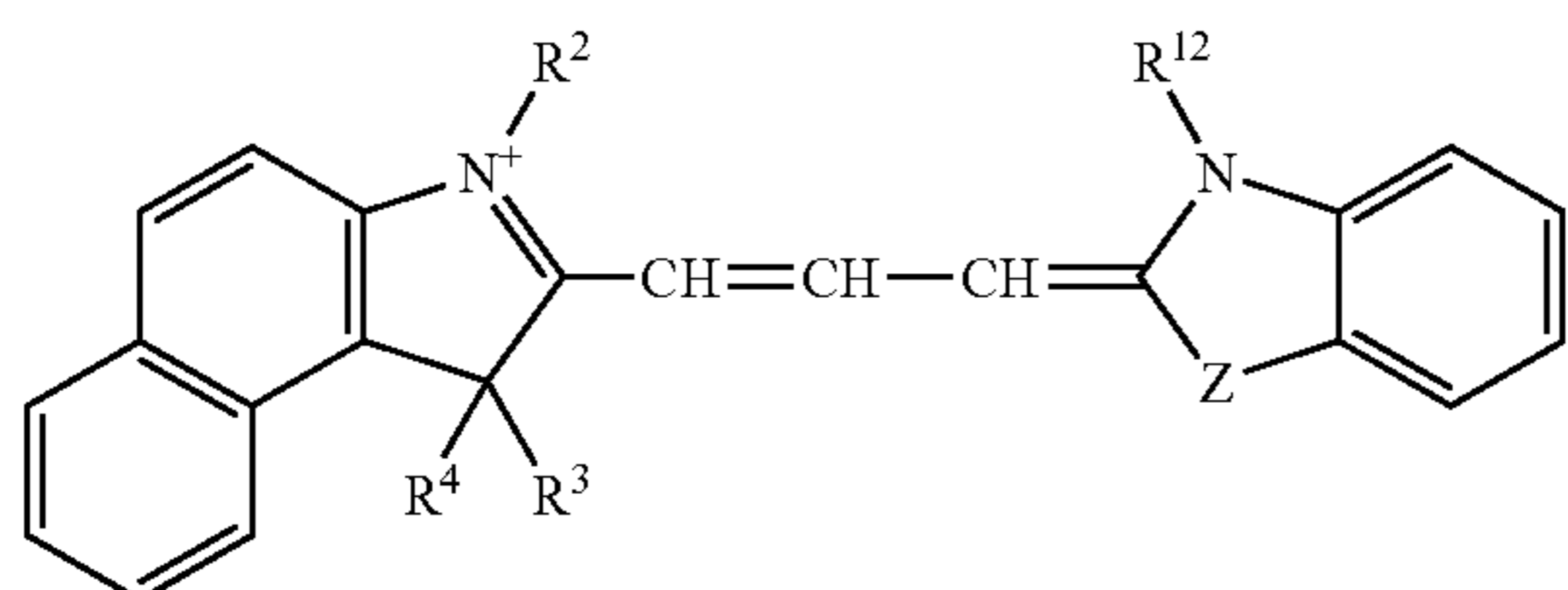
Formula XIII
