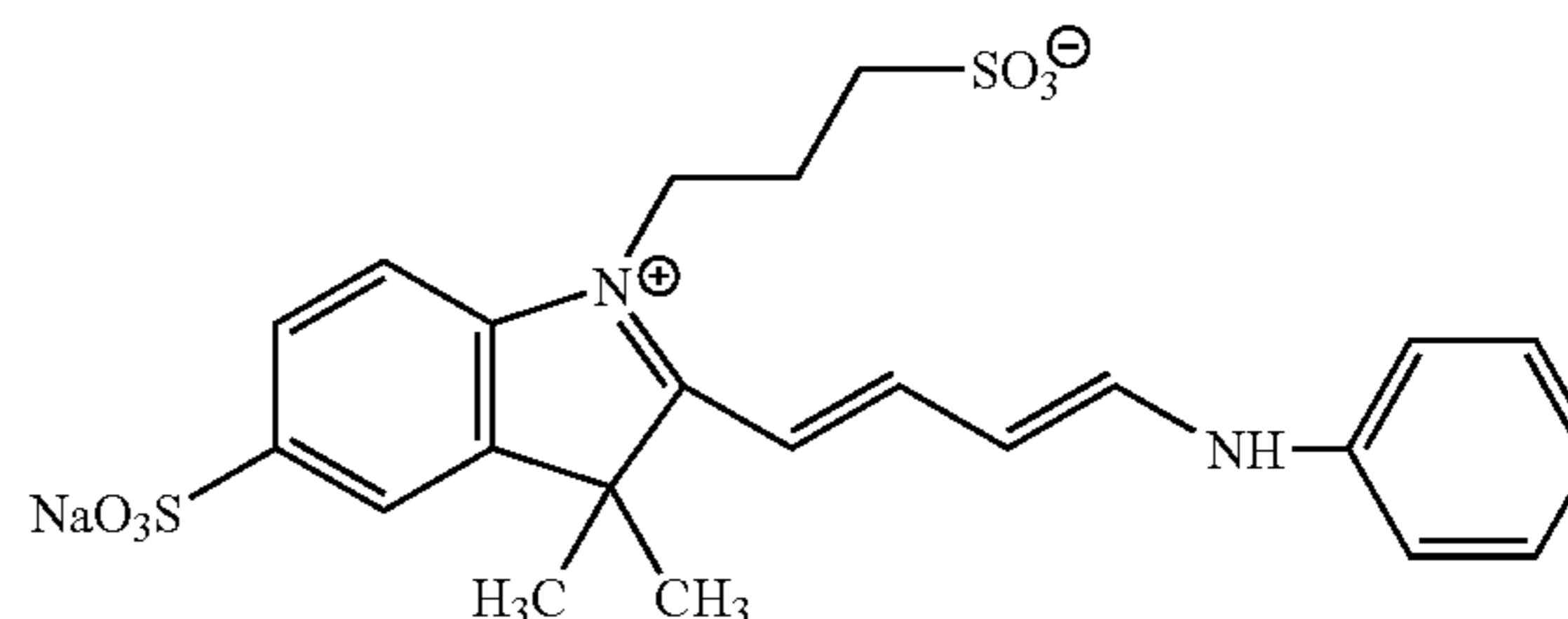
Compound 4
