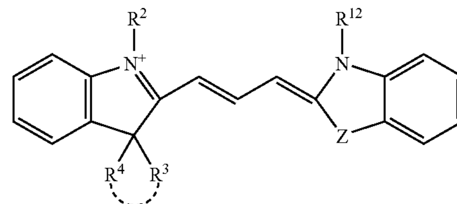
Formula XVIII
