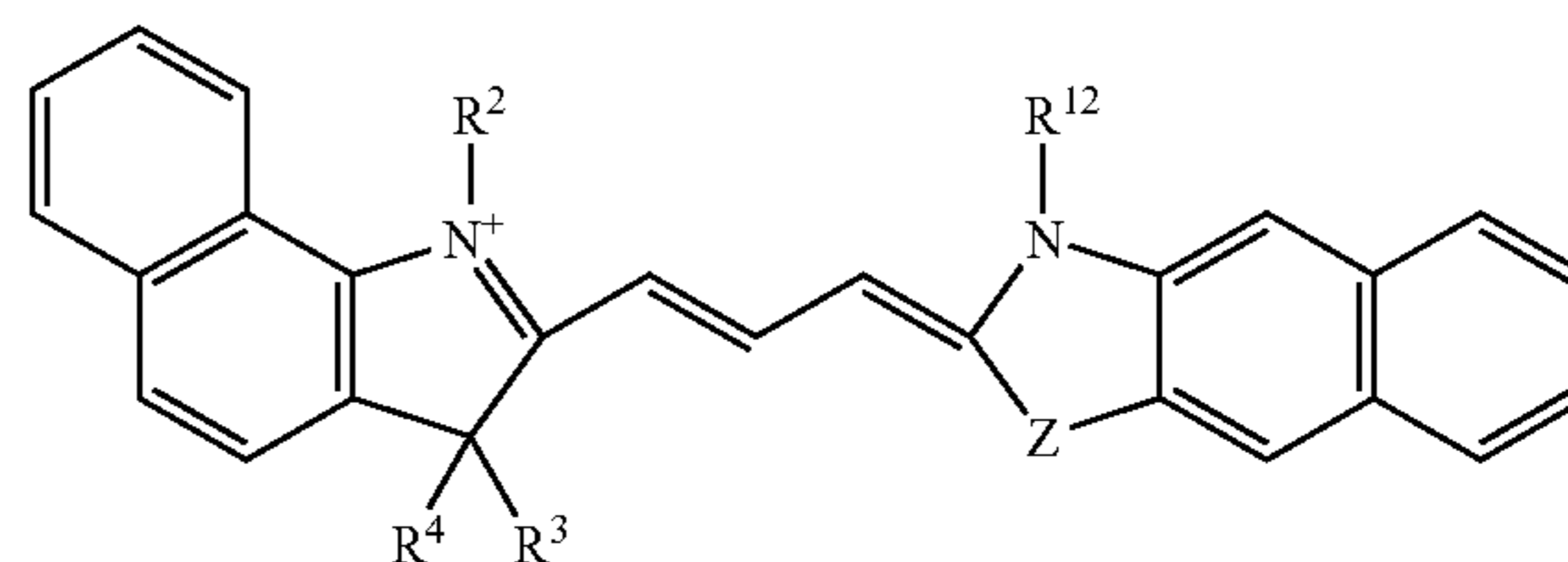
Formula XX
