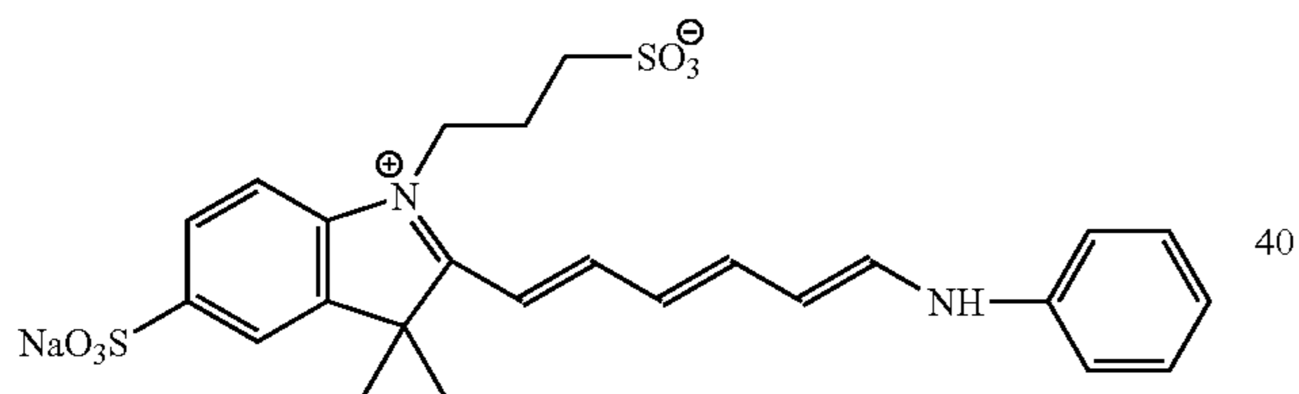
Compound 20 35
