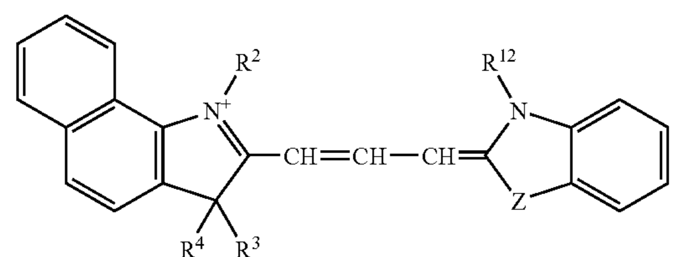
Formula XVI
