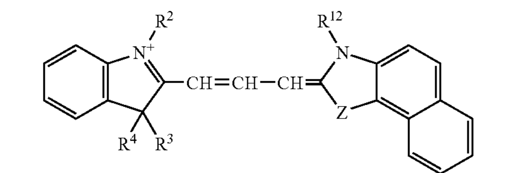
Formula XIII
