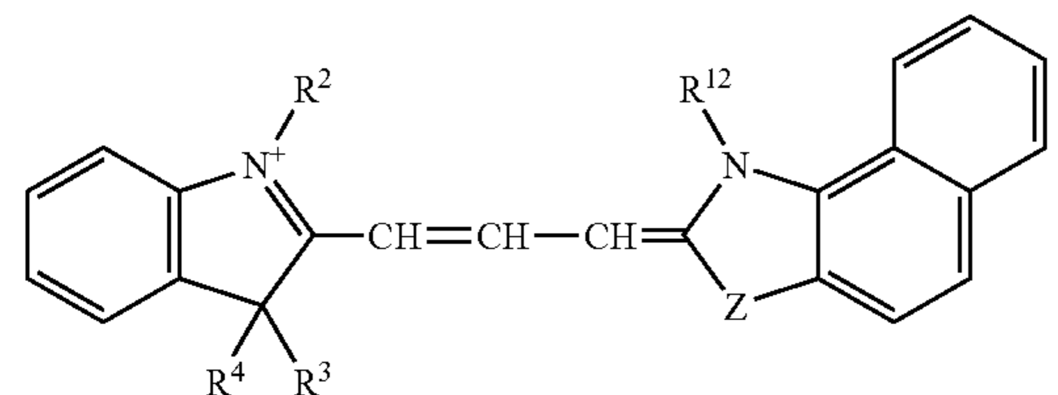
Formula XVII
