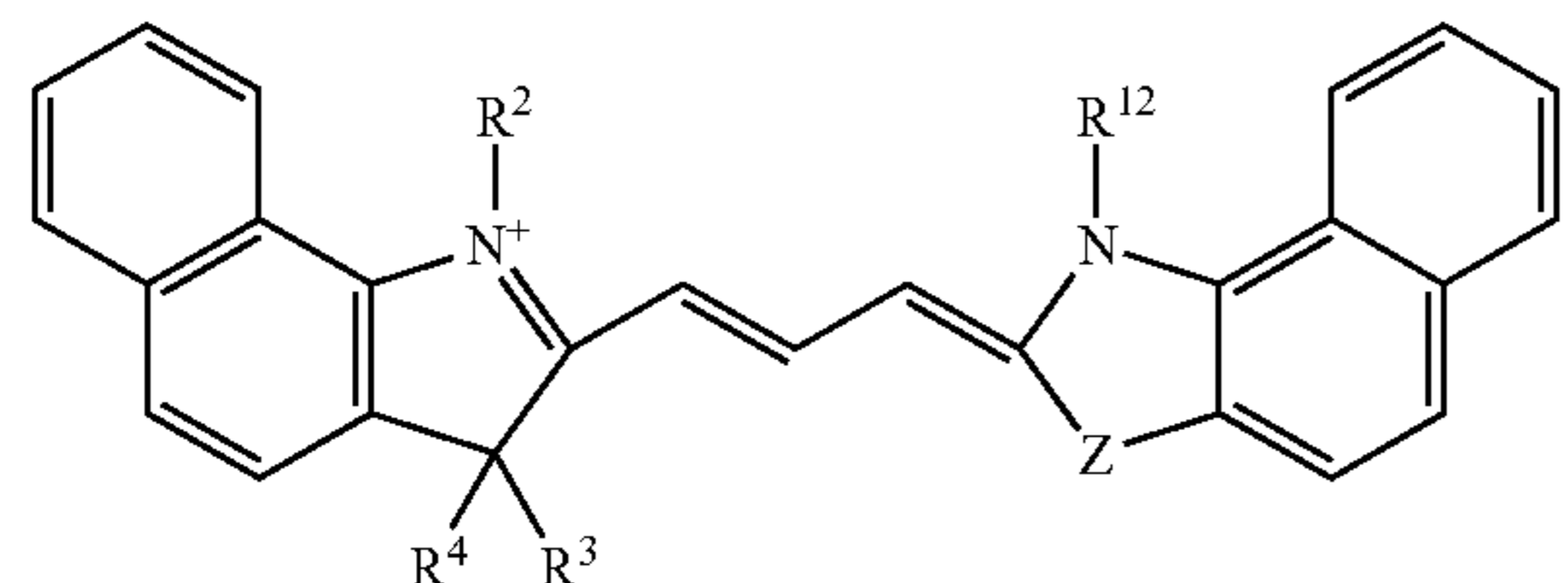
Formula XVII
