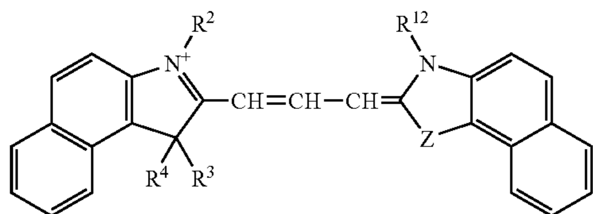
Formula XV
