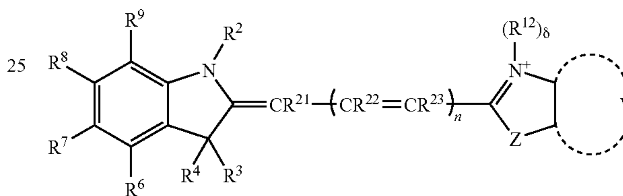
Formula XI
