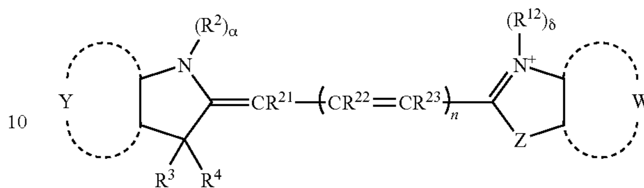
Formula X
