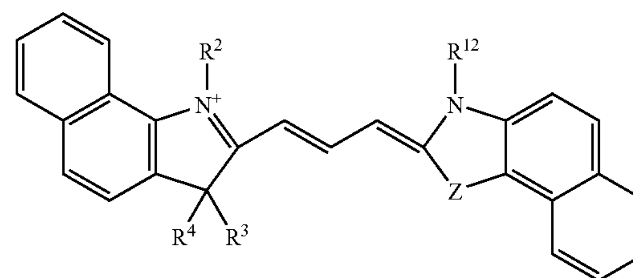
Formula XX
