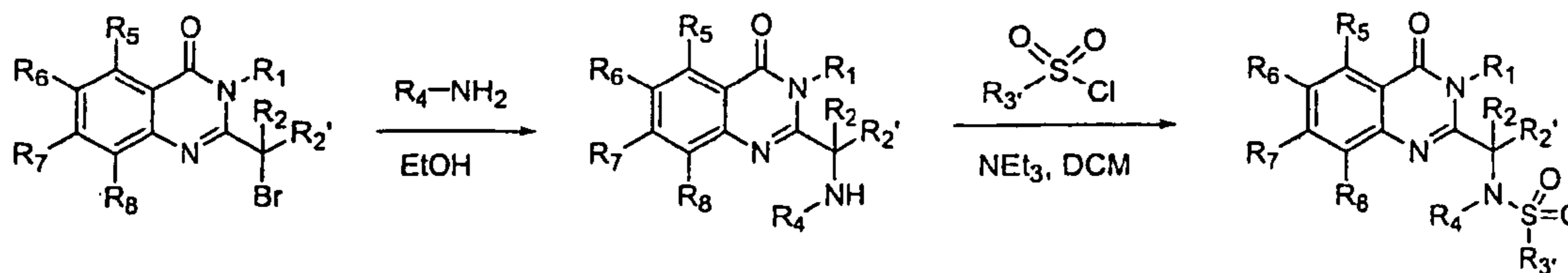
Figure 5a: Sulfonamide Synthesis
