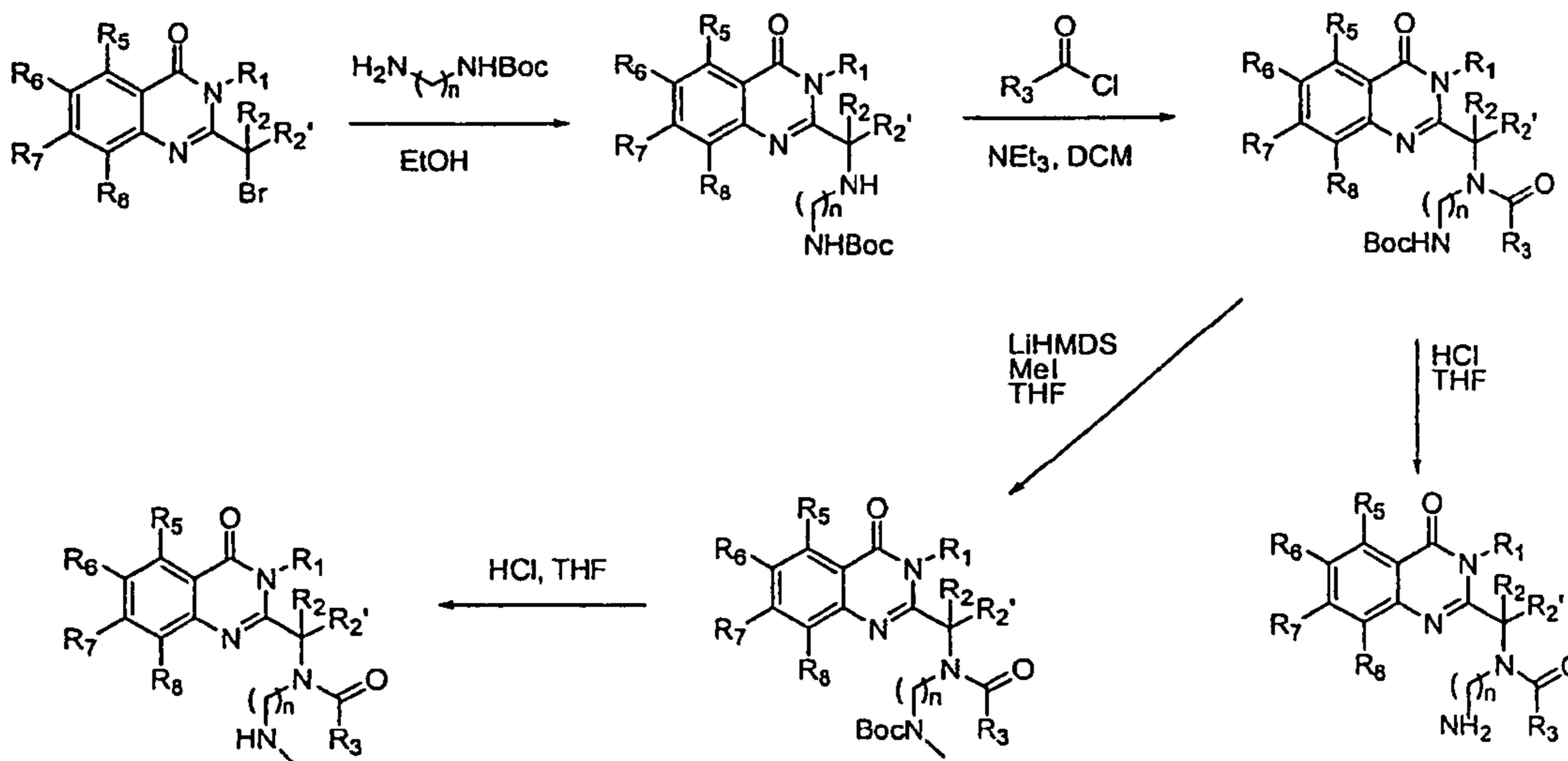
Figure 5d: Primary and Secondary Amine R4 Synthesis
