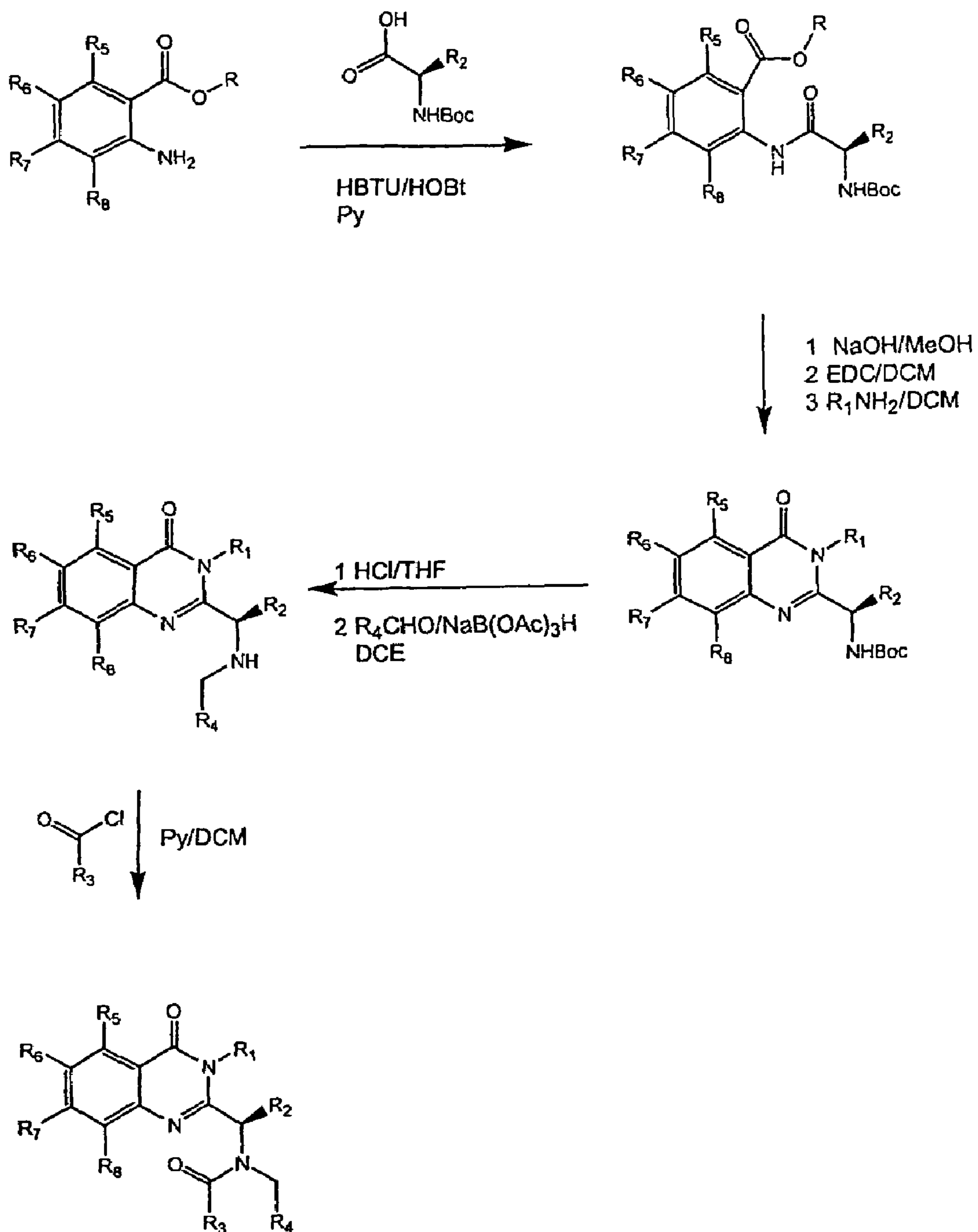
Figure 4: Asymmetric Synthesis
