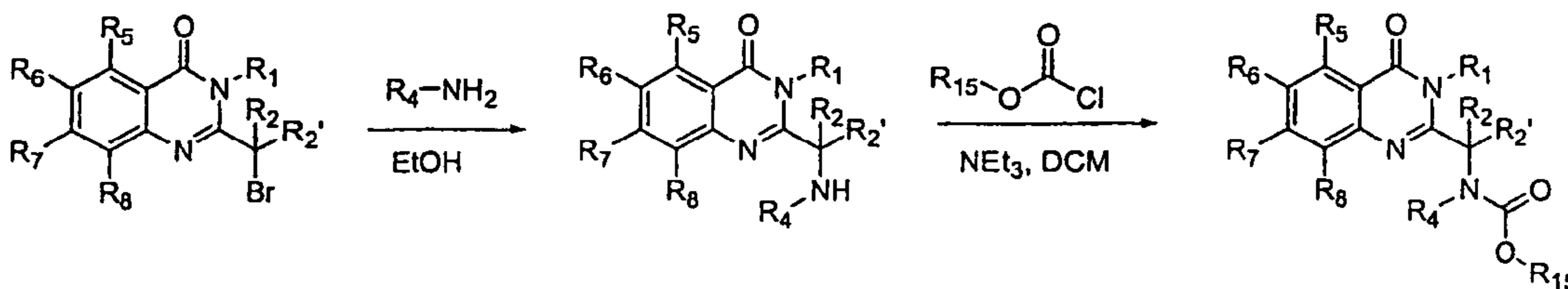
Figure 5c: Urea Synthesis
