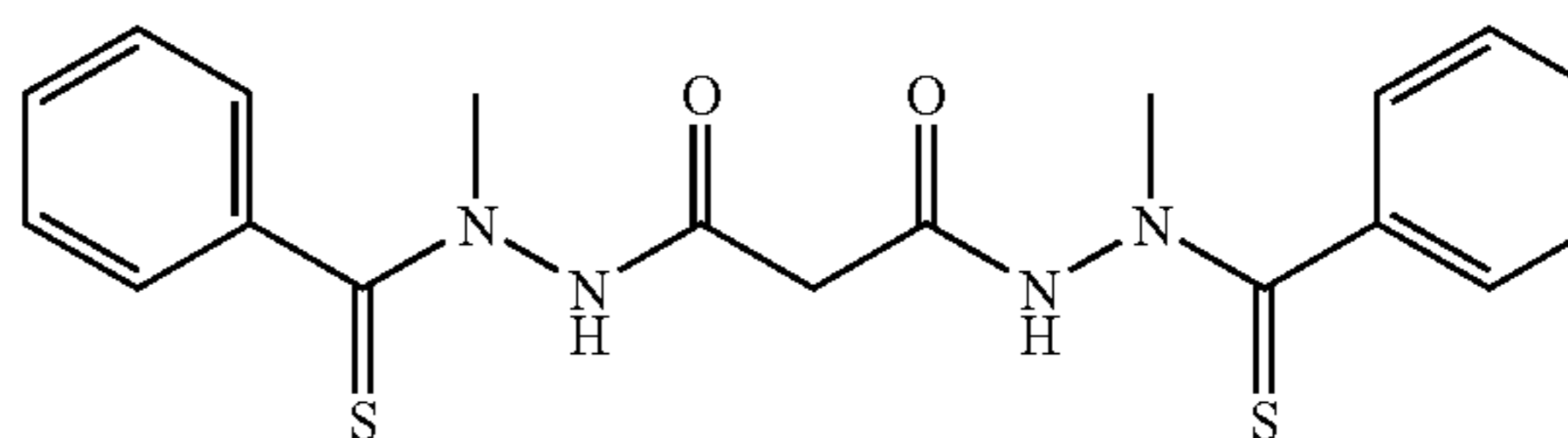
Compound (1)
