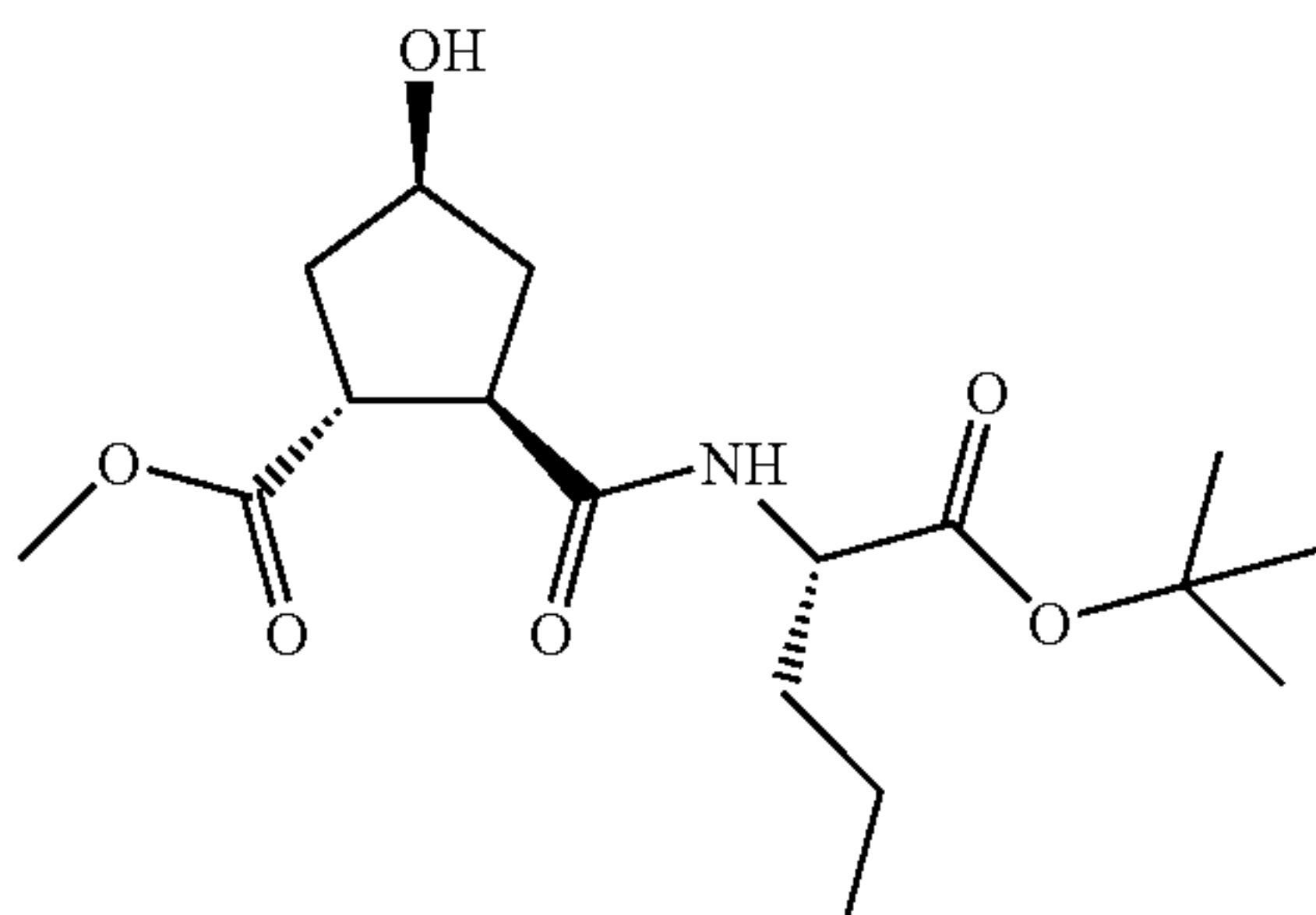
(1R,2R,4S)-2-((S)-1-tert-Butoxycarbonyl-butylcarbamoyl)-4-hydroxy-cyclopentanecarboxylic acid methyl ester (42)
