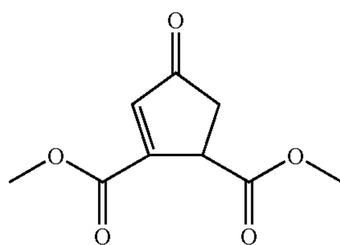
(Rac)-4-oxocyclopent-2-ene-1,2-dicarboxylic acid dimethyl ester (2)
