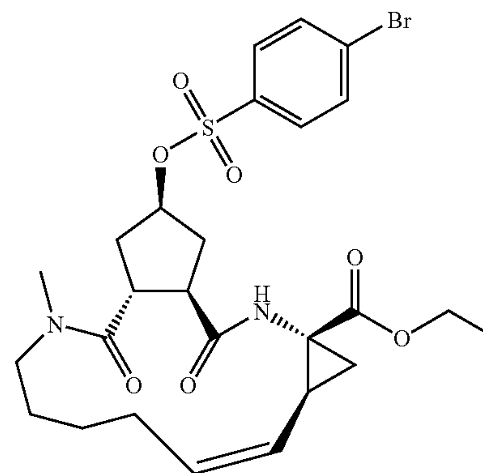
17-(4-Bromo-benzensulphonyloxy)-13-methyl-2,14-dioxo-3,13-diaza-tricyclo[13.3.0.0*4,6*]octadec-7-ene-4-carboxylic acid ethyl ester (108)
