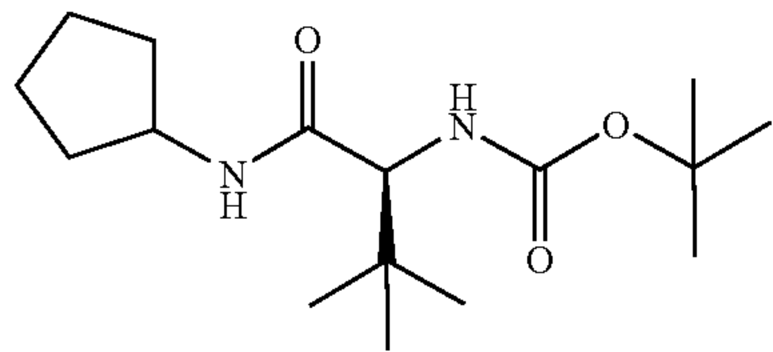
((S)-1-Cyclopentylcarbamoyl-2,2-dimethyl-propyl)-carbamic acid tert-butyl ester (51)
