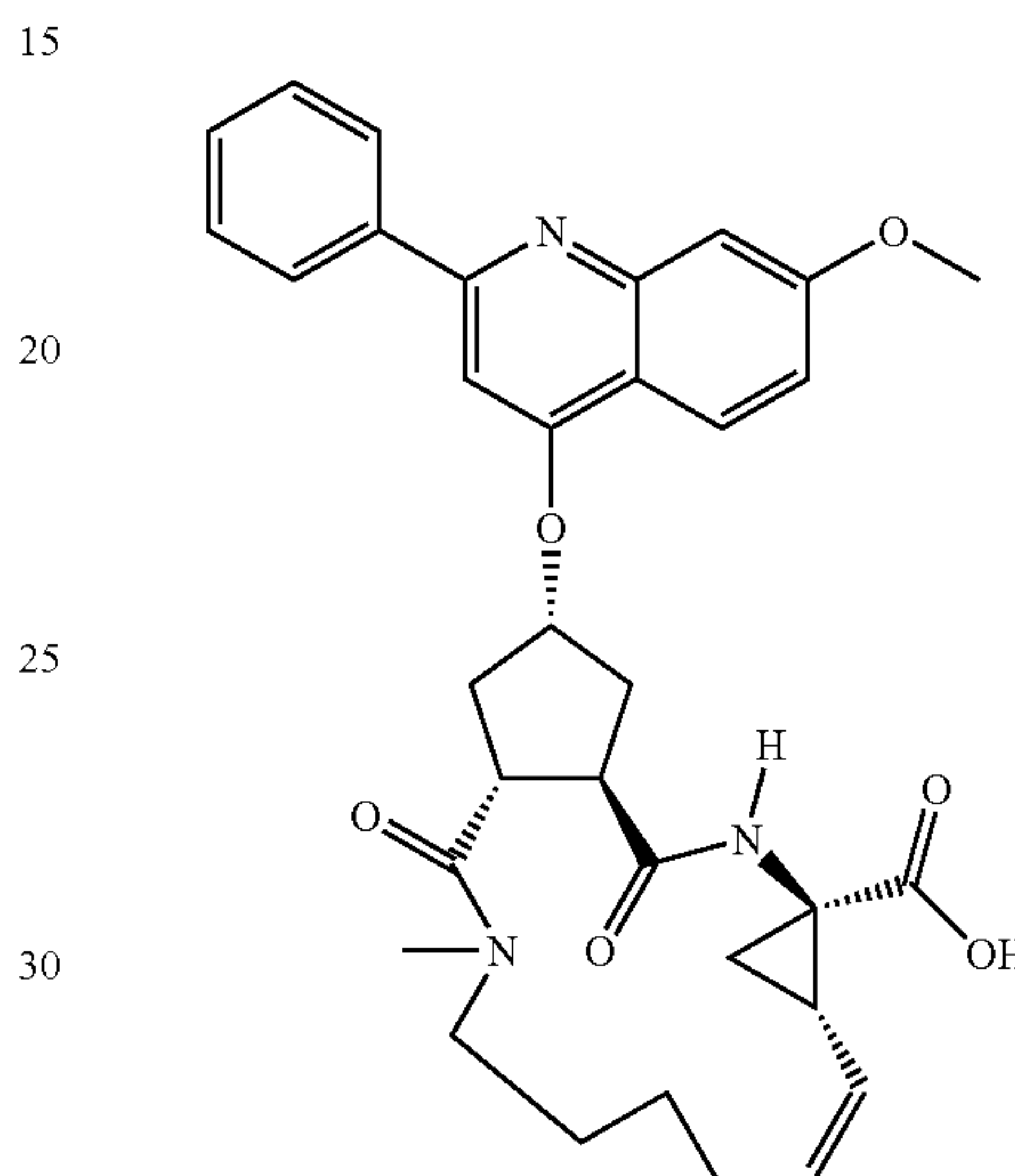
1-([2-(2-hex-5-enyl-1-methylcarbamoyl)-4-(7-methoxy-2-phenylquinolin-4-yloxy)cyclopentanecarbonyl]amino)-2-vinylcyclopropanecarboxylic acid ethyl ester (95)
