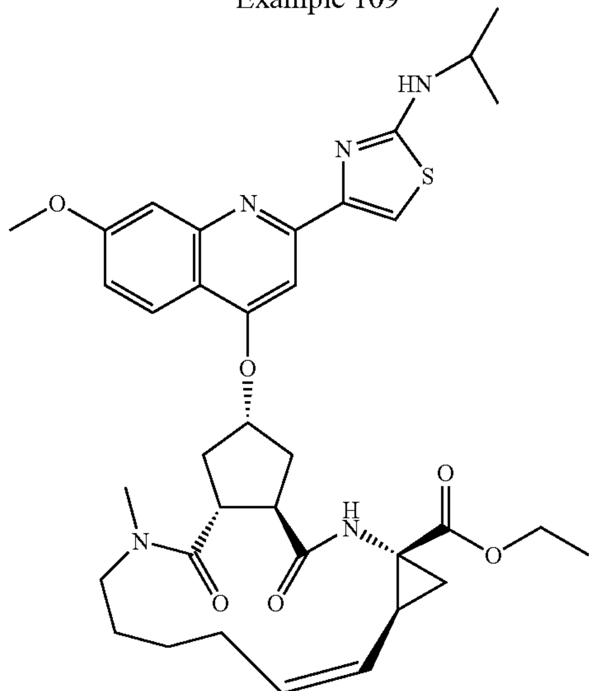
17-[2-(2-Isopropylamino-thiazol-4-yl)-7-methoxy-quinolin-4-yloxy]-13-methyl-2,14-dioxo-3,13-diazatricyclo[13.3.0.0*4,6*]octadec-7-ene-4-carboxylic acid ethyl ester (109)
