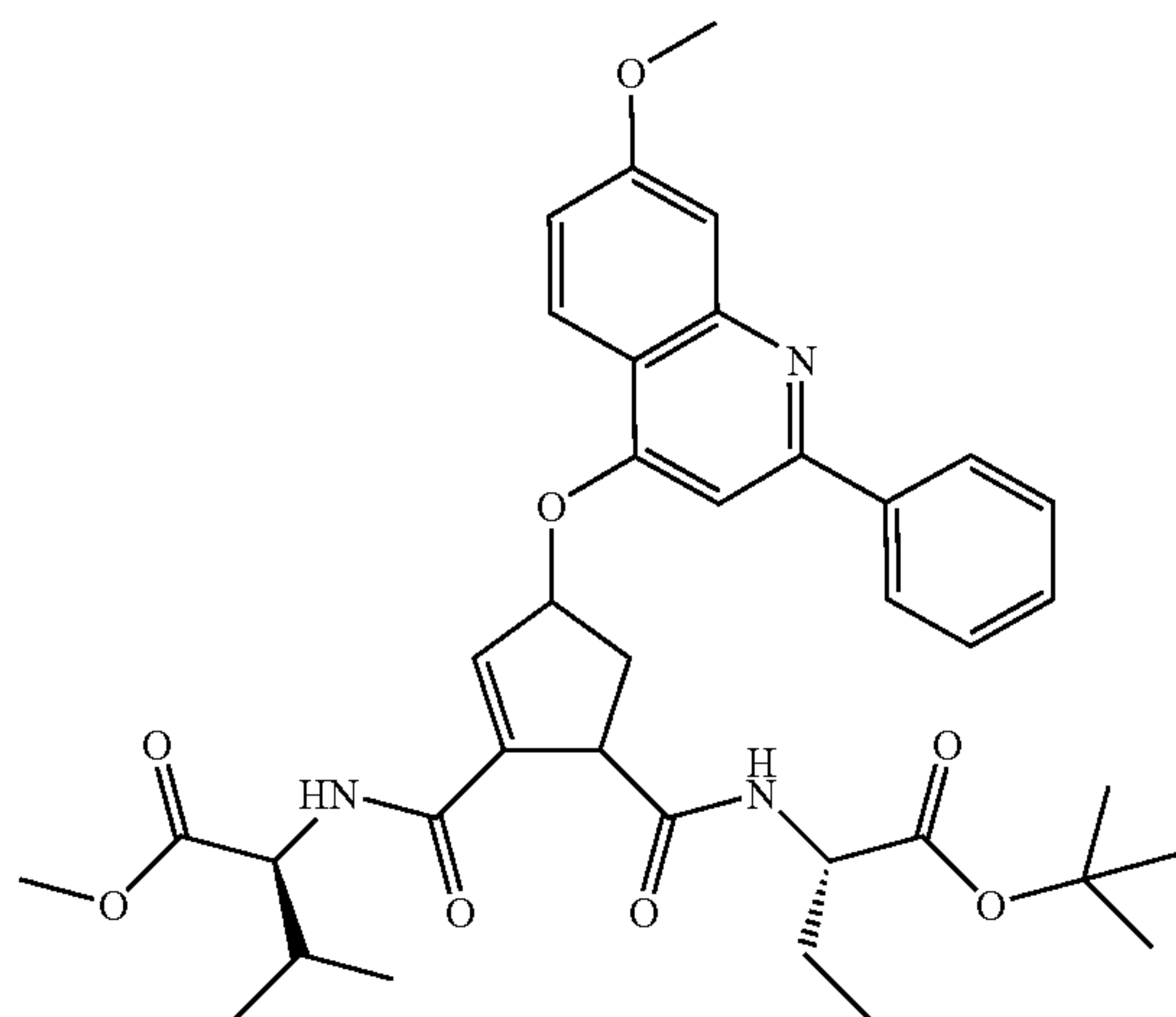
(S)-2-(((3R,5R) & (3S,5S))-5-((S)-1-tert-Butoxycarbonyl-propylcarbamoyl)-3-(7-methoxy-2-phenylquinolin-4-yloxy)-cyclopent-1-enecarbonyl)-amino}-3-methyl-butiric acid methyl ester (16)
