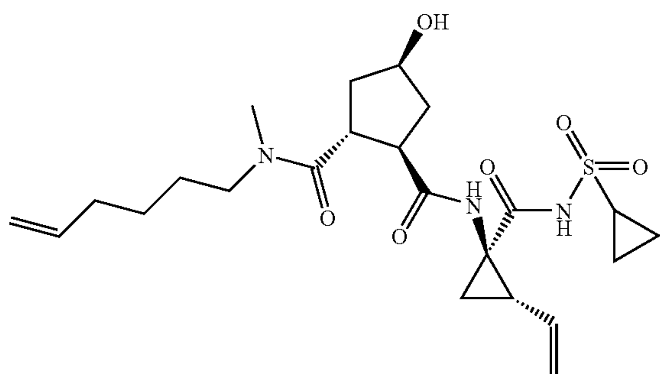
4-Hydroxycyclopentane-1,2-dicarboxylic acid 1-[(1-cyclopropanesulphonylamino-carbonyl-2-vinylcyclopropyl)-amide]2-(hex-5-enyl-methylamide) (102)
