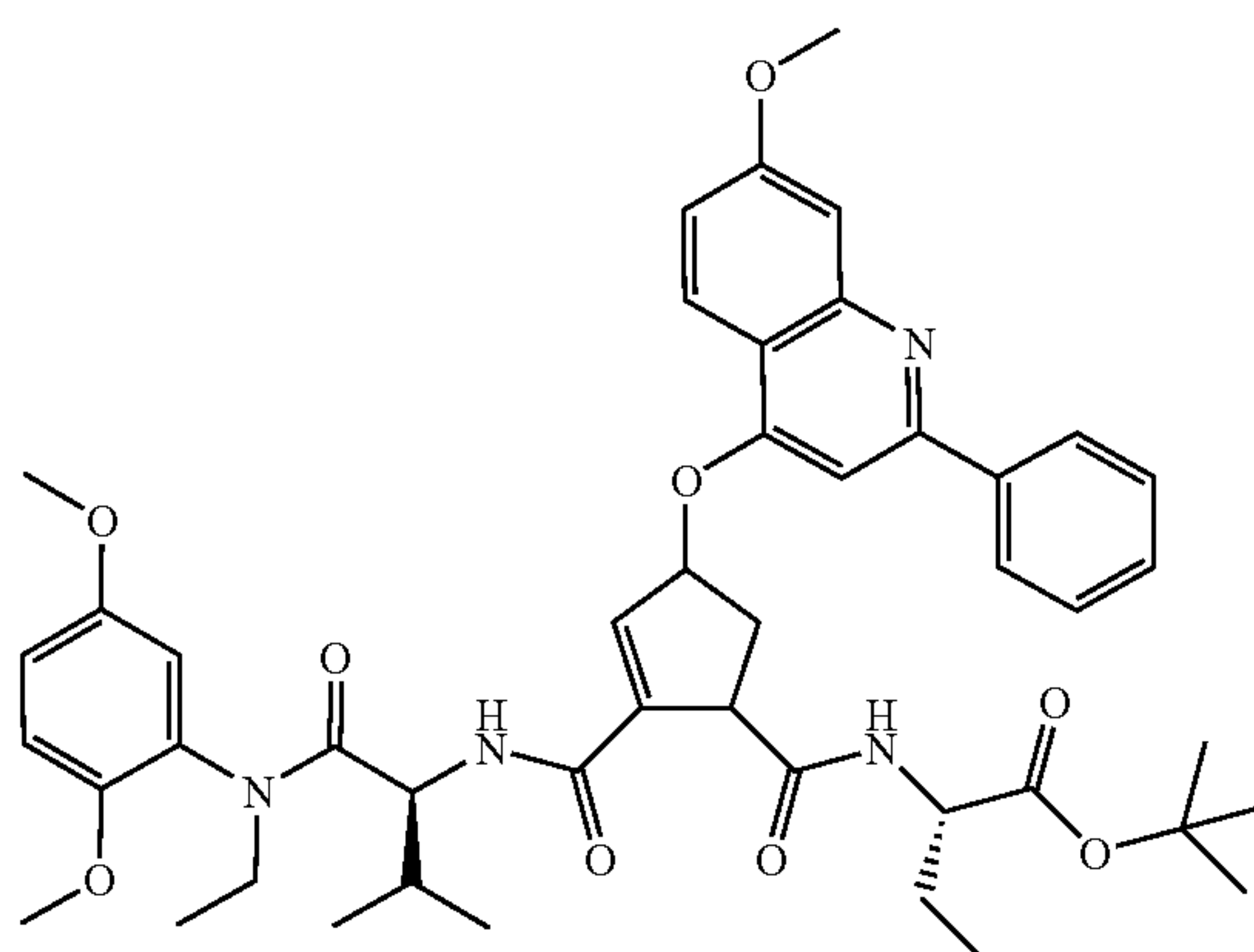
(S)-2-(((1R,4R) & (1S,4S))-2-((S)-1-[(2,5-Dimethoxy-phenyl)-ethyl-carbamoyl]-2-methyl-propylcarbamoyl)-4-(7-methoxy-2-phenyl-quinolin-4-yloxy)-cyclopent-2-enecarbonyl)-amino}-butyric acid tert-butyl ester (17)
