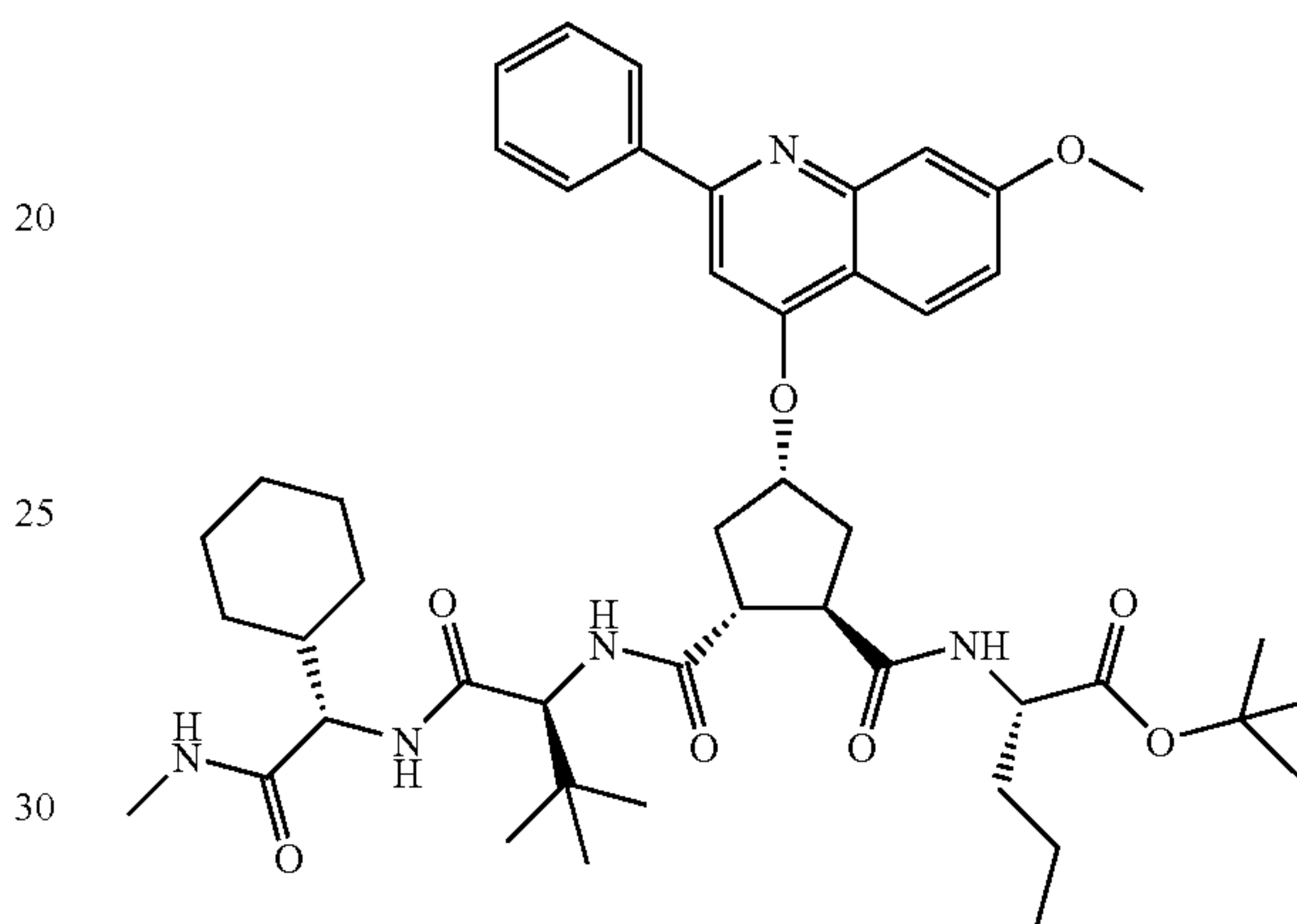
(S)-2-[[[(1R,2R,4S)-2-((S)-1-tert-Butoxycarbonyl-butylcarbamoyl)-4-hydroxy-cyclopentanecarboxylic acid methyl ester]-2,2-dimethylpropylcarbamoyl]-4-(7-methoxy-2-phenyl-quinolin-4-yloxy)-cyclopentanecarboxylic acid tert-butyl ester (44)
