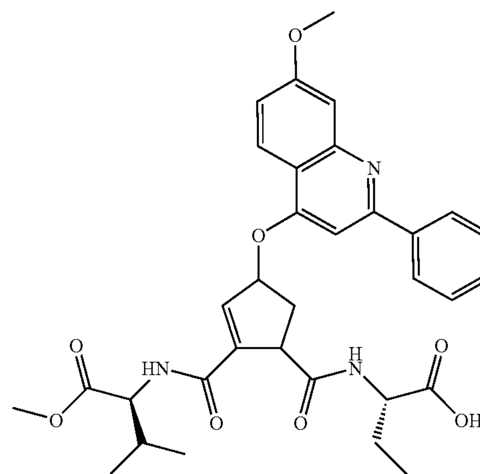
(S)-2-[[[(3R,5R) & (3S,5S)]-5-[(S)-1-Carboxy-propylcarbamoyl]-3-(7-methoxy-2-phenyl-quinolin-4-yloxy)-cyclopent-1-enecarbonyl]-amino]-3-methylbutyric acid methyl ester (25)
