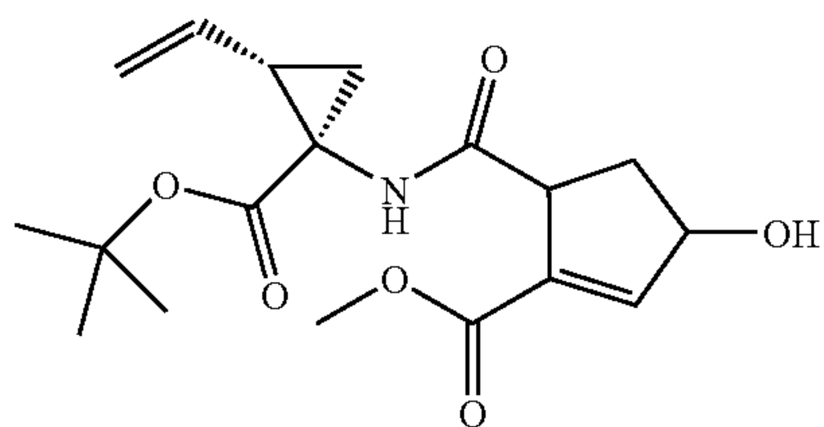
((3S,5R) & (3R,5S))-5-((1R,2S)-1-tert-Butoxycarbonyl-2-vinyl-cyclopropylcarbamoyl)-3-hydroxy-cyclopent-1-enecarboxylic acid methyl ester (7)
