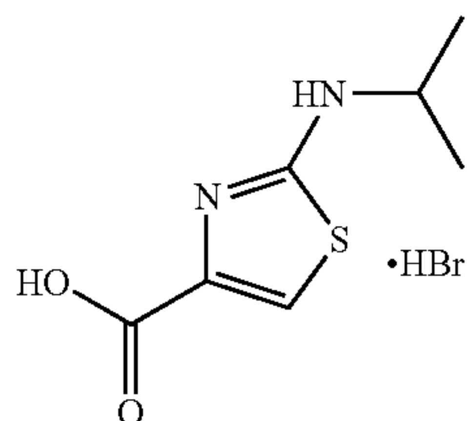
2-(Isopropylamino)-1,3-thiazole-4-carboxylic acid hydrobromide (69)
