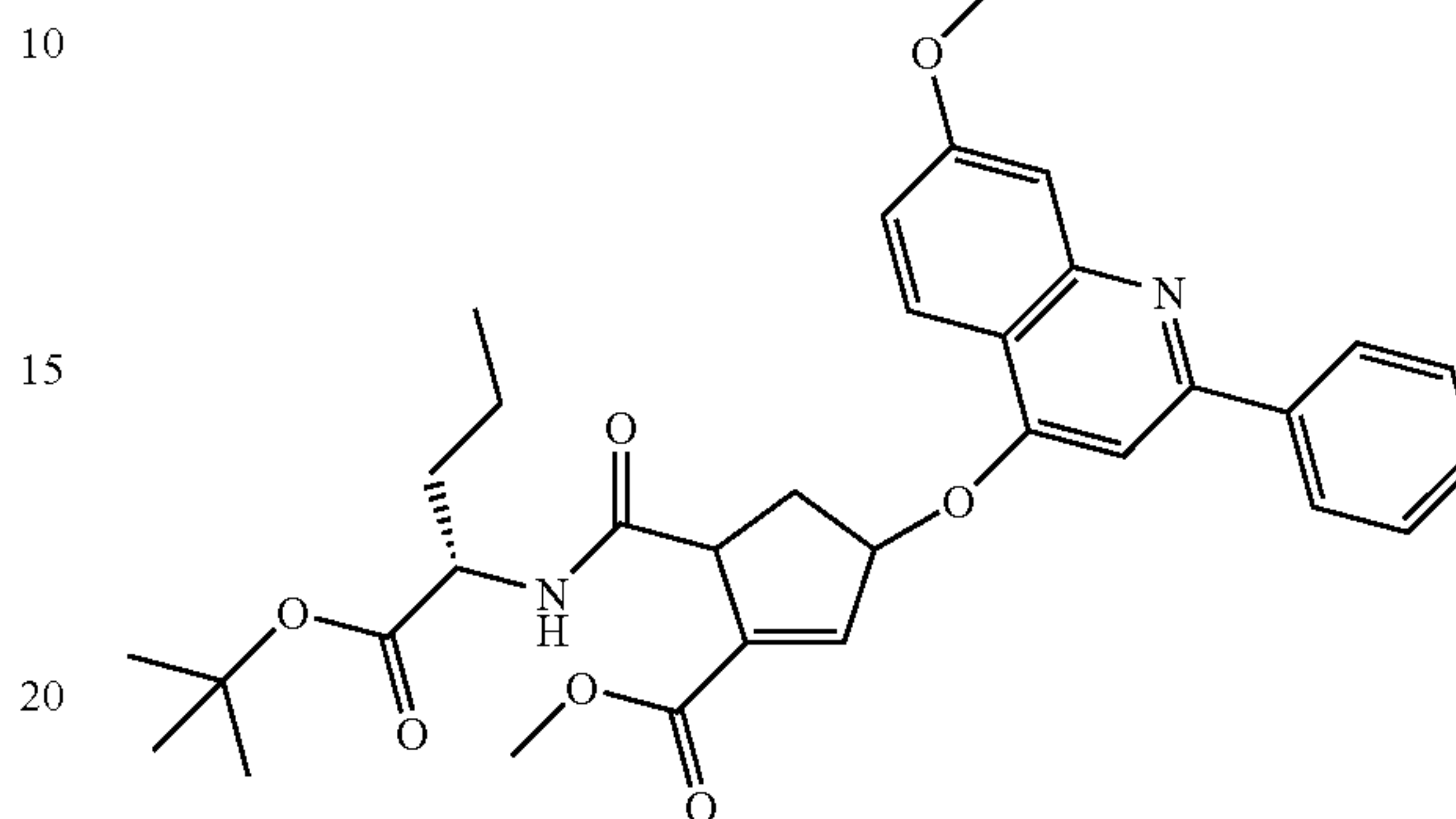
((3R,5R) & (3S,5S))-5-((S)-1-tert-Butoxycarbonyl-butylcarbamoyl)-3-(7-methoxy-2-phenyl-quinolin-4-yloxy)-cyclopent-1-enecarboxylic acid methyl ester (8)
