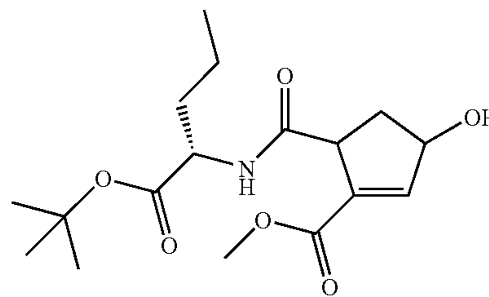
((3S,5R) & (3R,5S))-5-((S)-1-tert-Butoxycarbonyl-butylcarbamoyl)-3-hydroxy-cyclopent-1-enecarboxylic acid methyl (5)
