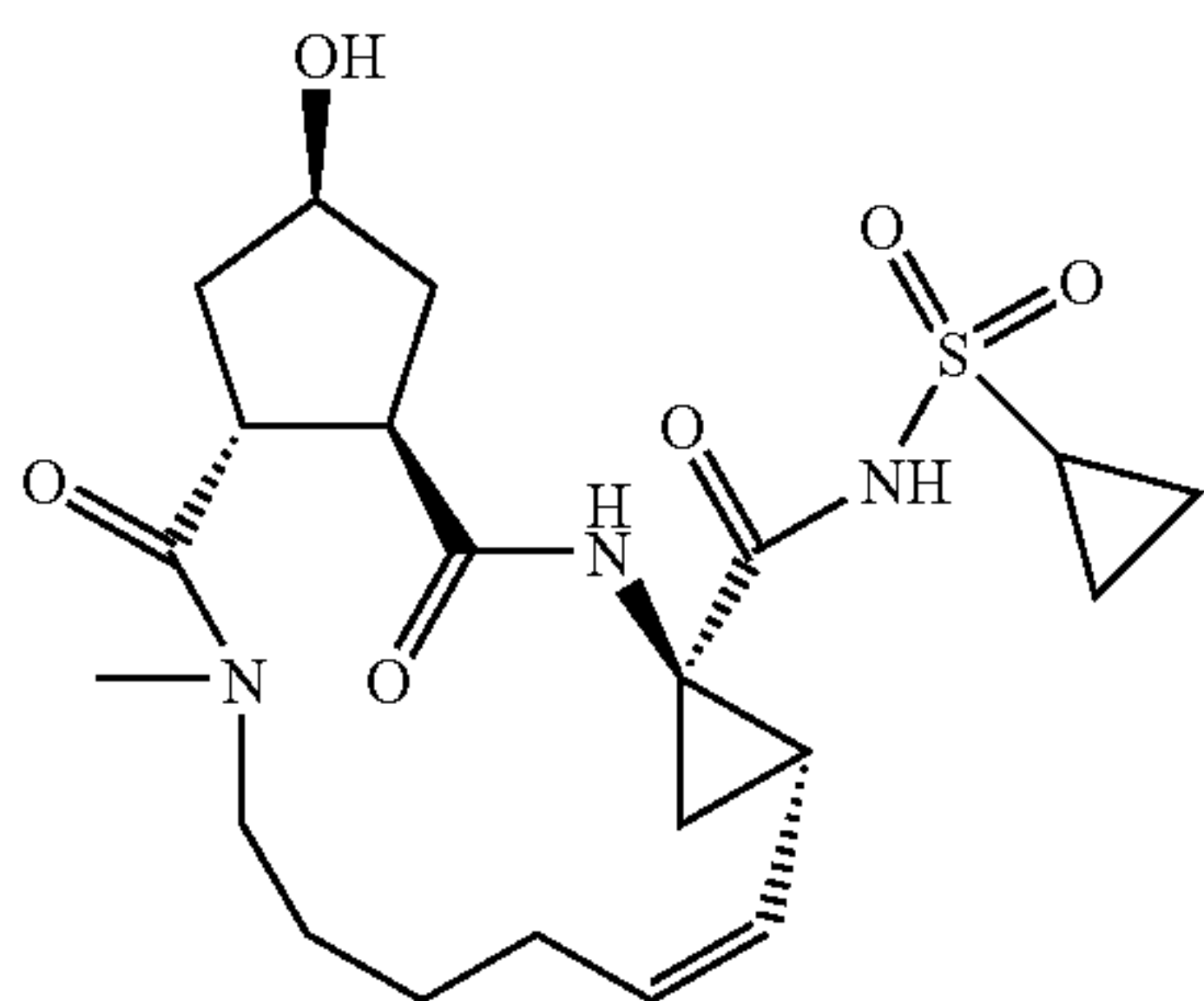
Cyclopropanesulphonic acid (17-hydroxy-13-methyl-2,14-dioxo-3,13-diazatricyclo[13.3.0.0*4,6*]octadec-7-ene-4-carbonyl)-amide (103)
