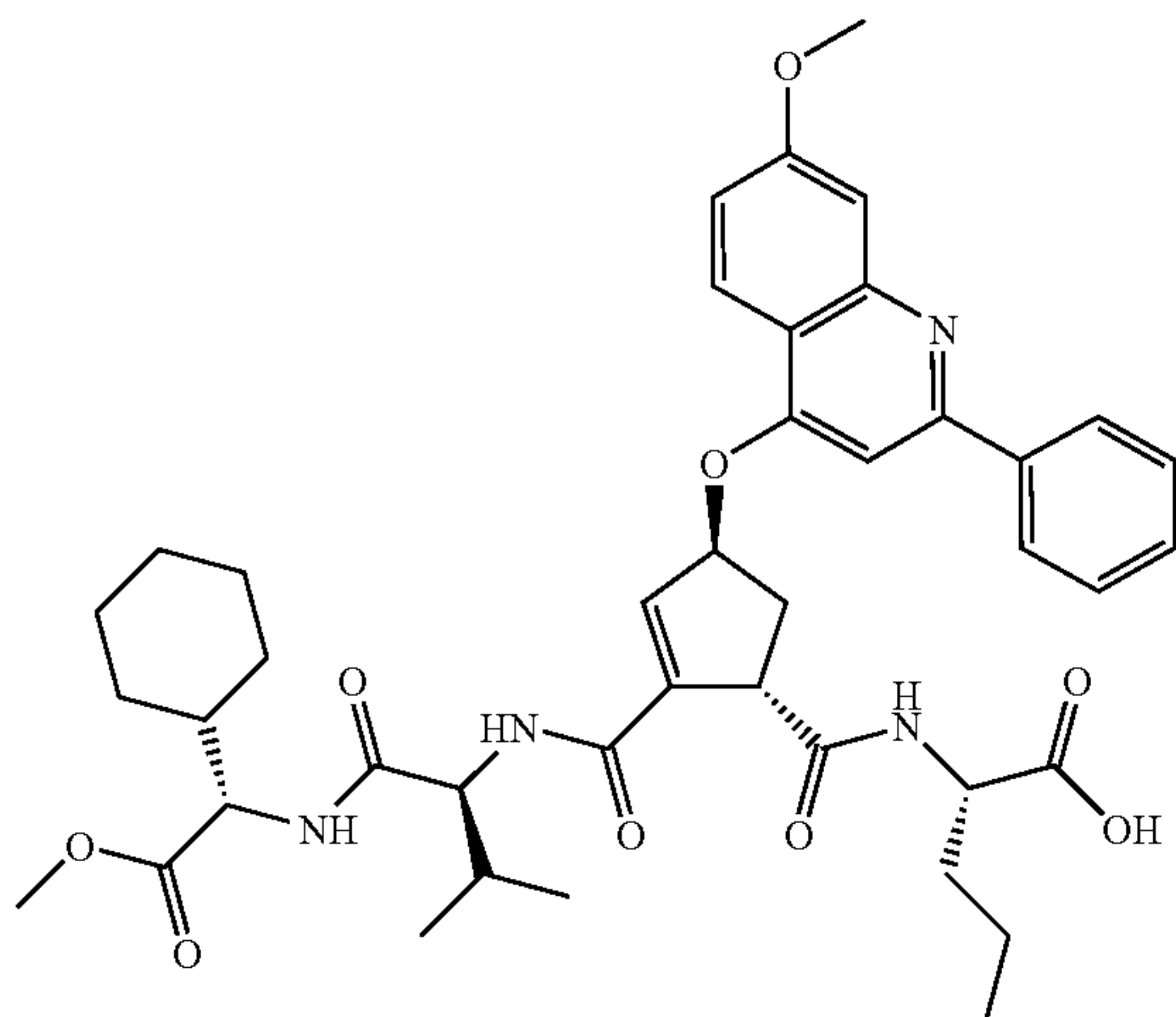
(S)-2-[[[(1S,4S)-2-[(S)-1-[[[(S)-Cyclohexyl-methoxycarbonyl-methyl]-carbamoyl]-2-methyl-propylcarbamoyl]-4-(7-methoxy-2-phenyl-quinolin-4-yloxy)-cyclopent-2-enecarbonyl]-amino]-pentanoic acid tert-butyl ester (29)
