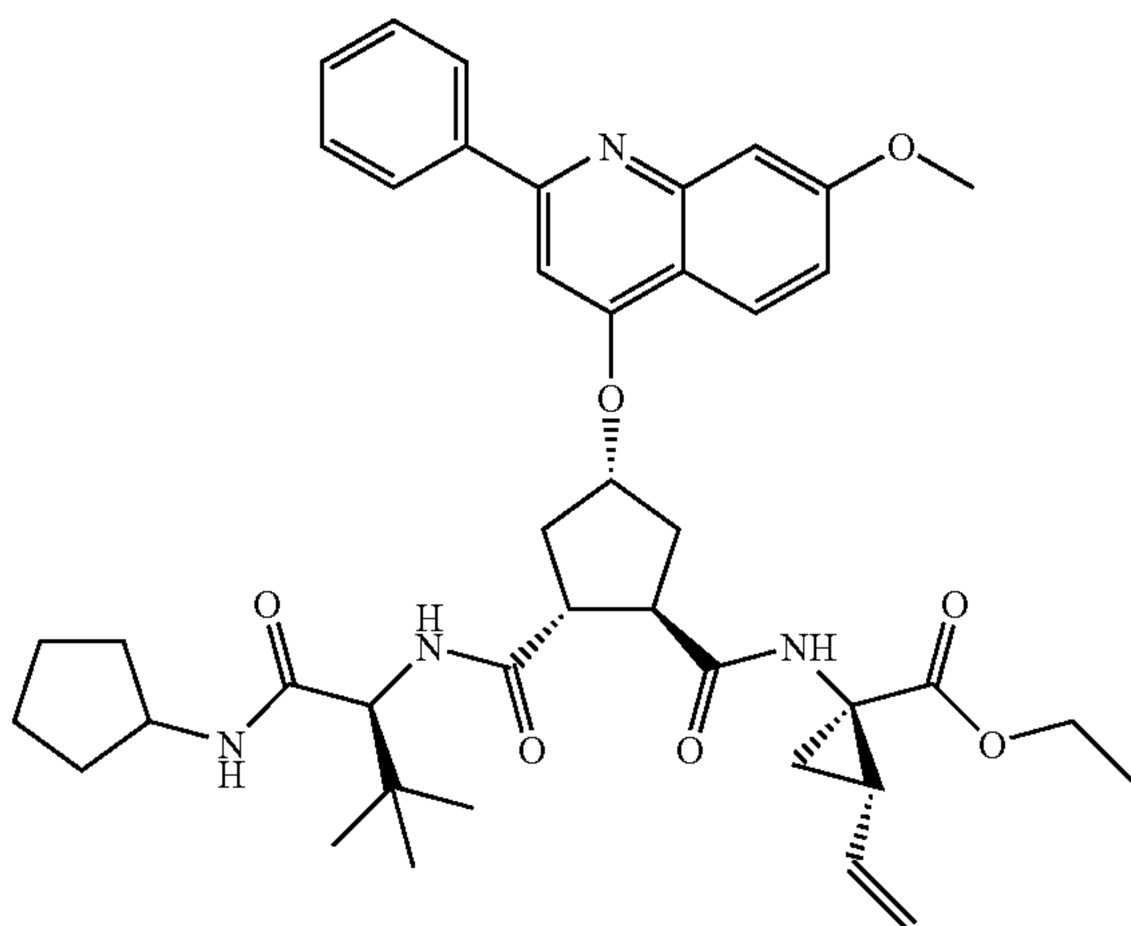
(1R,2S)-1-[[[(1R,2R,4S)-2-((S)-1-Cyclopentylcarbamoyl-2,2-dimethyl-propylcarbamoyl)-4-(7-methoxy-2-phenyl-quinolin-4-yloxy)-cyclopentanecarbonyl]-amino]-2-vinyl-cyclopropanecarboxylic acid ethyl ester (52)
