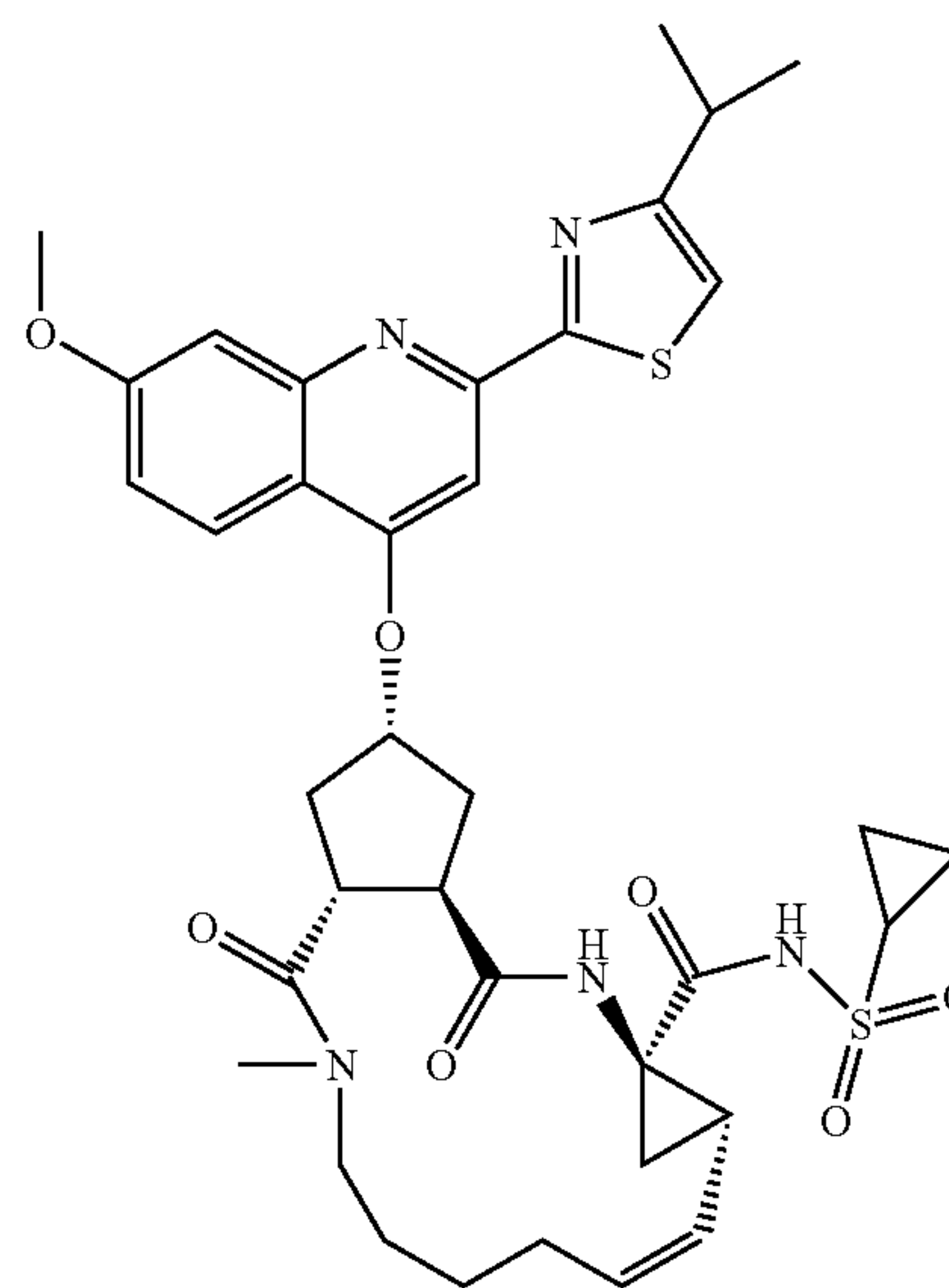
Cyclopropanesulphonic acid {17-[2-(4-isopropylthiazol-2-yl)-7-methoxyquinolin-4-yloxy]-13-methyl-2,14-dioxo-3,13-diazatricyclo[13.3.0.0*4,6*]octadec-7-ene-4-carbonyl)-amide (104)
