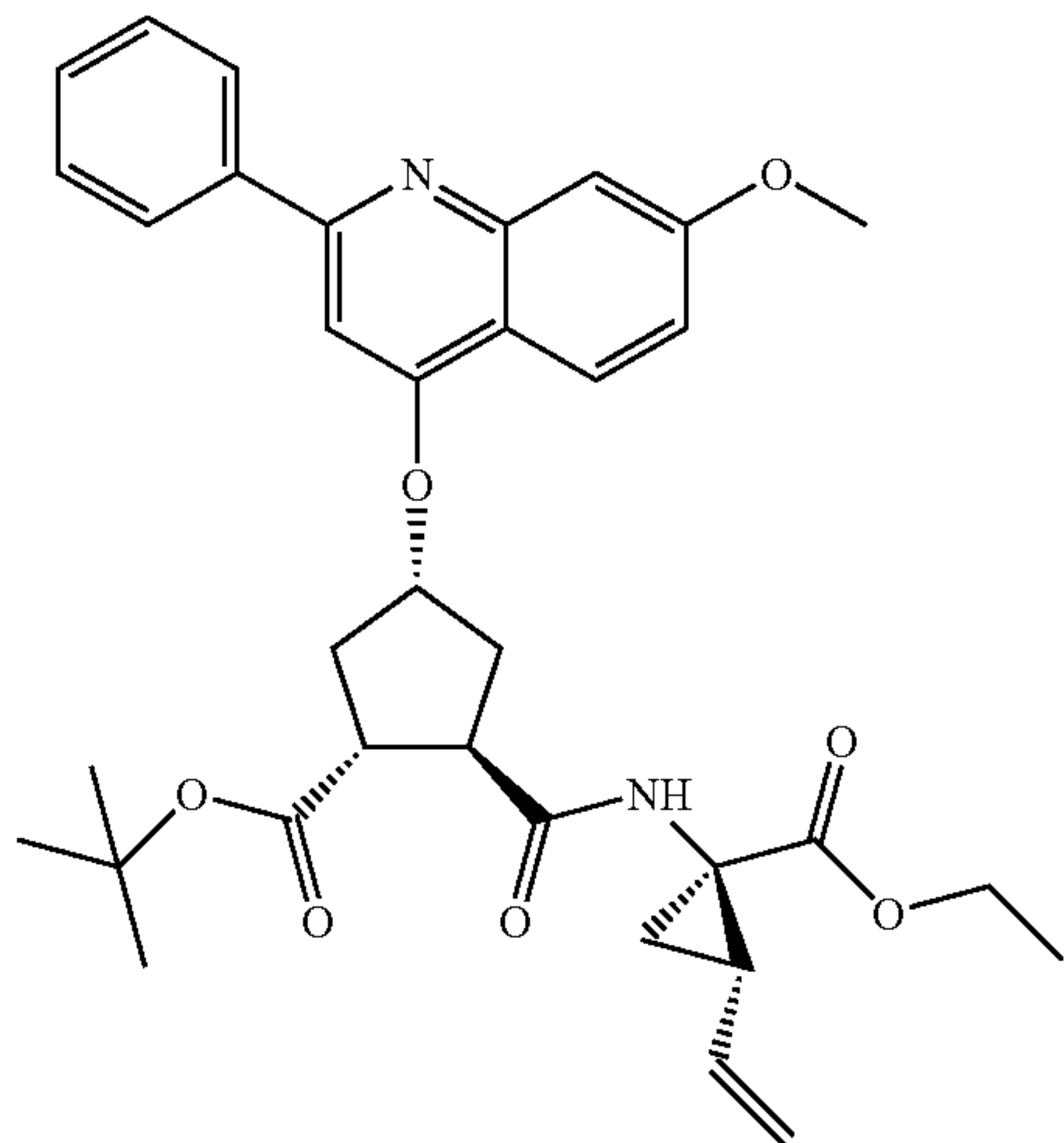
(1R,2R,4R)-2-((1R,2S)-1-Ethoxycarbonyl-2-vinyl-cyclopropylcarbamoyl)-4-(7-methoxy-2-phenyl-quinolin-4-yloxy)-cyclopentanecarboxylic acid tert-butyl ester (35)
