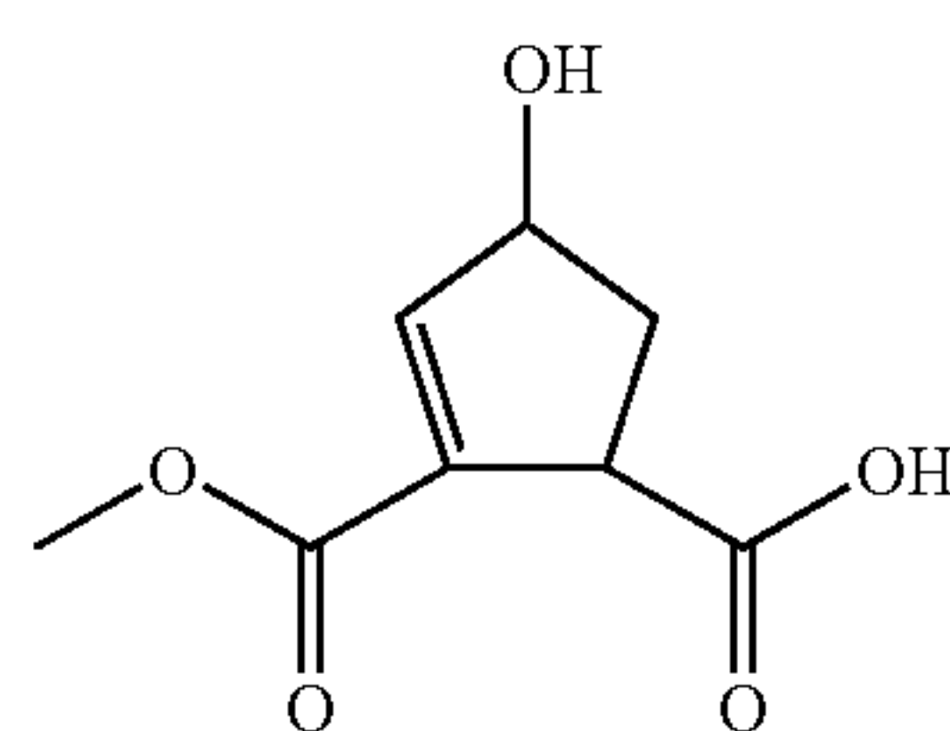
(1S,4R) & (1R,4S)-4-hydroxy-cyclopent-2-ene-1,2-dicarboxylic acid 2-methyl ester (4)
