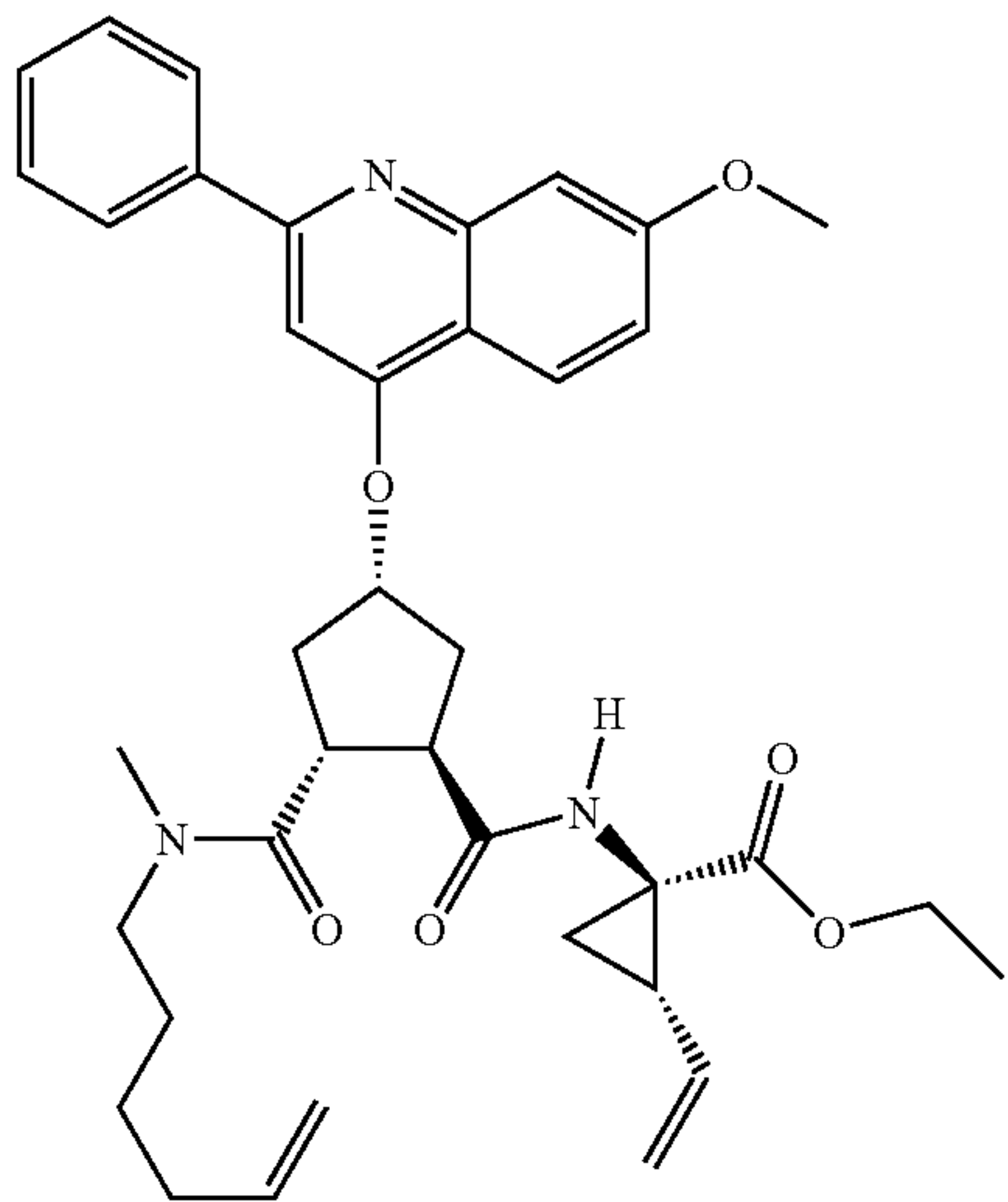
1-([2-(2-hex-5-enyl-1-methylcarbamoyl)-4-(7-methoxy-2-phenylquinolin-4-yloxy)cyclopentanecarbonyl]amino)-2-vinylcyclopropanecarboxylic acid ethyl ester (95)
