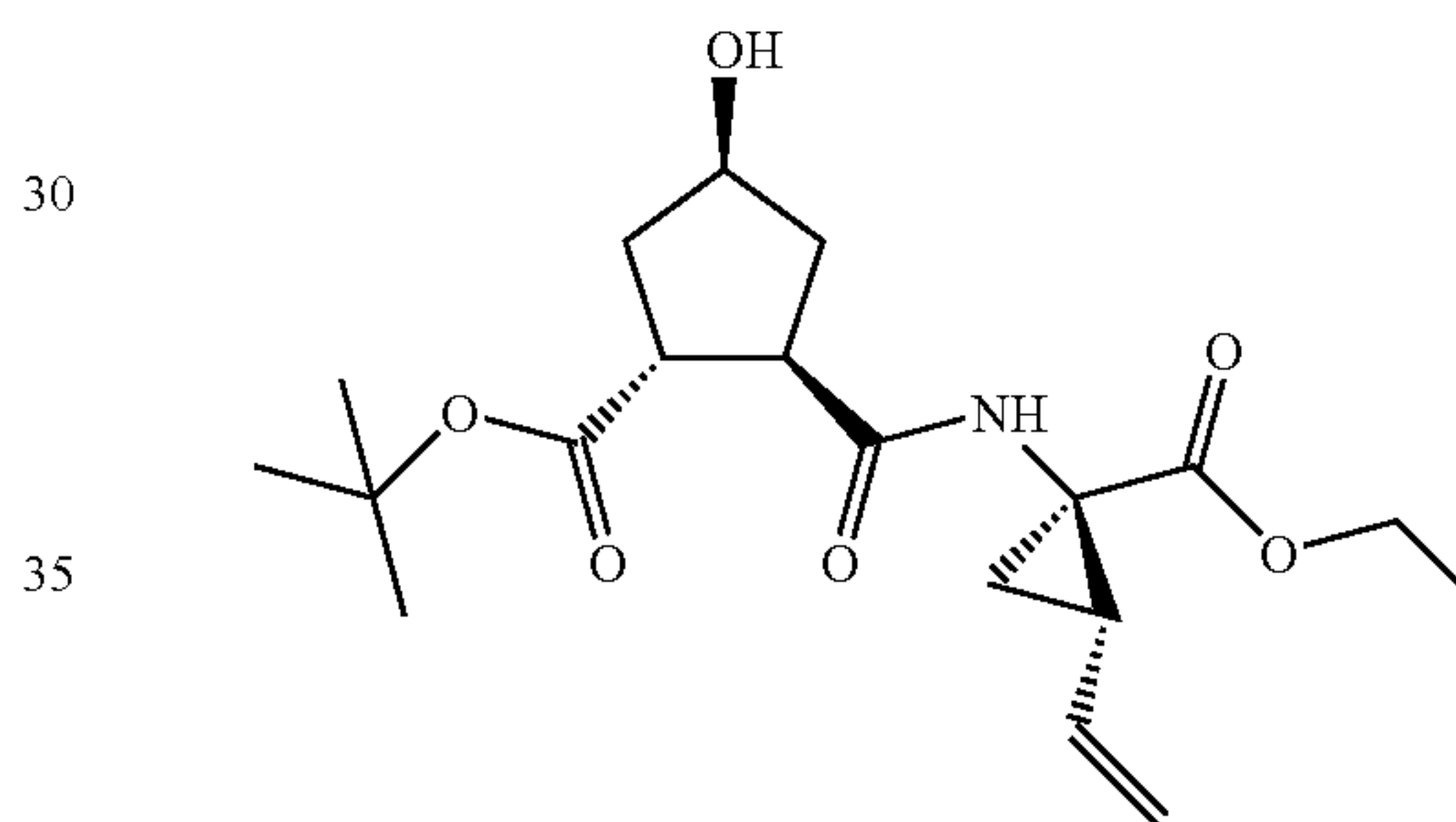
(1R,2R,4S)-2-((1R,2S)-1-Ethoxycarbonyl-2-vinylcyclopropylcarbamoyl)-4-hydroxy-cyclopentanecarboxylic acid tert-butyl ester (34)
