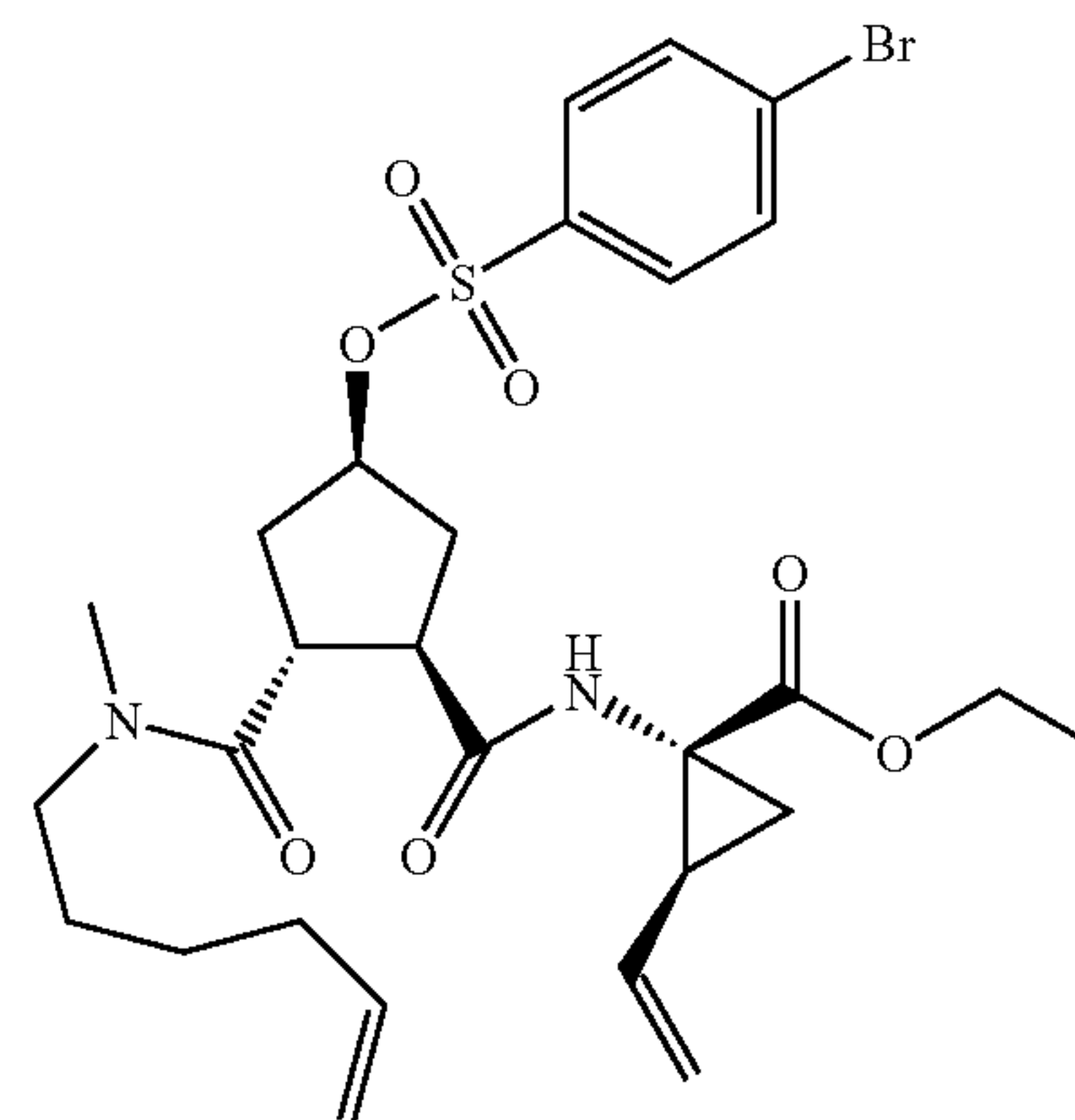
1-{[4-(4-Bromo-benzensulphonyloxy-2-(hex-5-enyl-methyl-carbamoyl)-cyclopentanecarbonyl]-amino}-2-vinyl-cyclopropanecarboxylic acid ethyl ester (107)
