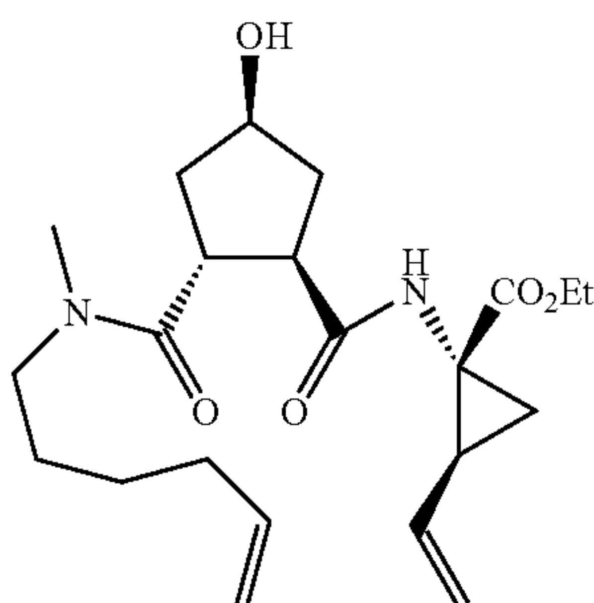
1-{[2-(Hex-5-enyl-methyl-carbamoyl)-4-hydroxy-cyclopentanecarbonyl]-amino}-2-vinyl-cyclopropanecarboxylic acid ethyl ester (106)
