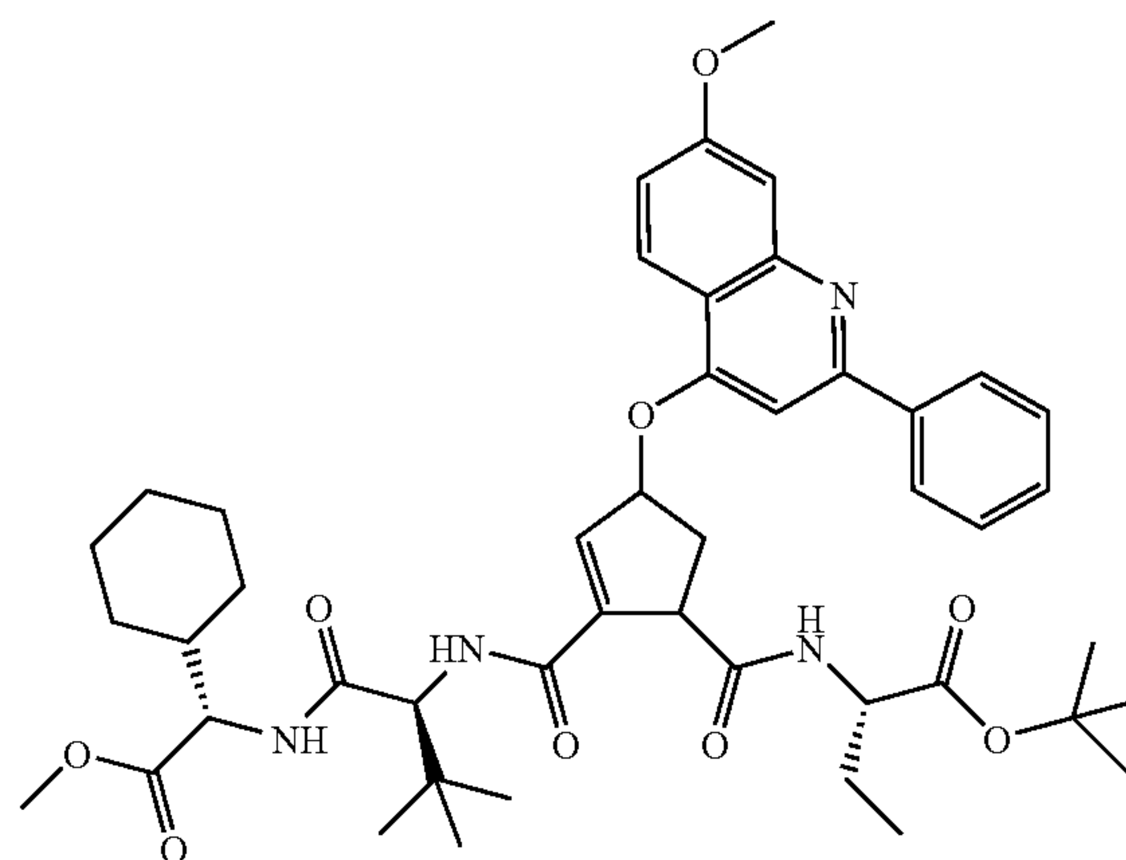
(S)-2-(((1R,4R) & (1S,4S))-2-((S)-1-[(S)-Cyclohexyl-methoxycarbonyl-methyl]-carbamoyl]-2,2-dimethyl-propylcarbamoyl)-4-(7-methoxy-2-phenyl-quinolin-4-yloxy)-cyclopent-2-enecarbonyl)-amino}-butyric acid tert-butyl ester (18)
