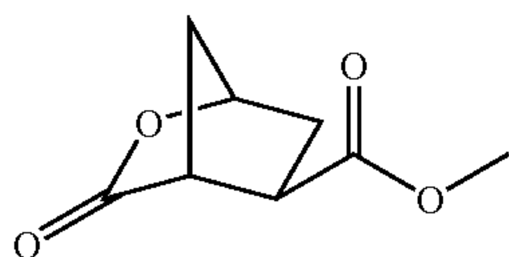
3-Oxo-2-oxa-bicyclo[2.2.1]heptane-5-carboxylic acid methyl ester (41)
