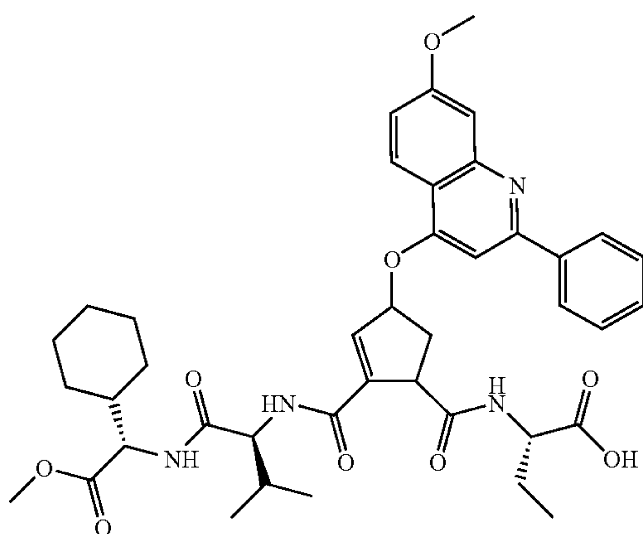
(S)-2-[[[(1R,4R) & (1S,4S)]-2-[(S)-1-[(S)-Carboxy-cyclohexyl-methyl]-carbamoyl]-2-methyl-propylcarbamoyl]-4-(7-methoxy-2-phenyl-quinolin-4-yloxy)-cyclopent-2-enecarbonyl]-amino]-butyric acid (24)
