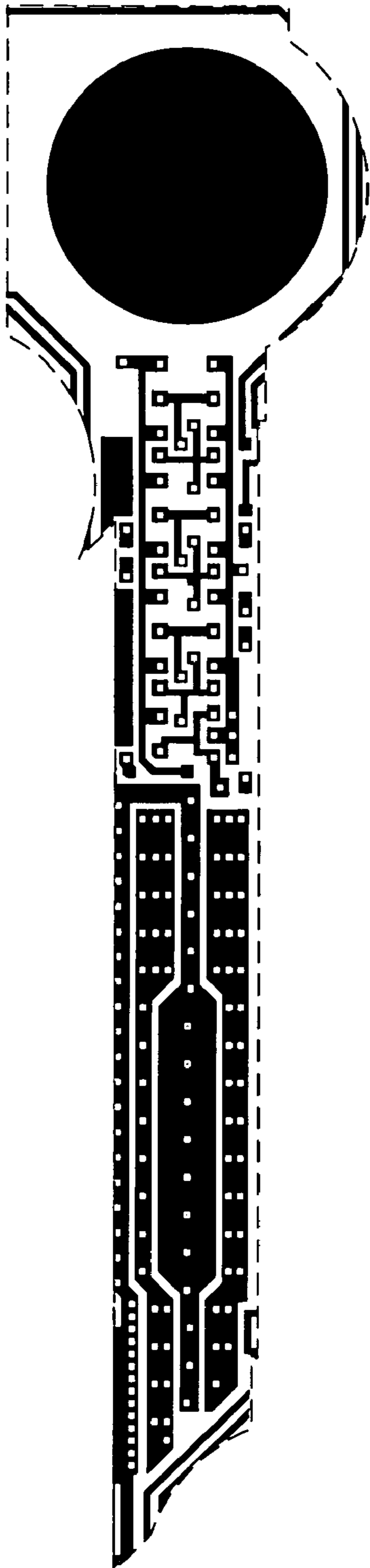
Metal 1 mask
