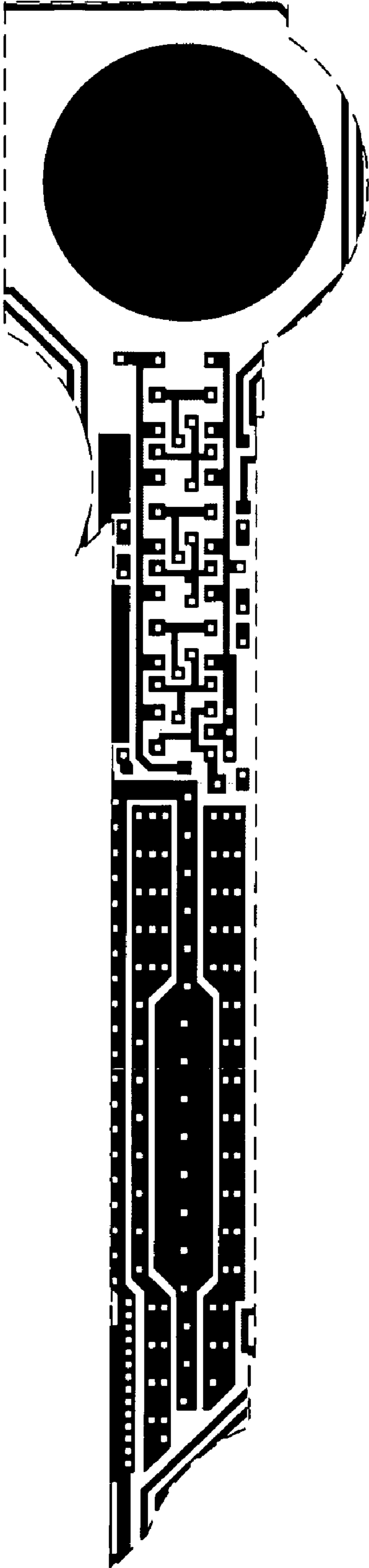
Metal 1 mask
