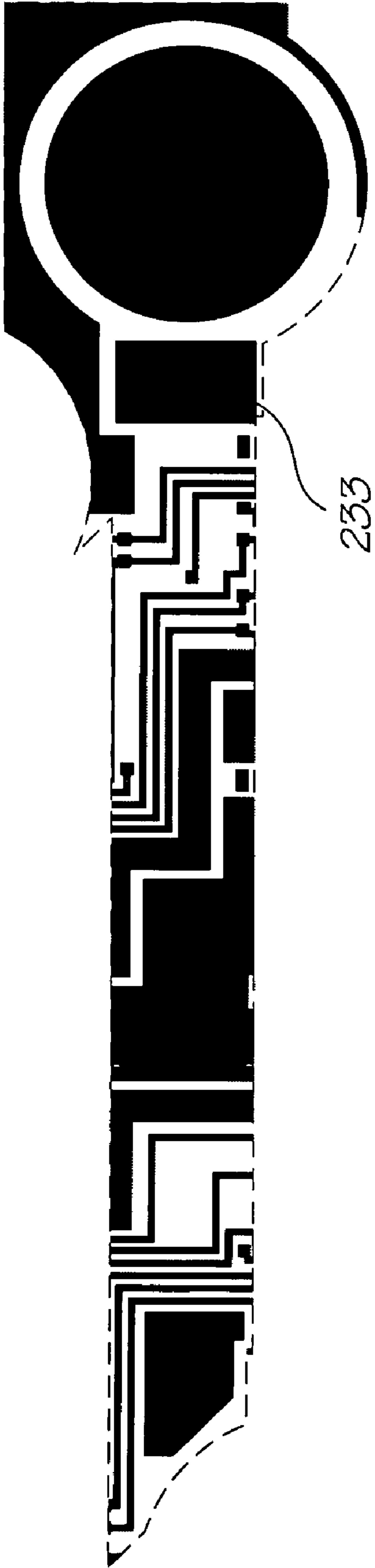
Metal 2 mask
