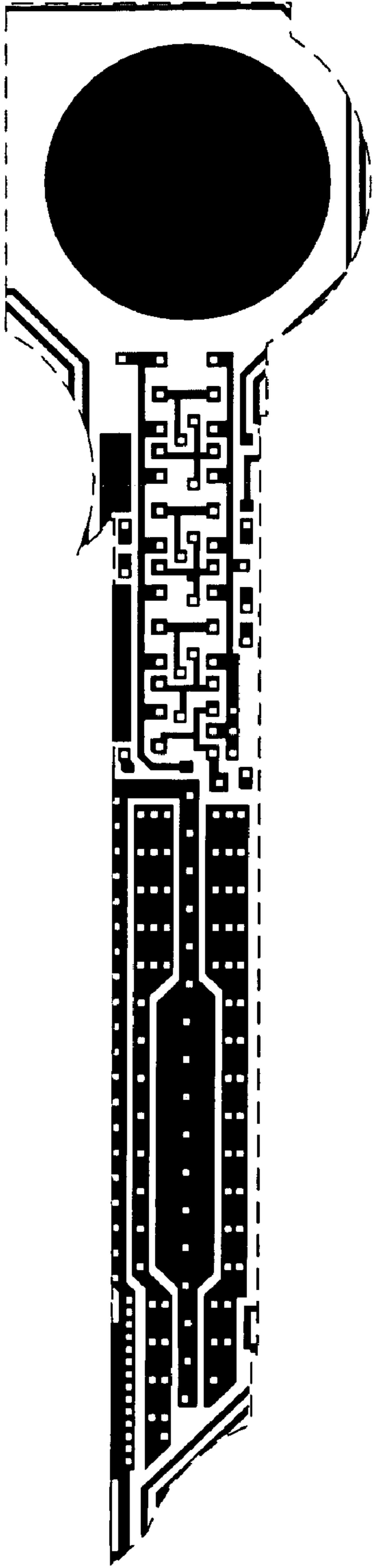
Metal 1 mask
