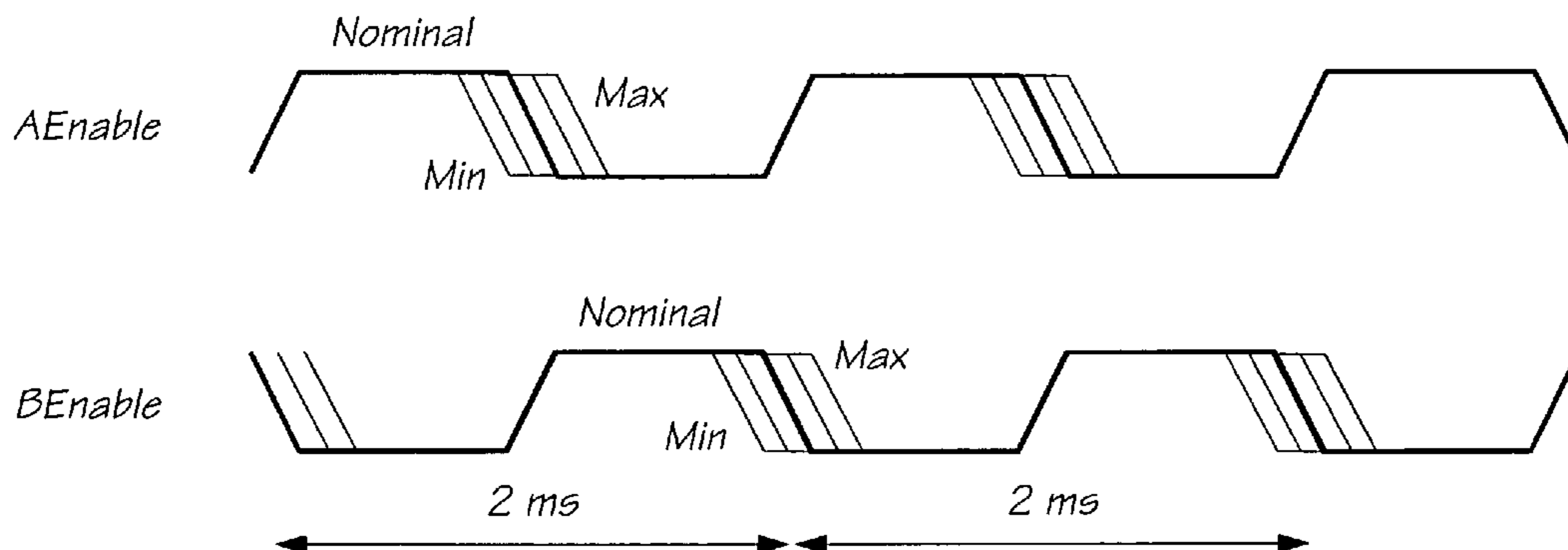
AEnable and BEnable during a Typical Print Cycle
