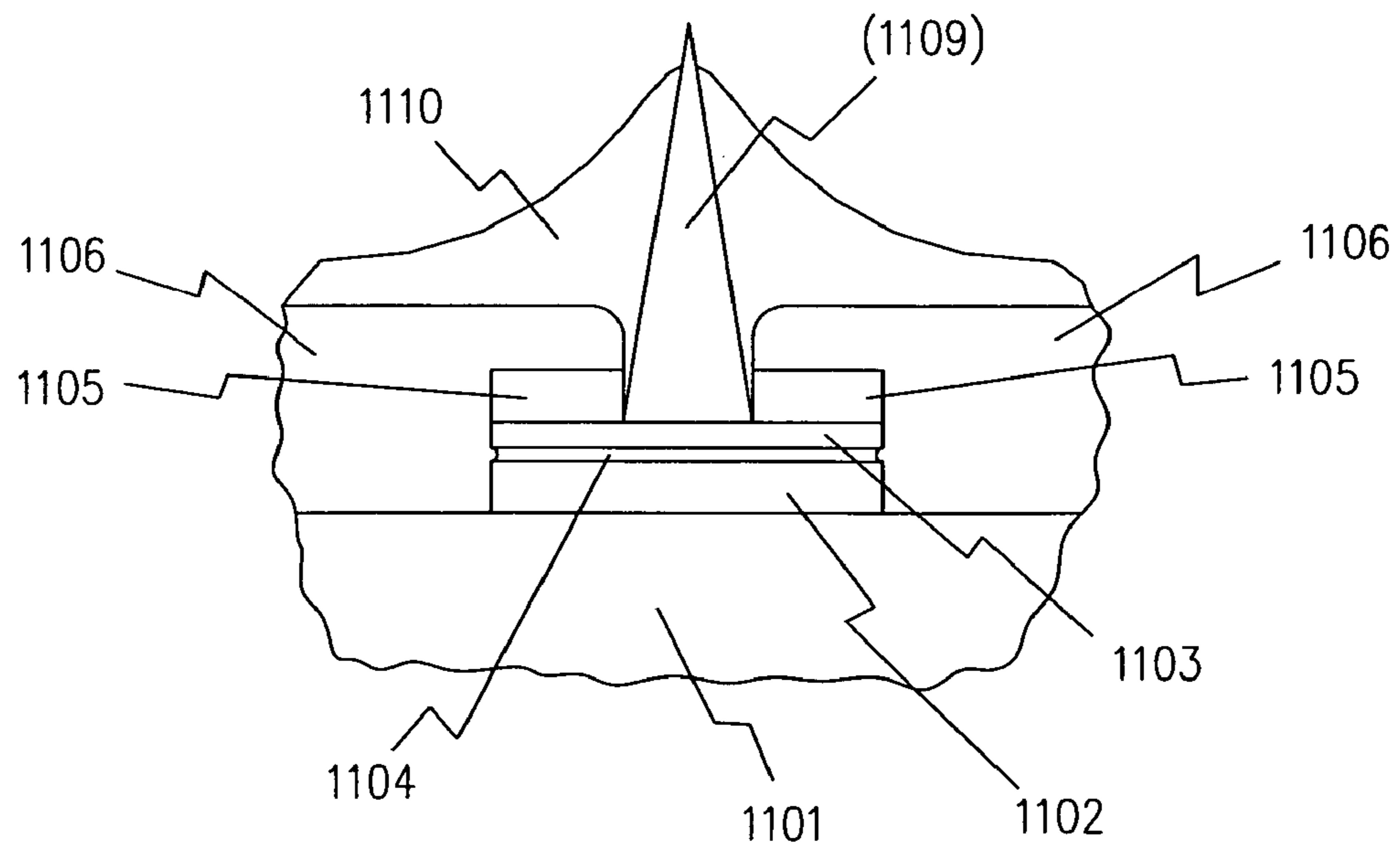
FIGURE 11b ELECTRODES
