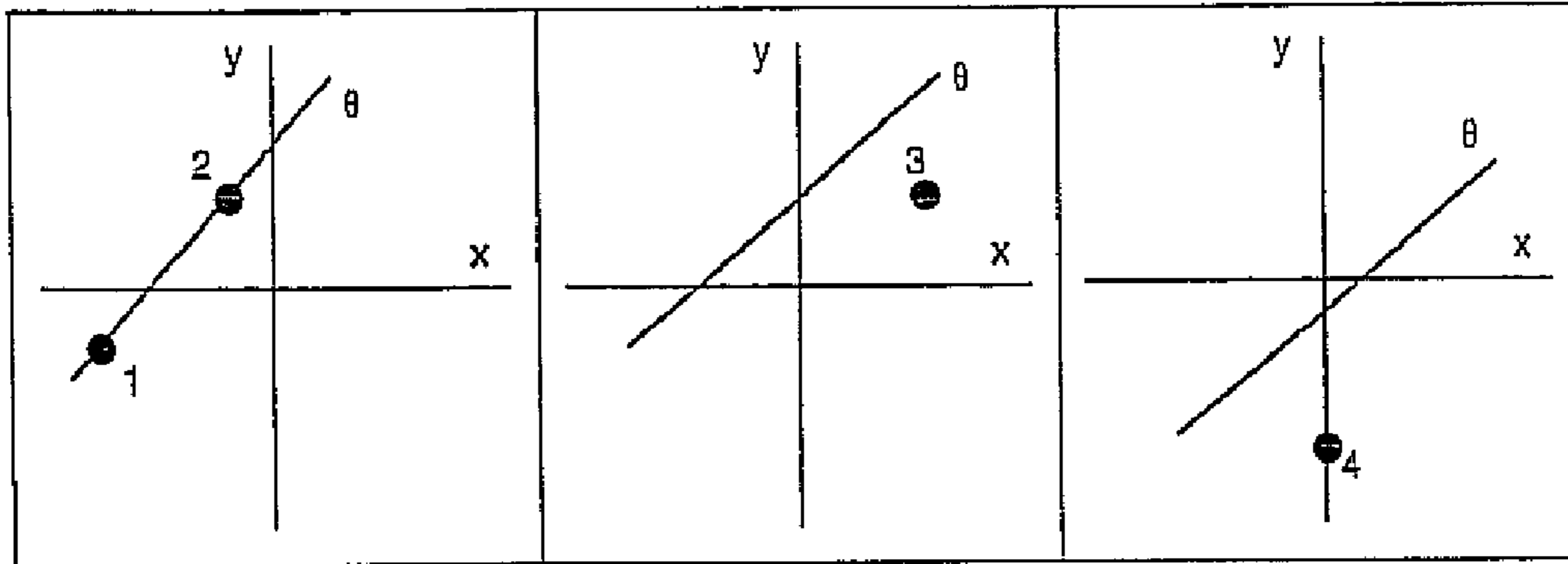
Figure 18: The Recursive Linear Least Squares Method for Updating q with Each Additional (x_i, y_i) Data Point.
