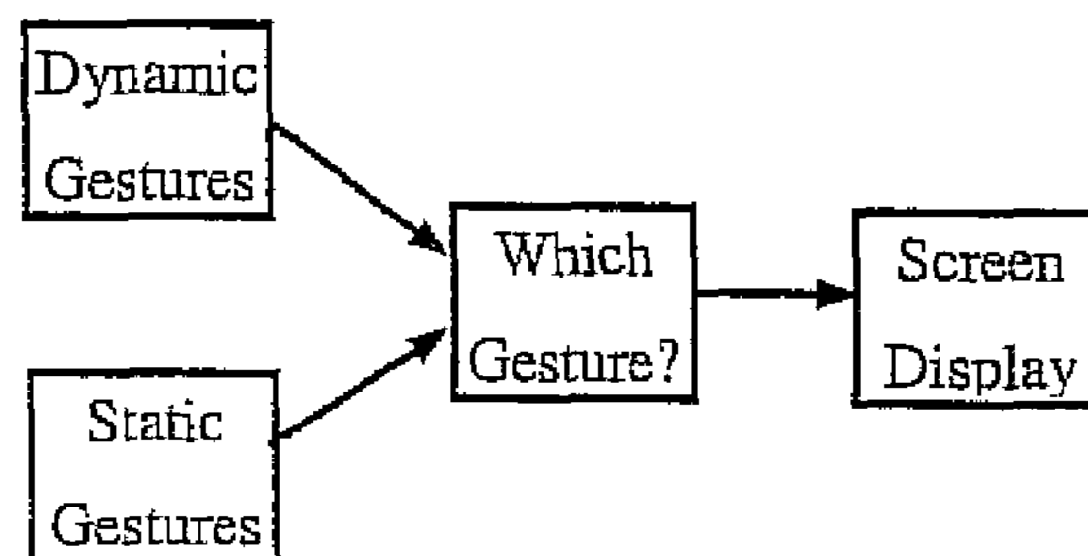
Figure 31: Identification Module.
