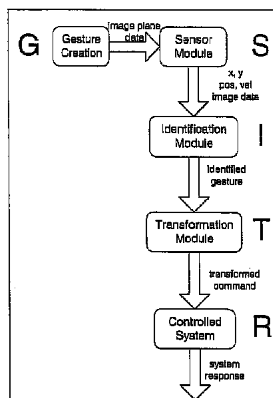
Signal Flow Diagram of the Gesture Recognition System.
