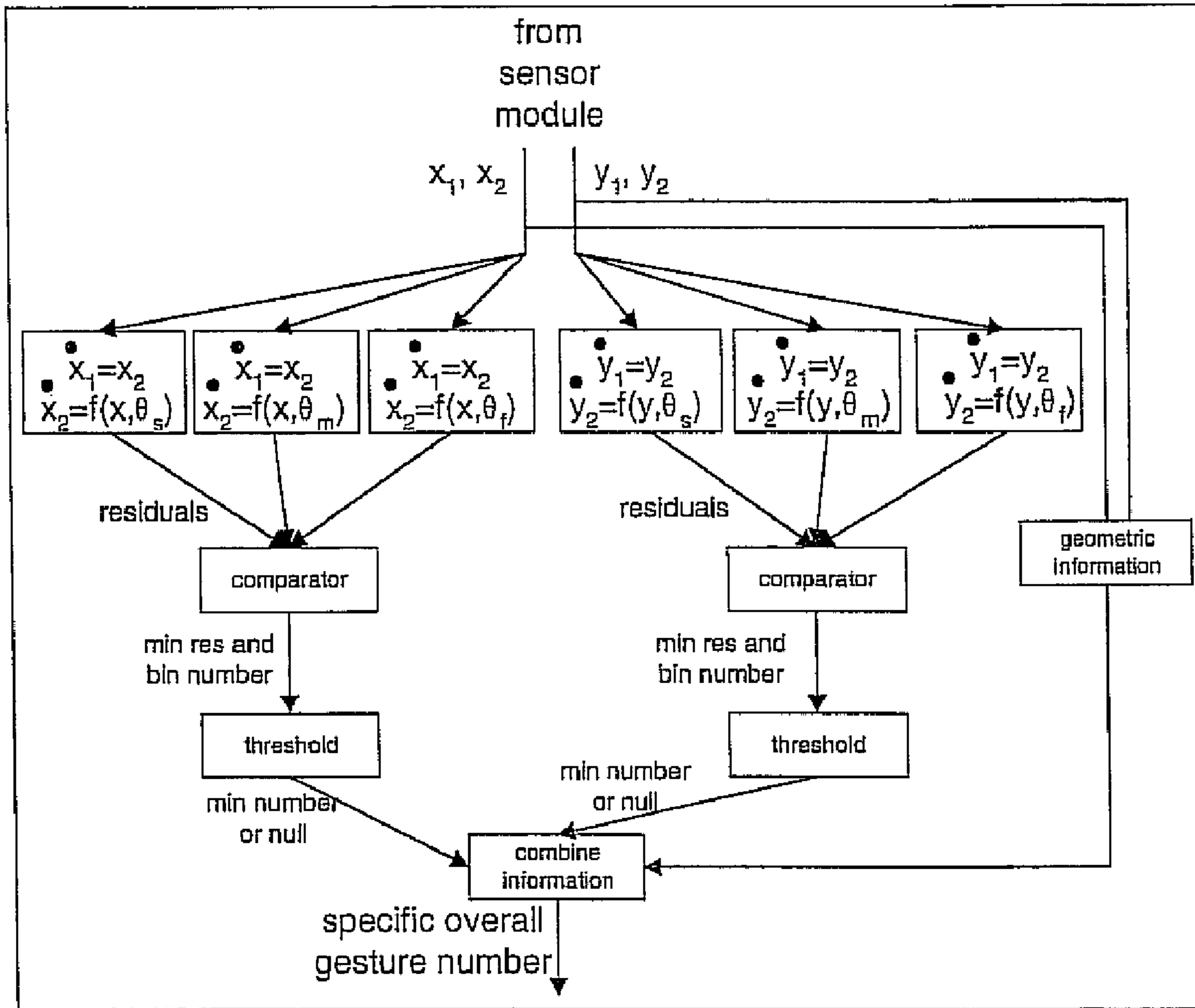
Figure 32: Simplified Diagram of the Dynamic Gesture Prediction Module.
