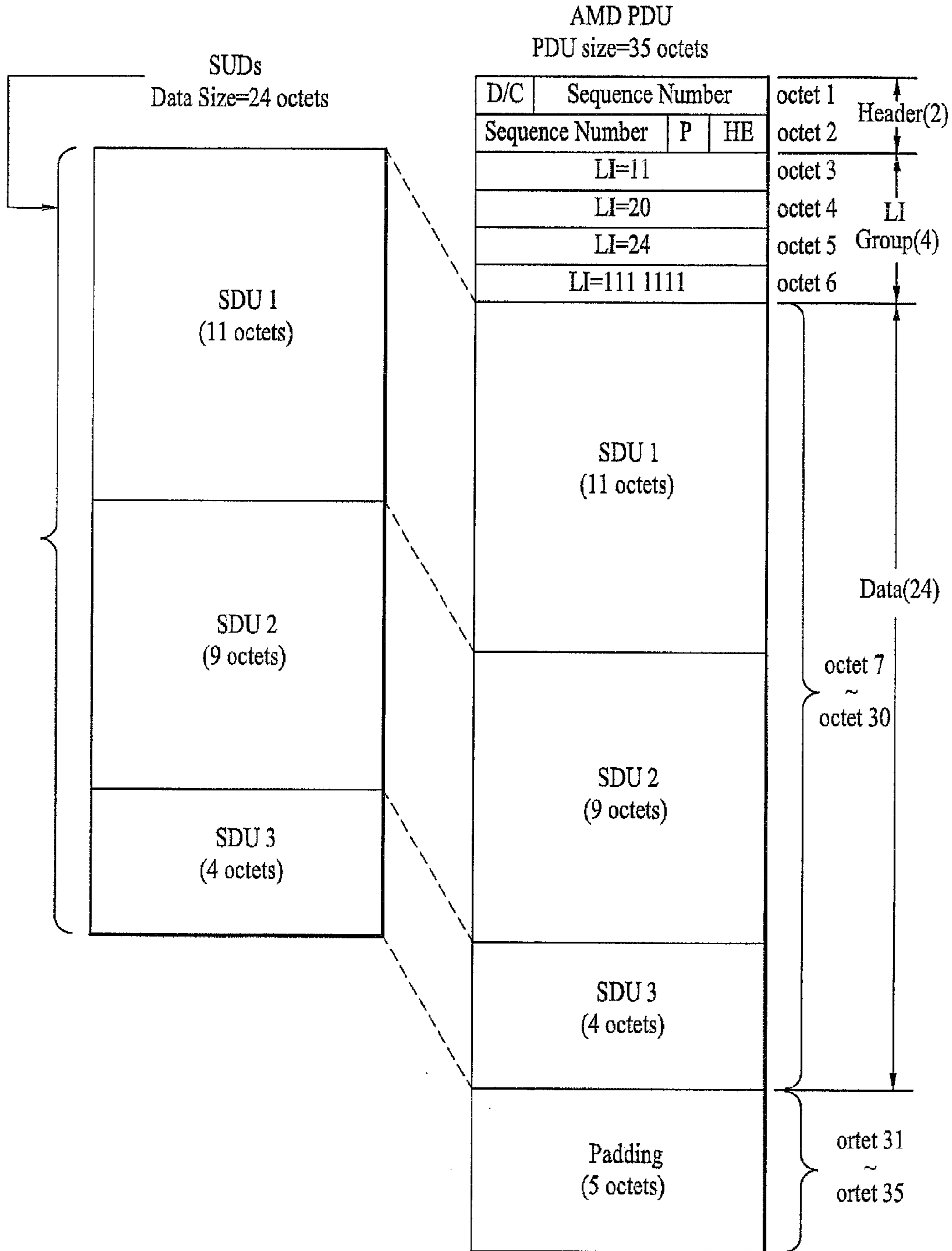
FIG. 3 Related Art
