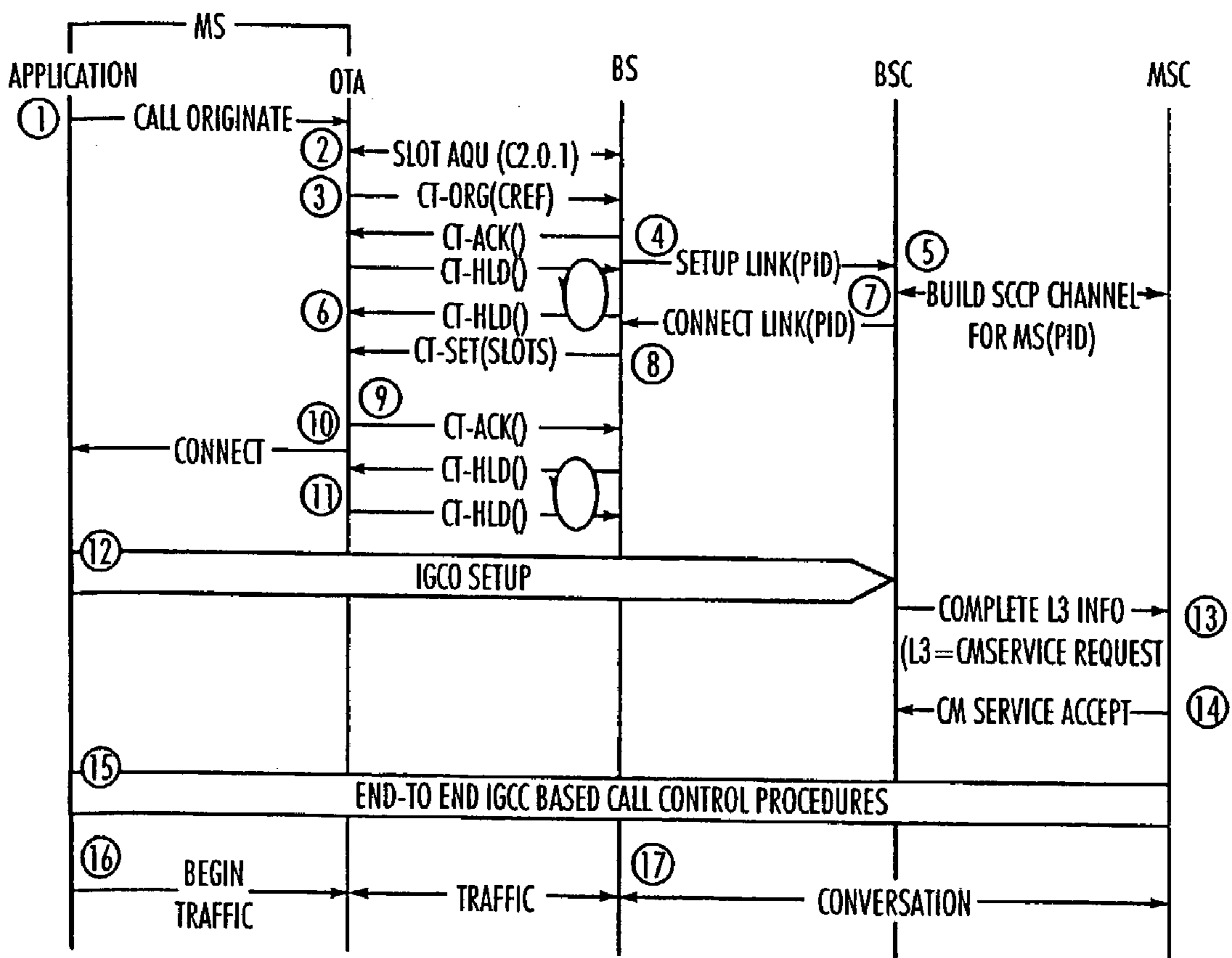
Fig. 9 MOBILE CALL ORIGINATION
