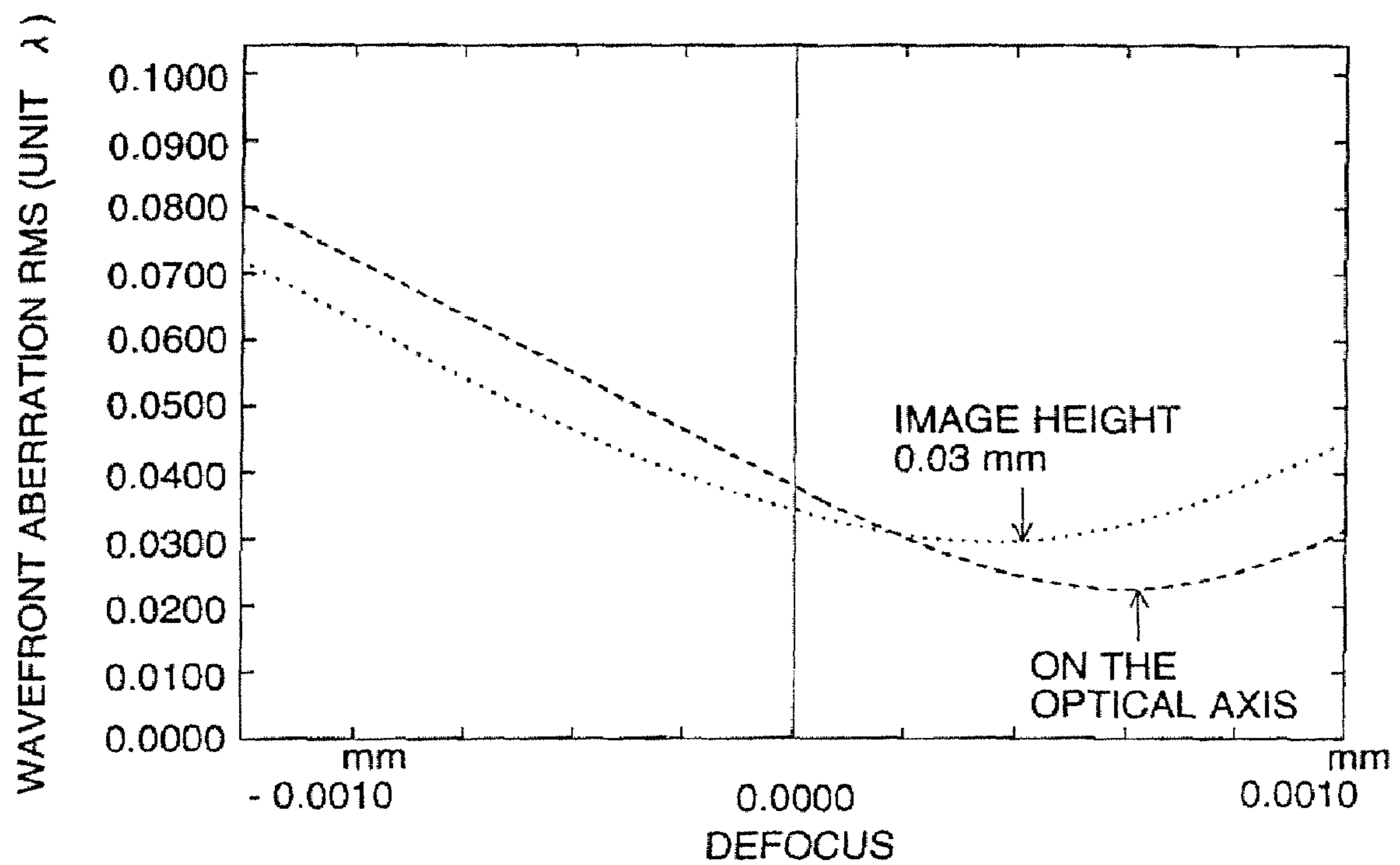
DIAGRAM SHOWING WAVEFRONT ABERRATION RMS FOR WAVELENGTH \lambda = 780\text{nm} IN EXAMPLE 8
