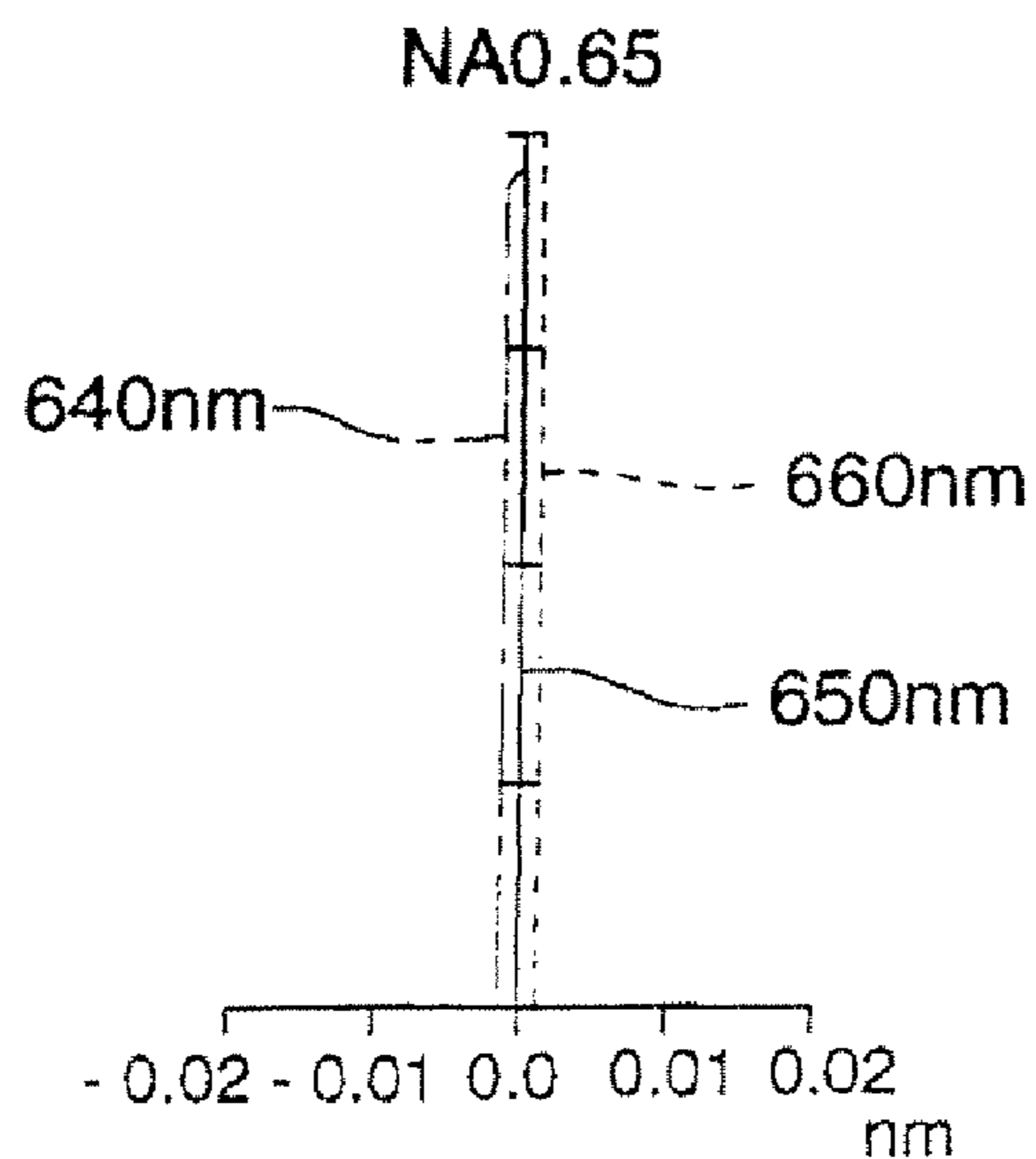
DIAGRAM SHOWING SPHERICAL ABERRATION
