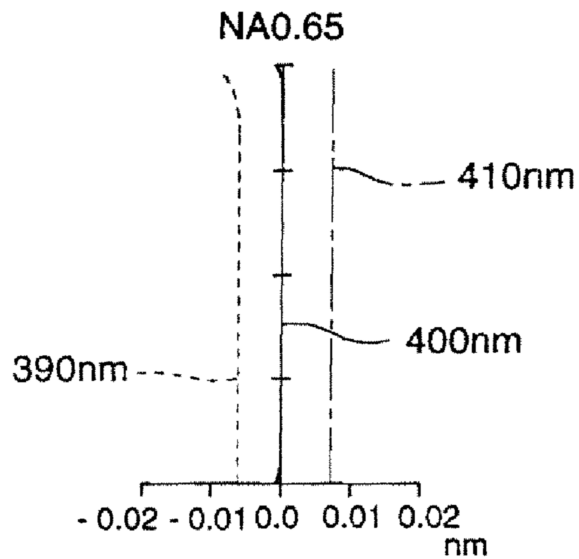
DIAGRAM SHOWING SPHERICAL ABERRATION
