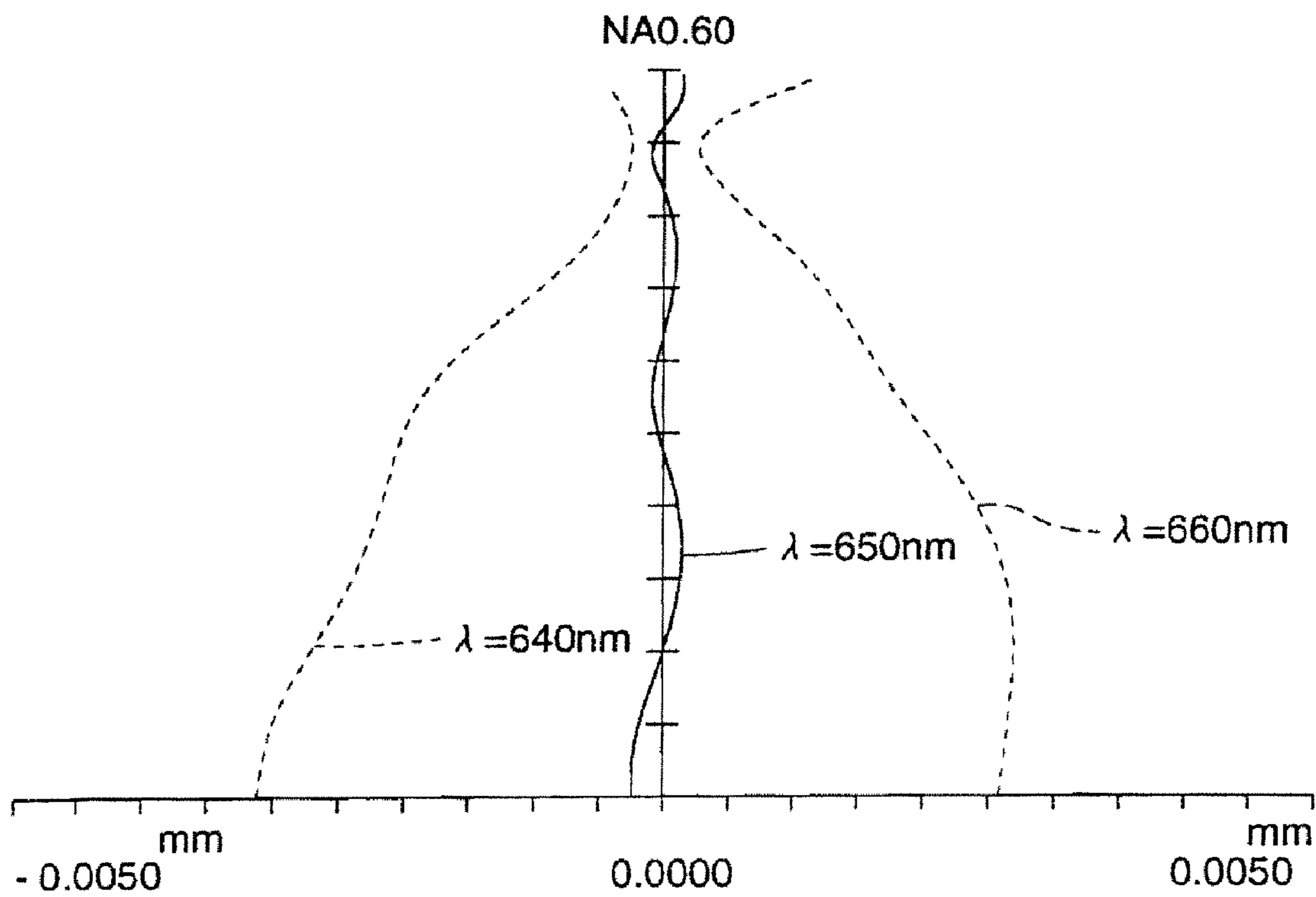
DIAGRAM SHOWING SPHERICAL ABERRATION FOR WAVELENGTH \lambda = 650 \pm 10\text{nm} IN EXAMPLE 6
