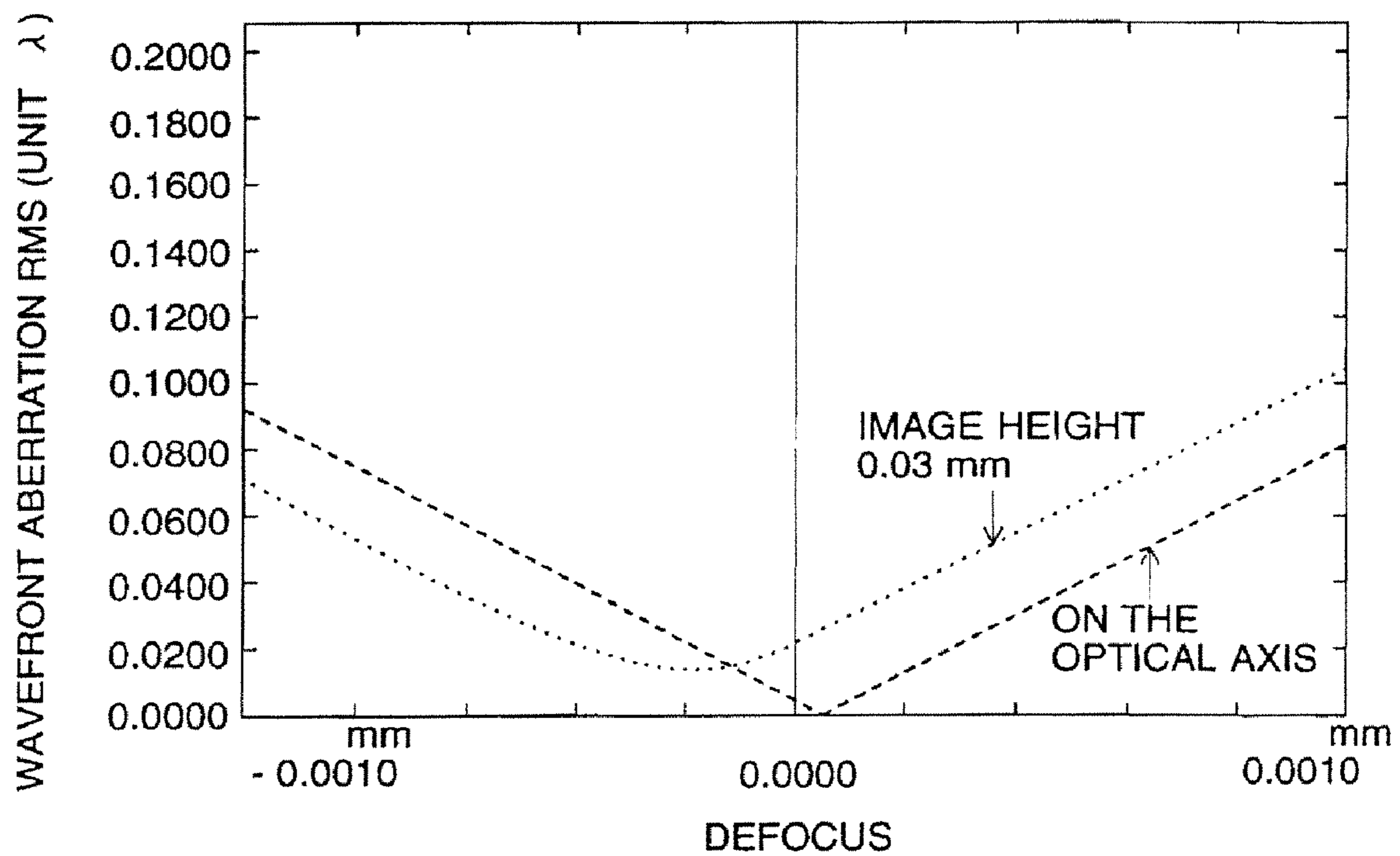
DIAGRAM SHOWING WAVEFRONT ABERRATION RMS FOR WAVELENGTH \lambda = 650\text{nm} IN EXAMPLE 8
