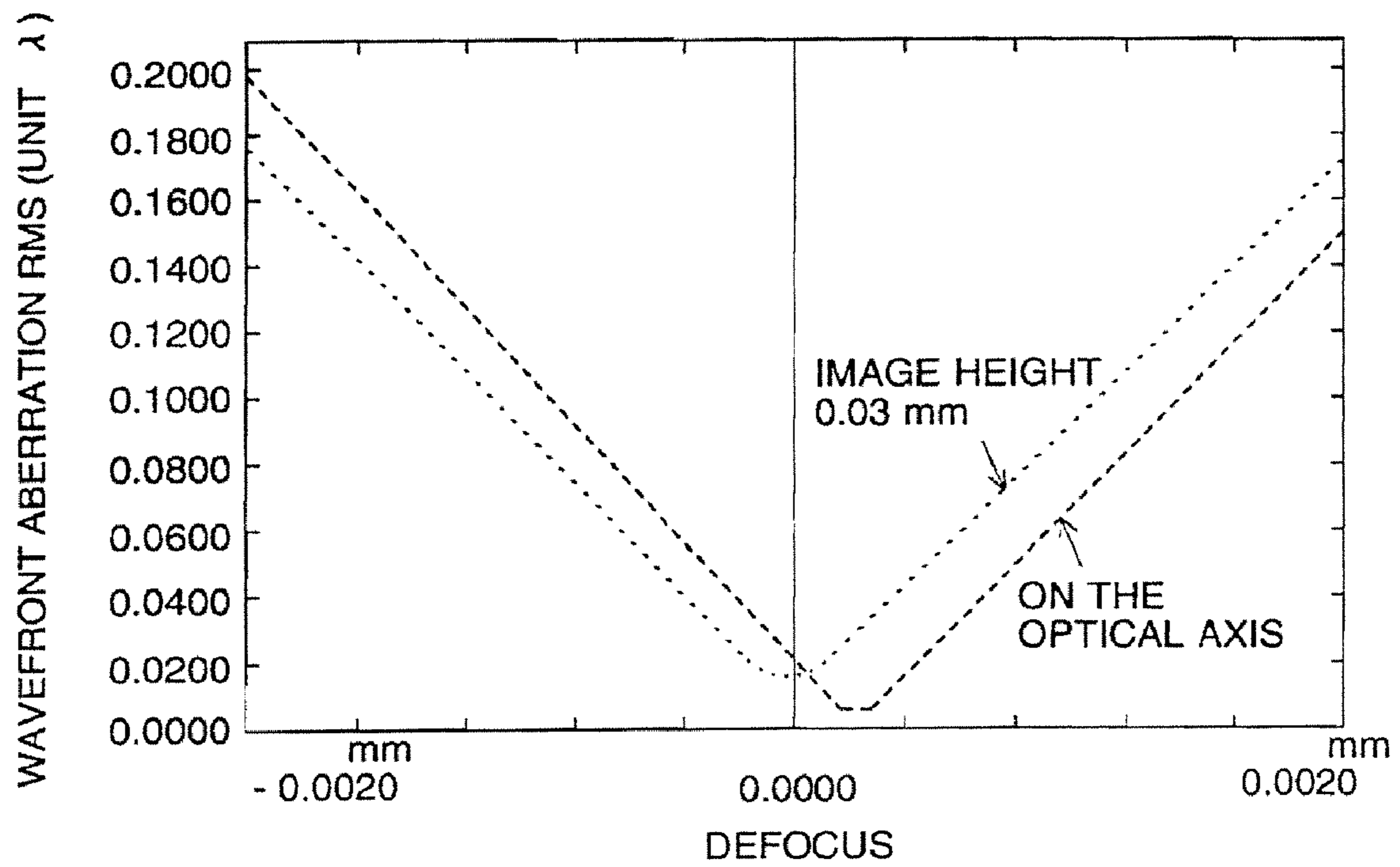
DIAGRAM SHOWING WAVEFRONT ABERRATION RMS FOR WAVELENGTH \lambda = 650\text{nm} IN EXAMPLE 7
