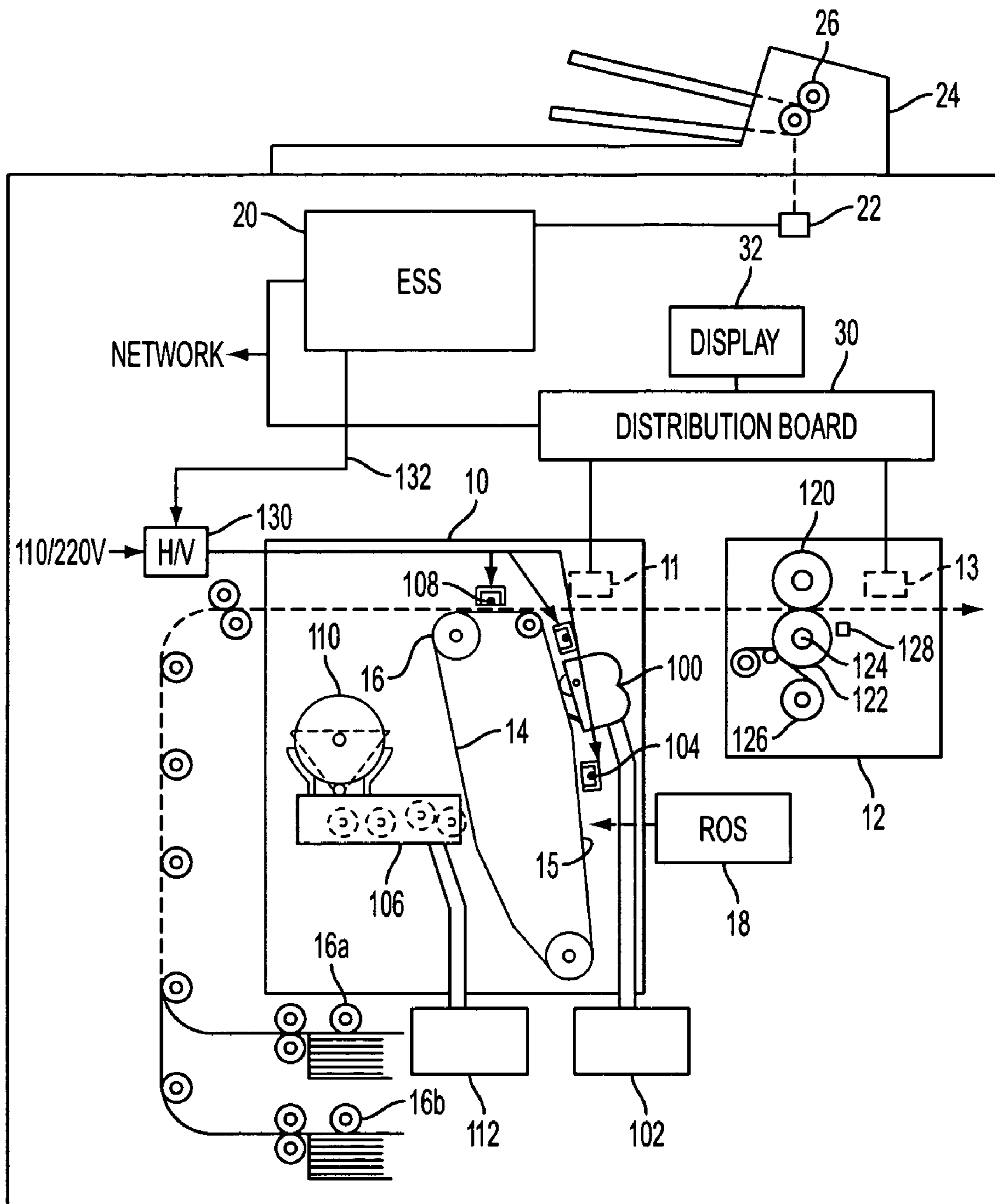
FIG. 1 PRIOR ART
