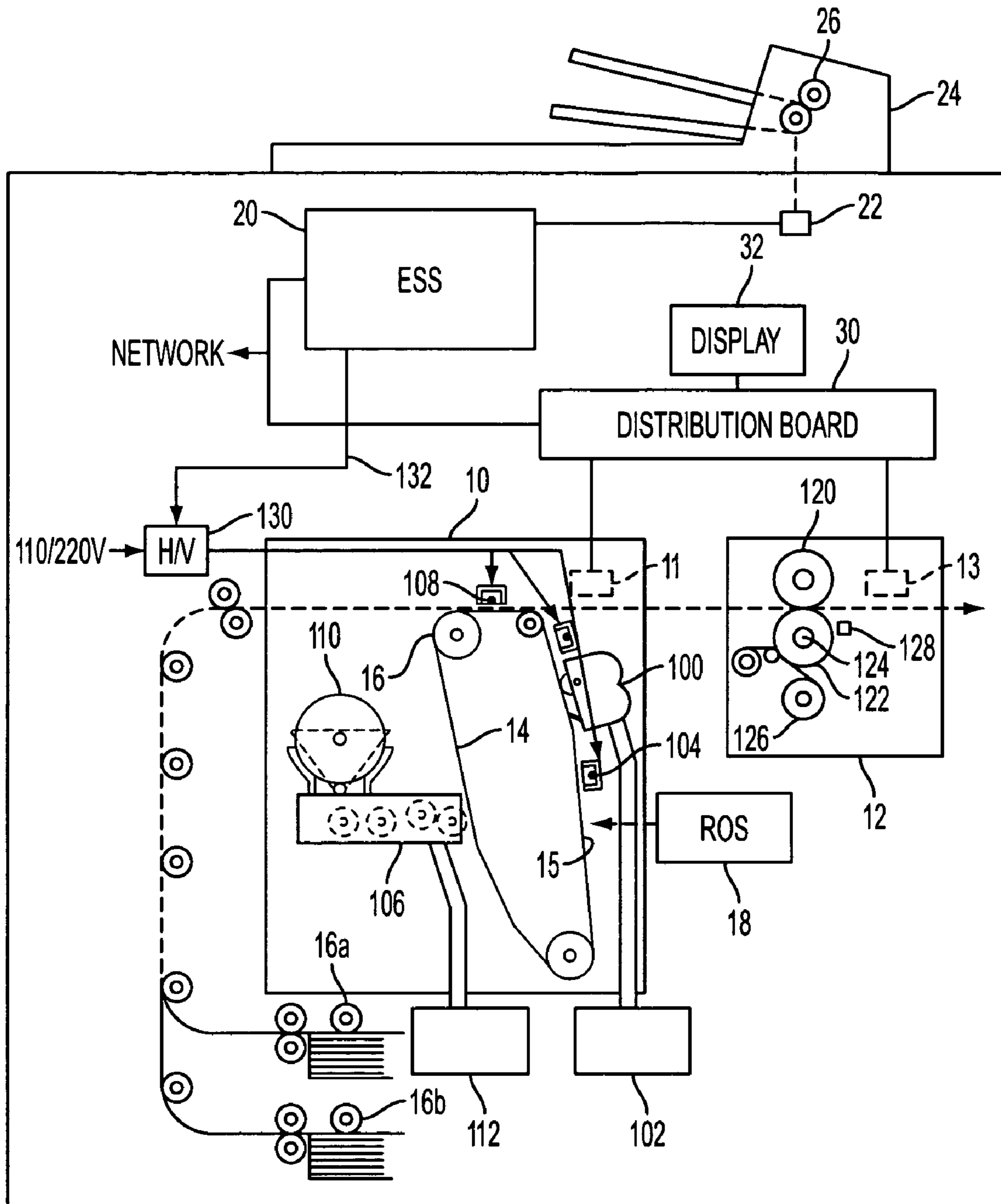
FIG. 1 PRIOR ART
