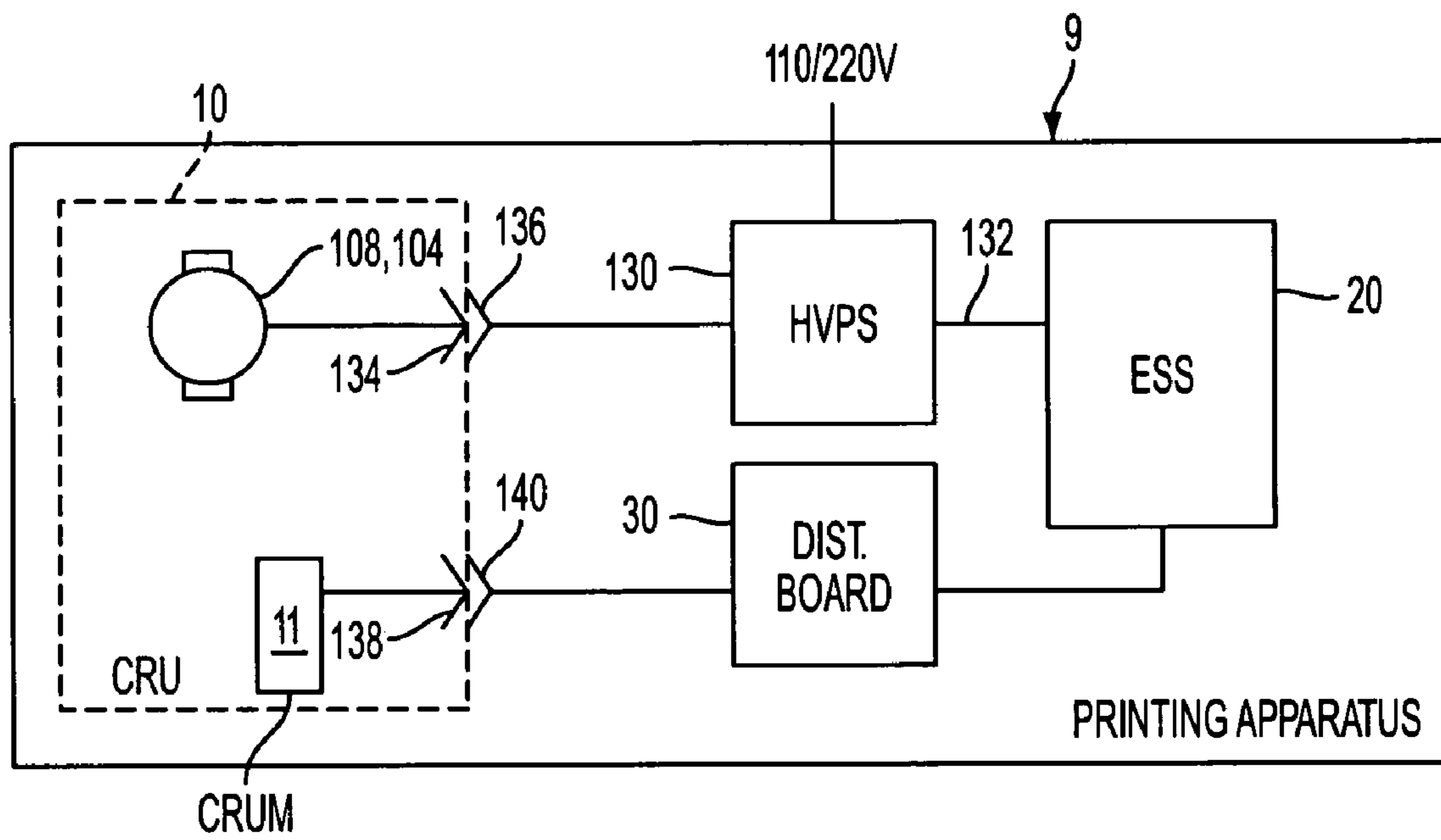
FIG. 2 PRIOR ART
