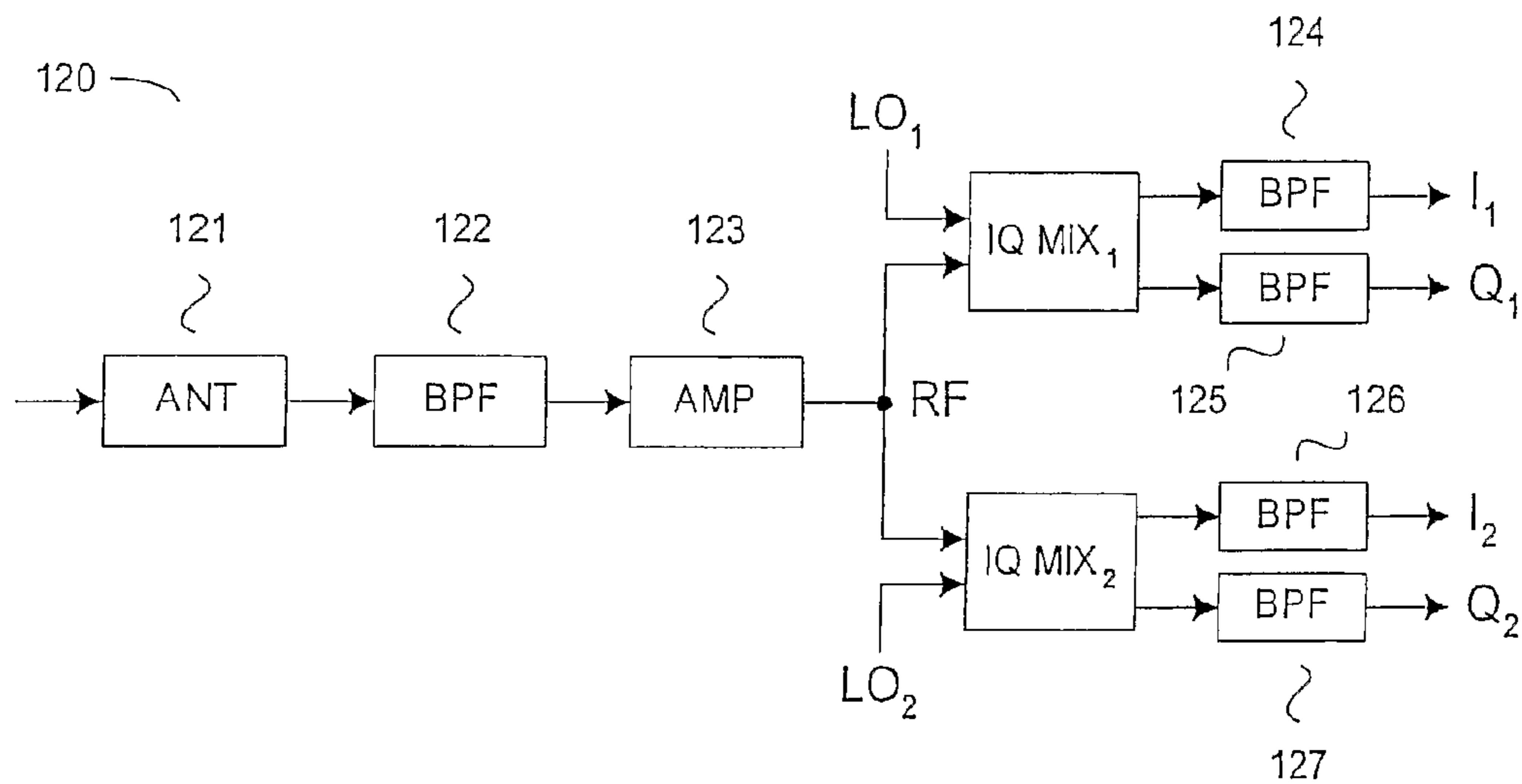
Fig. 1b Receiver (one channel)
