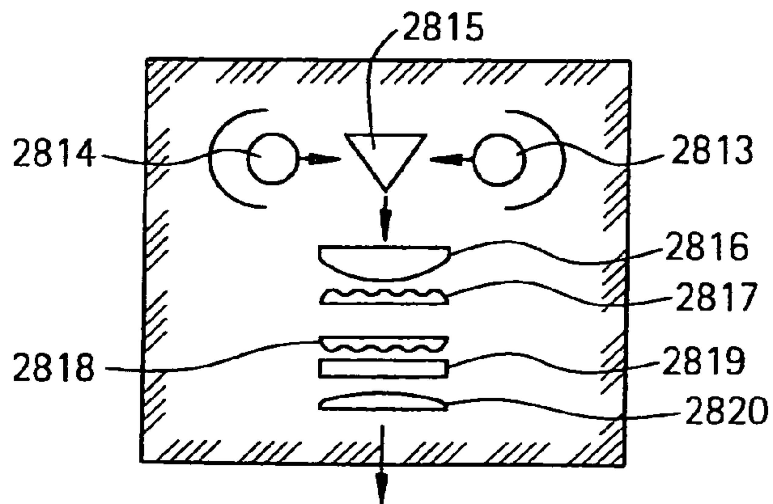
LIGHT SOURCE OPTICAL SYSTEM
