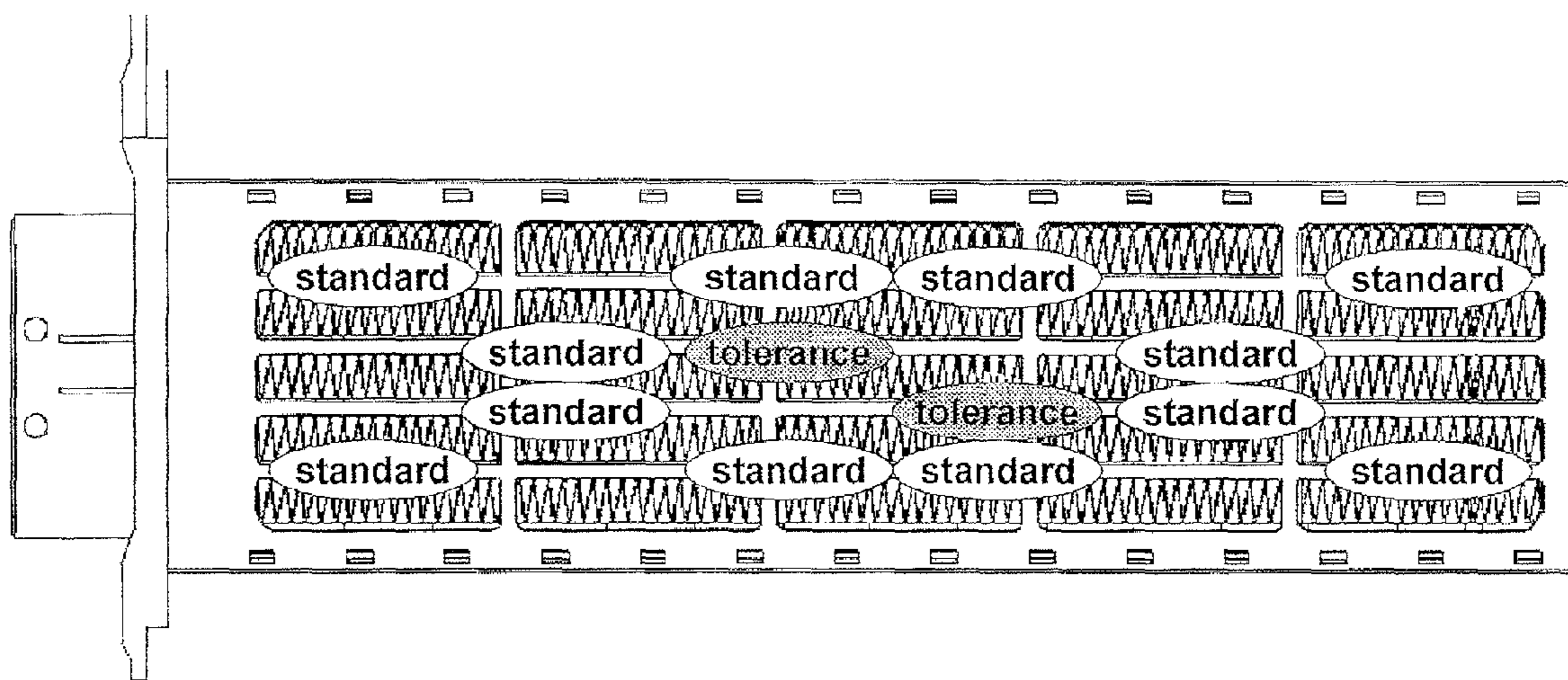
Use of standard PTCs with an R_{25} of 2,10 - 2,60 Ohm
