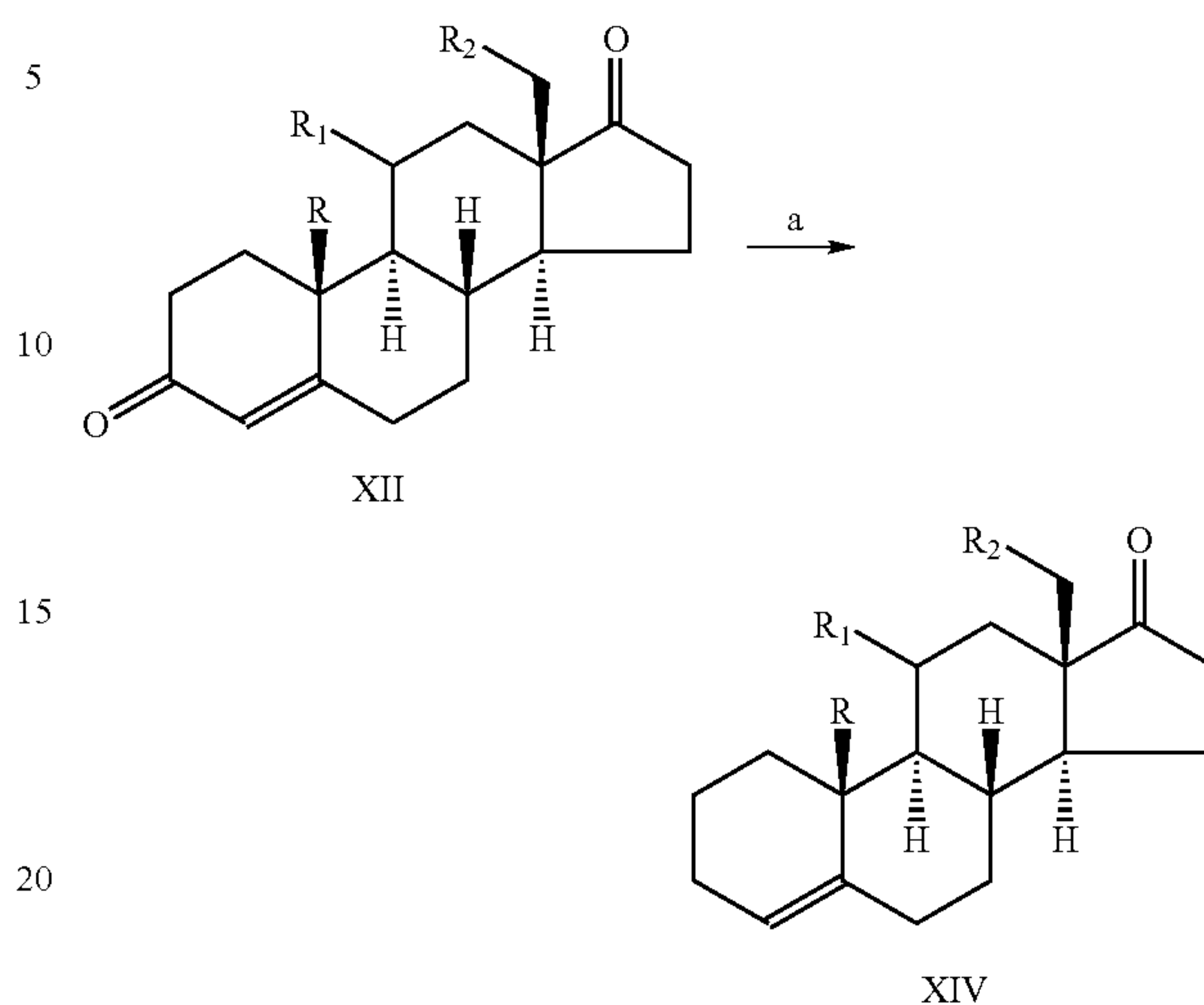
Scheme 5a
