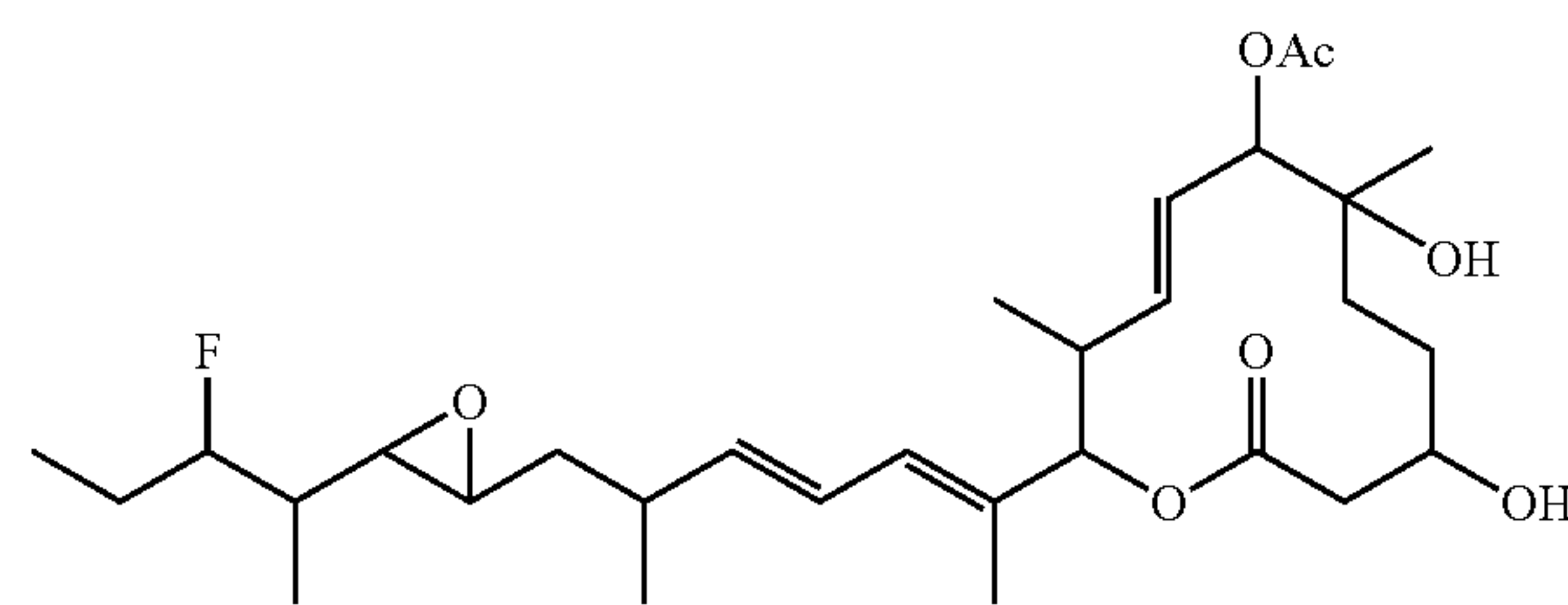
Compound B18-1
