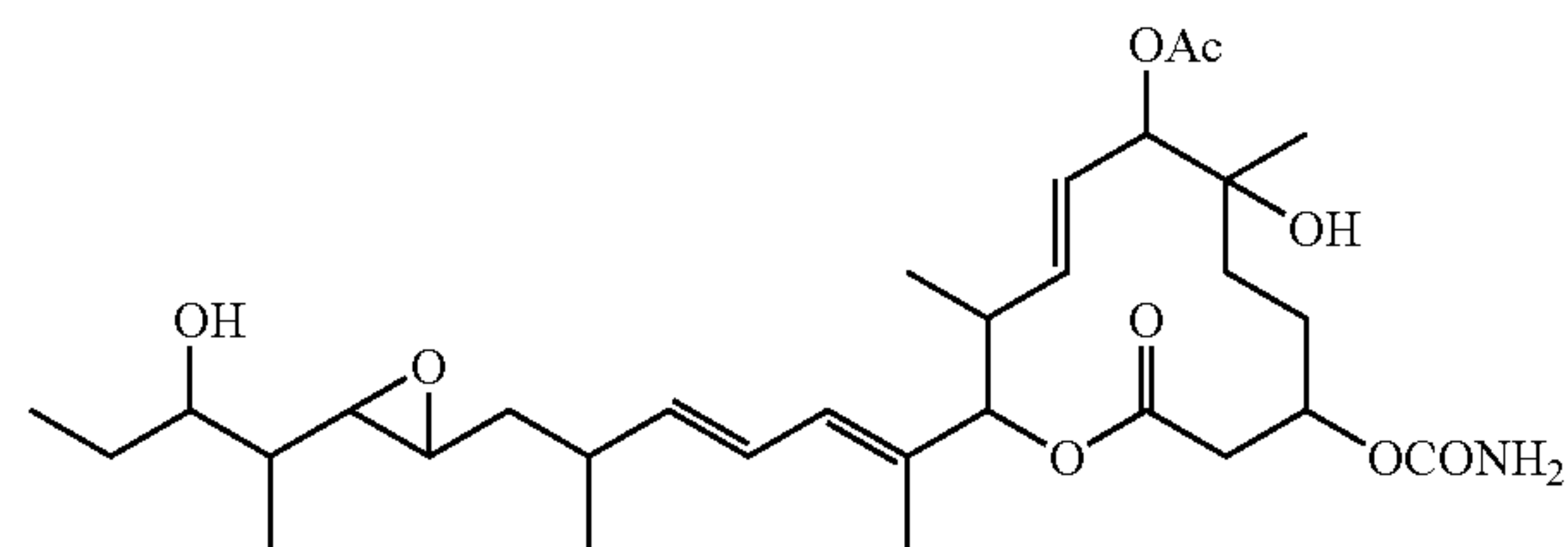
Compound B35-2
