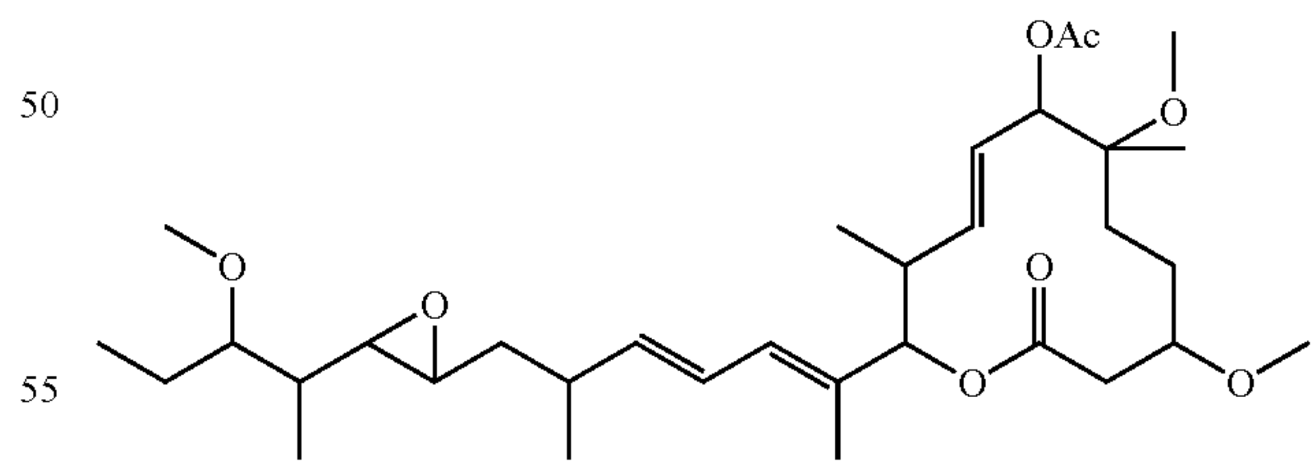
Compound B8-4
