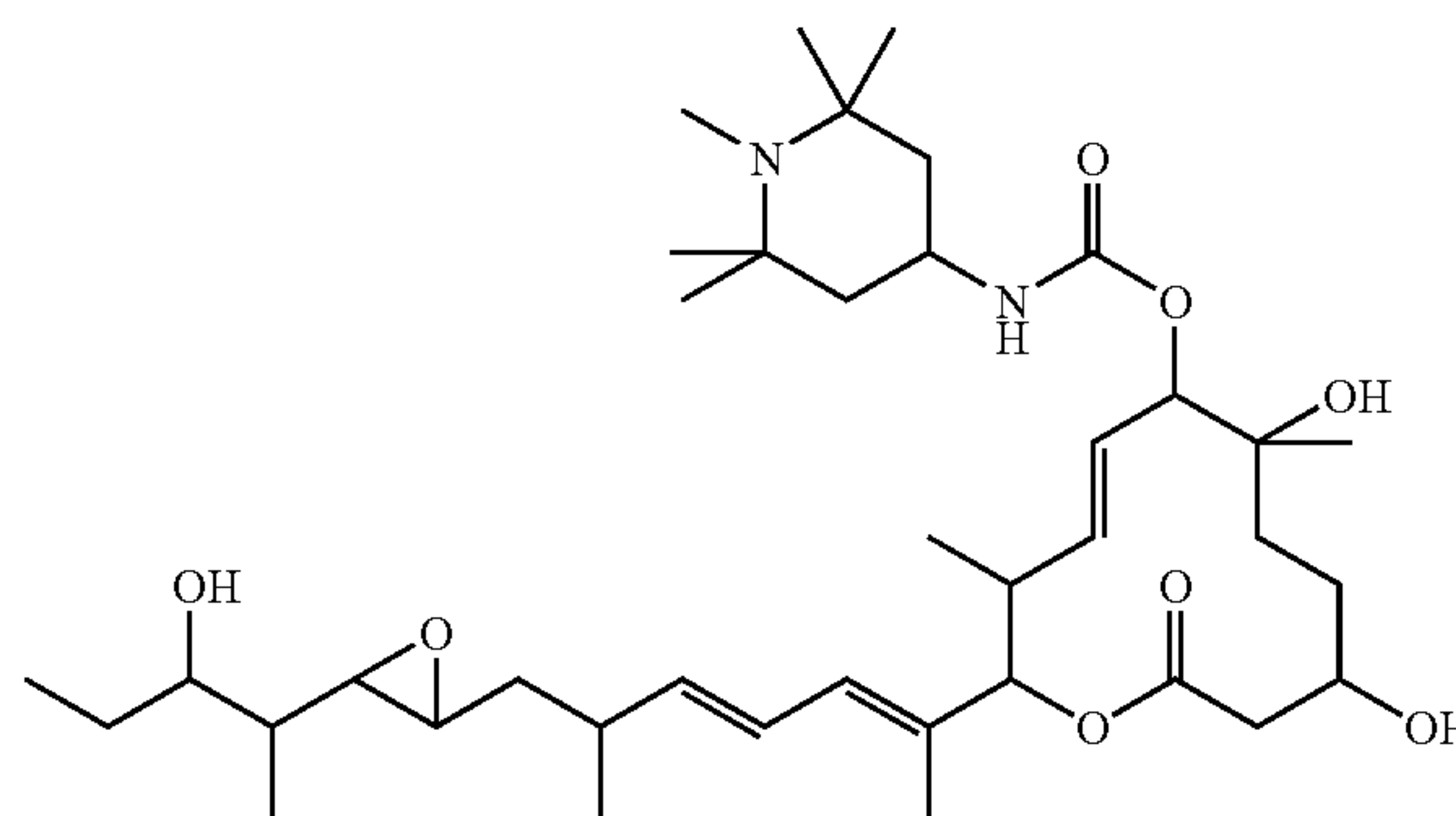
Compound B82
