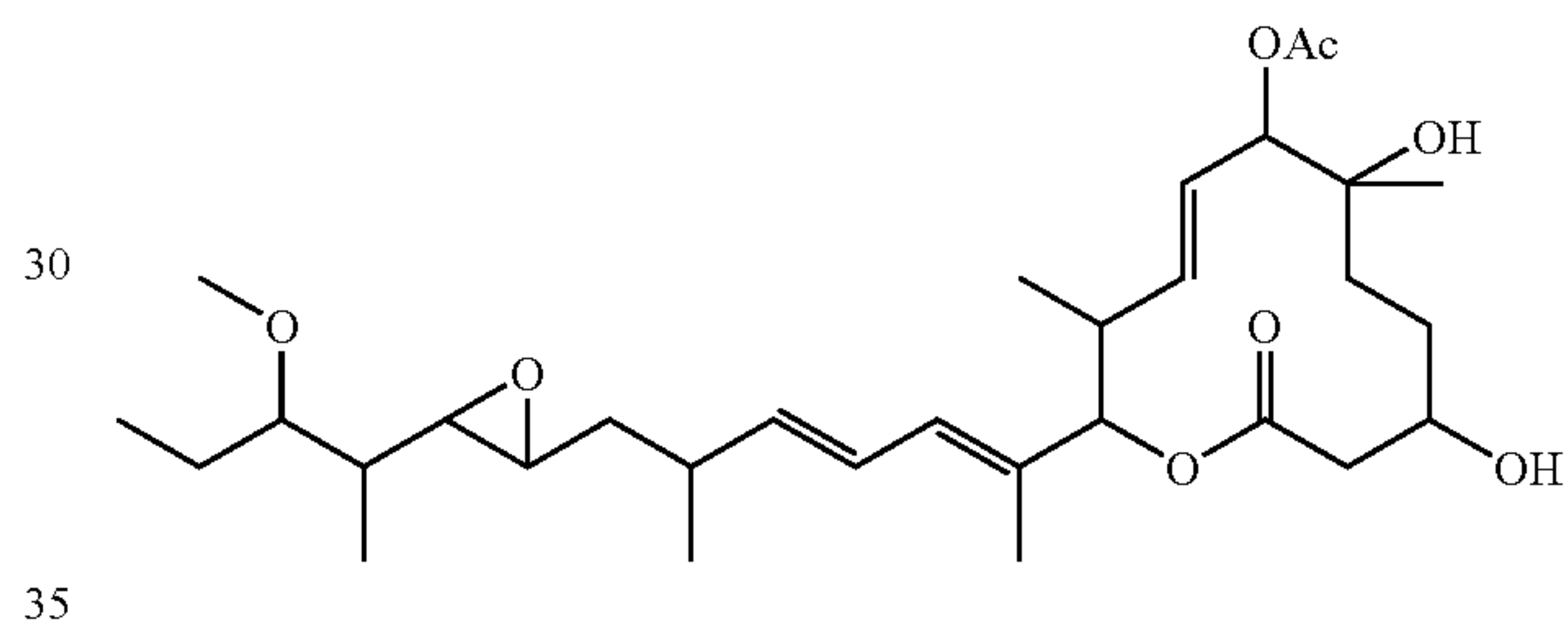
Compound B8-1
