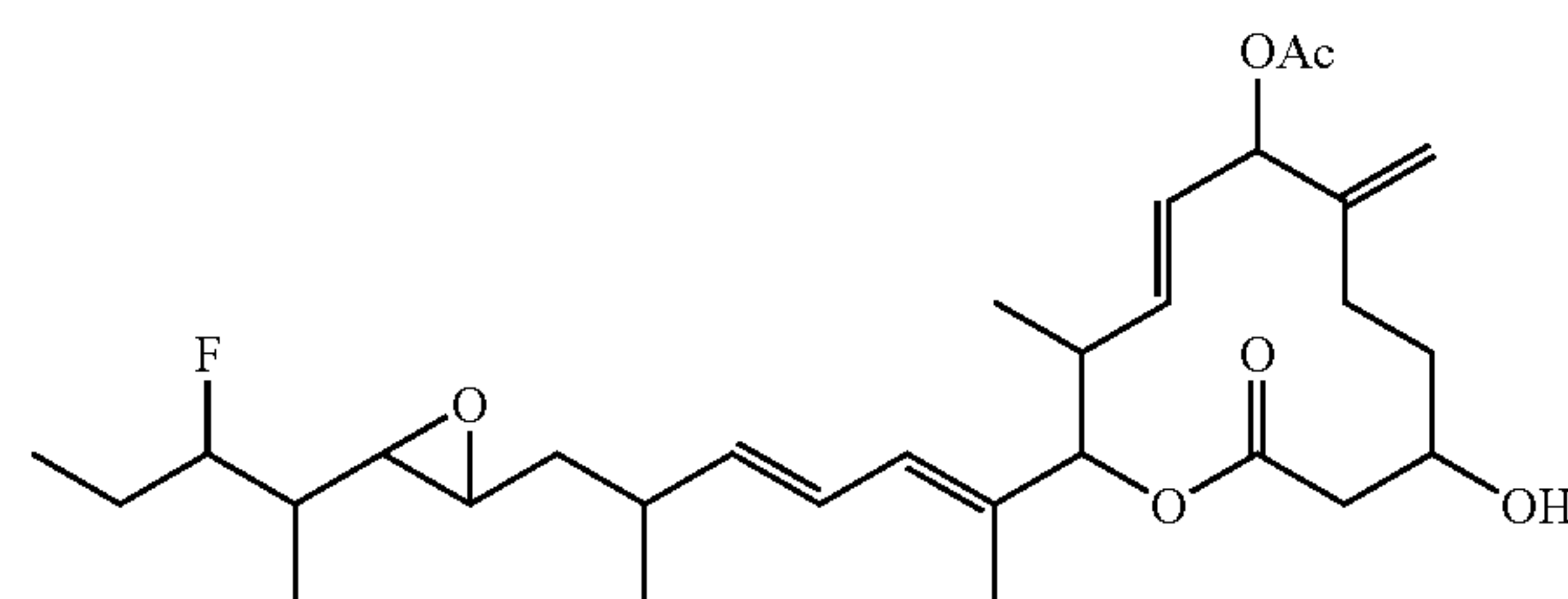
Compound B18-2
