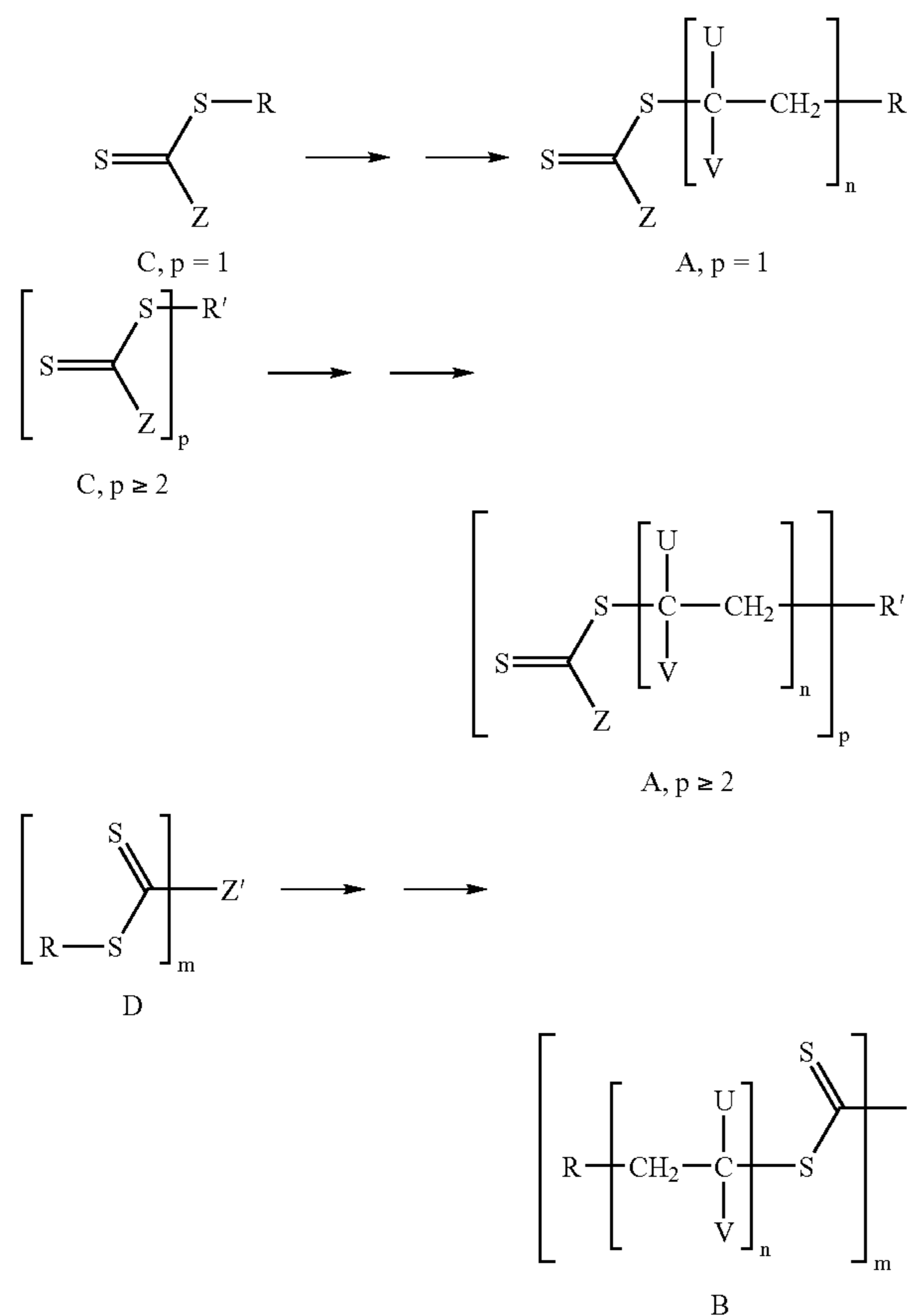
Scheme 4: Formation of linear polymer from CTA of formula C, p = 1
