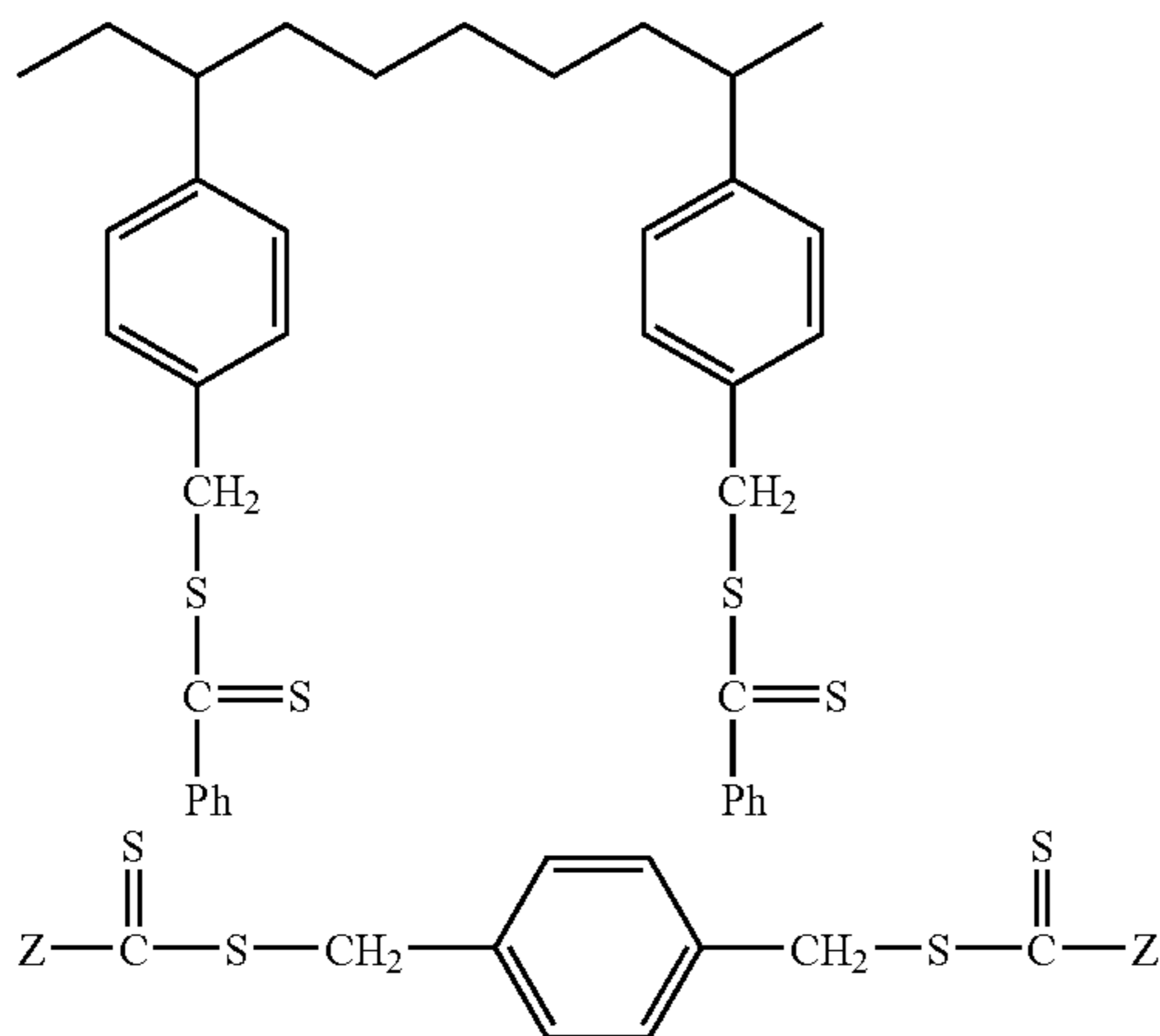
Examples of Multifunctional ( m \geq 2 ) Structures Represented by Formula D
