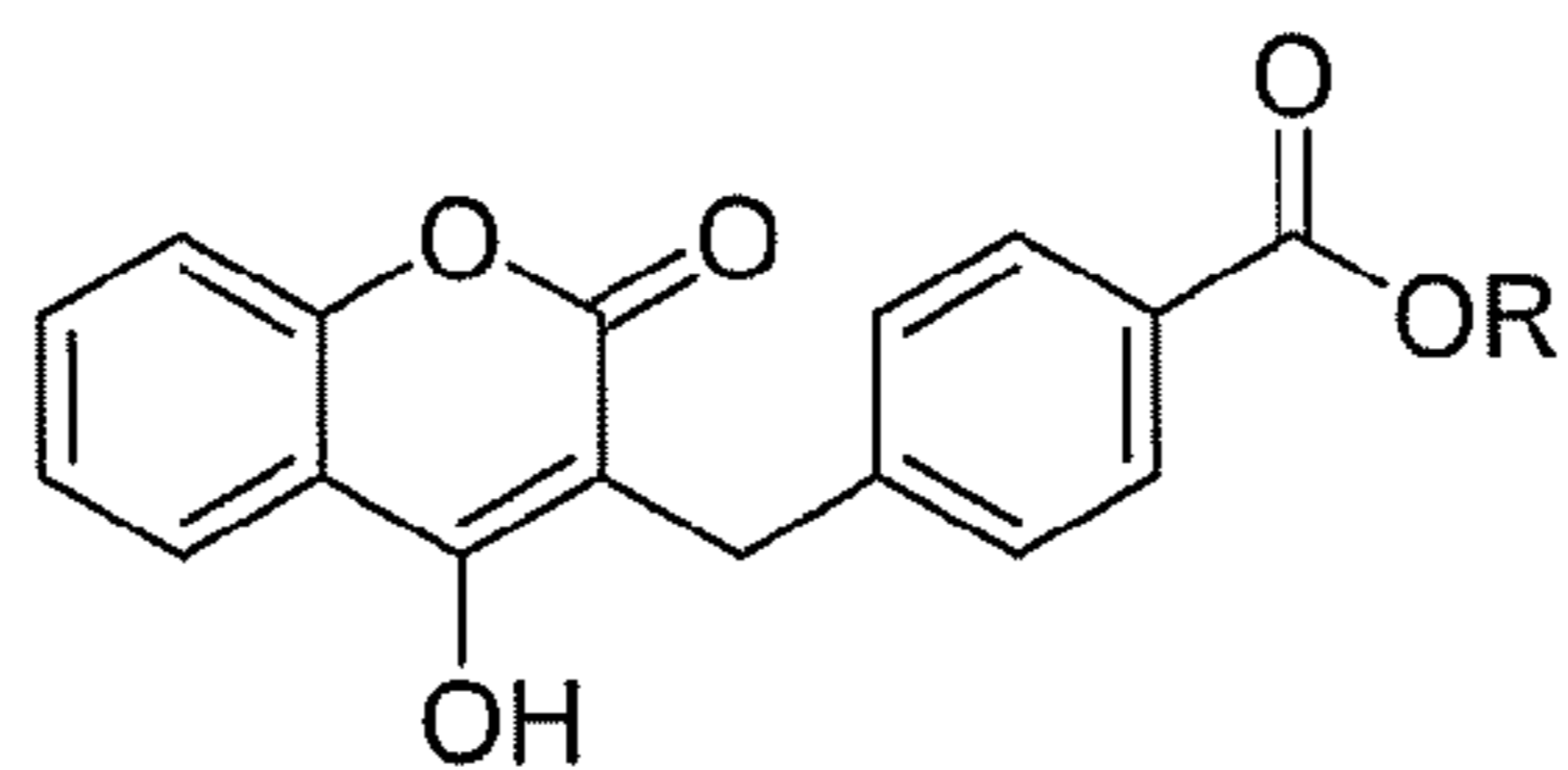
Figure 13 Effect of fluorination on the metabolism by cytochrome P450 and esterase in pooled human microsomes
