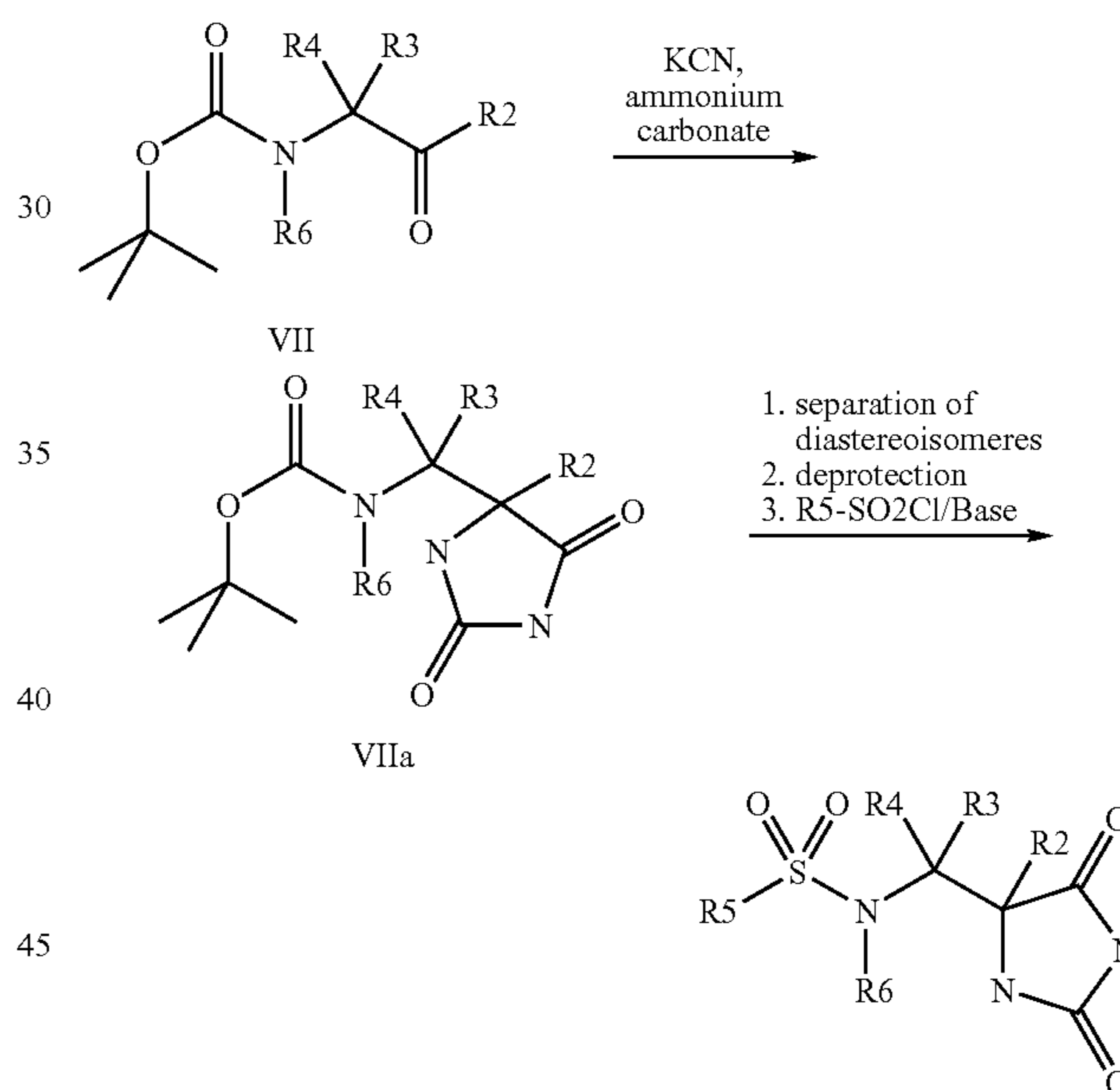
Scheme 2:
