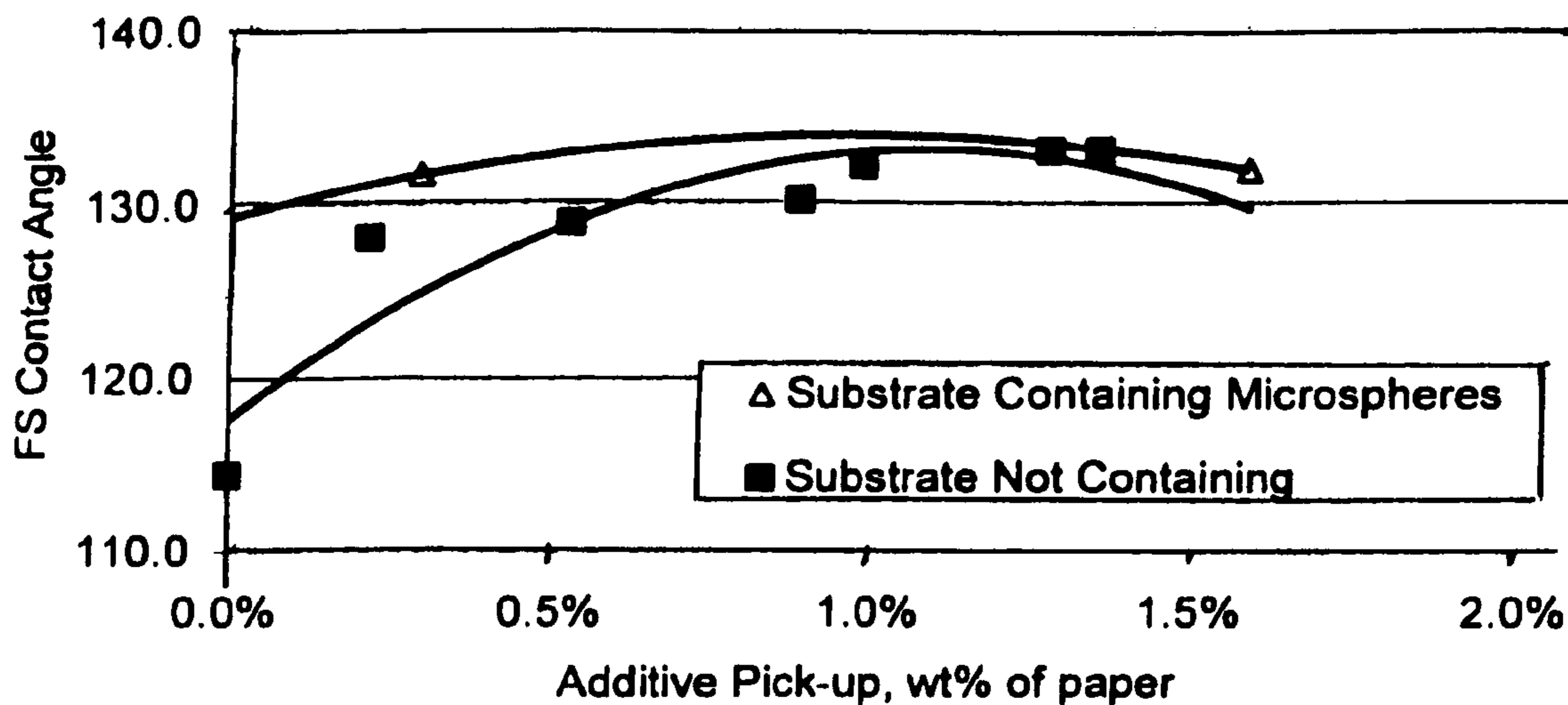
Fig. 3. Felt Side Contact Angle
