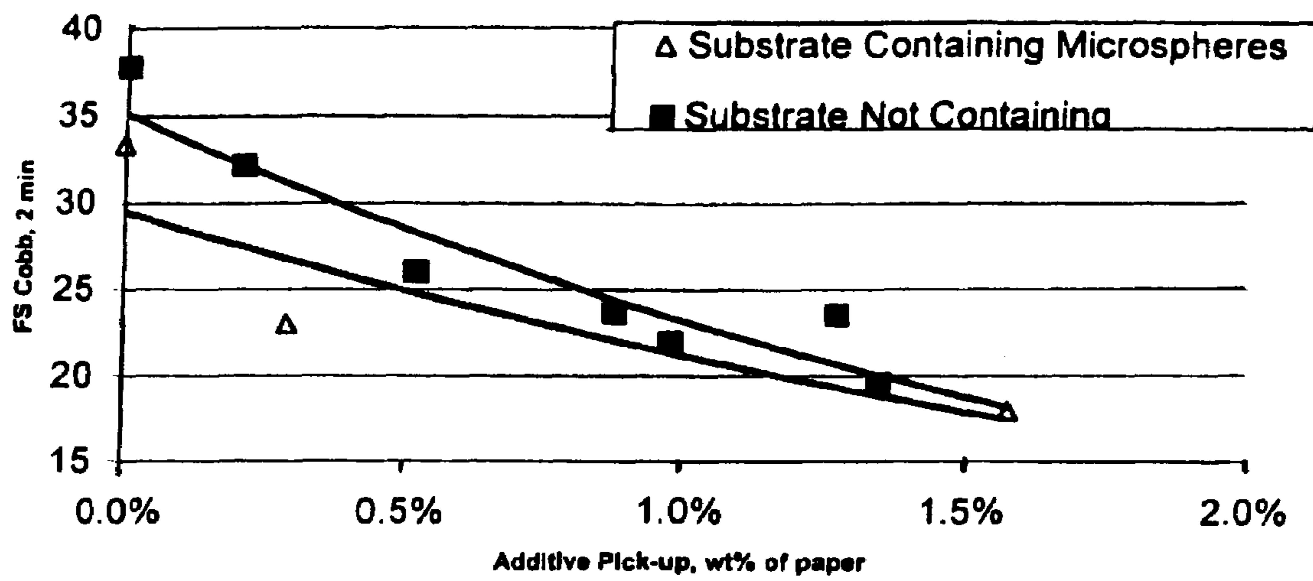
Fig. 1. Felt Side Cobb Size Test
