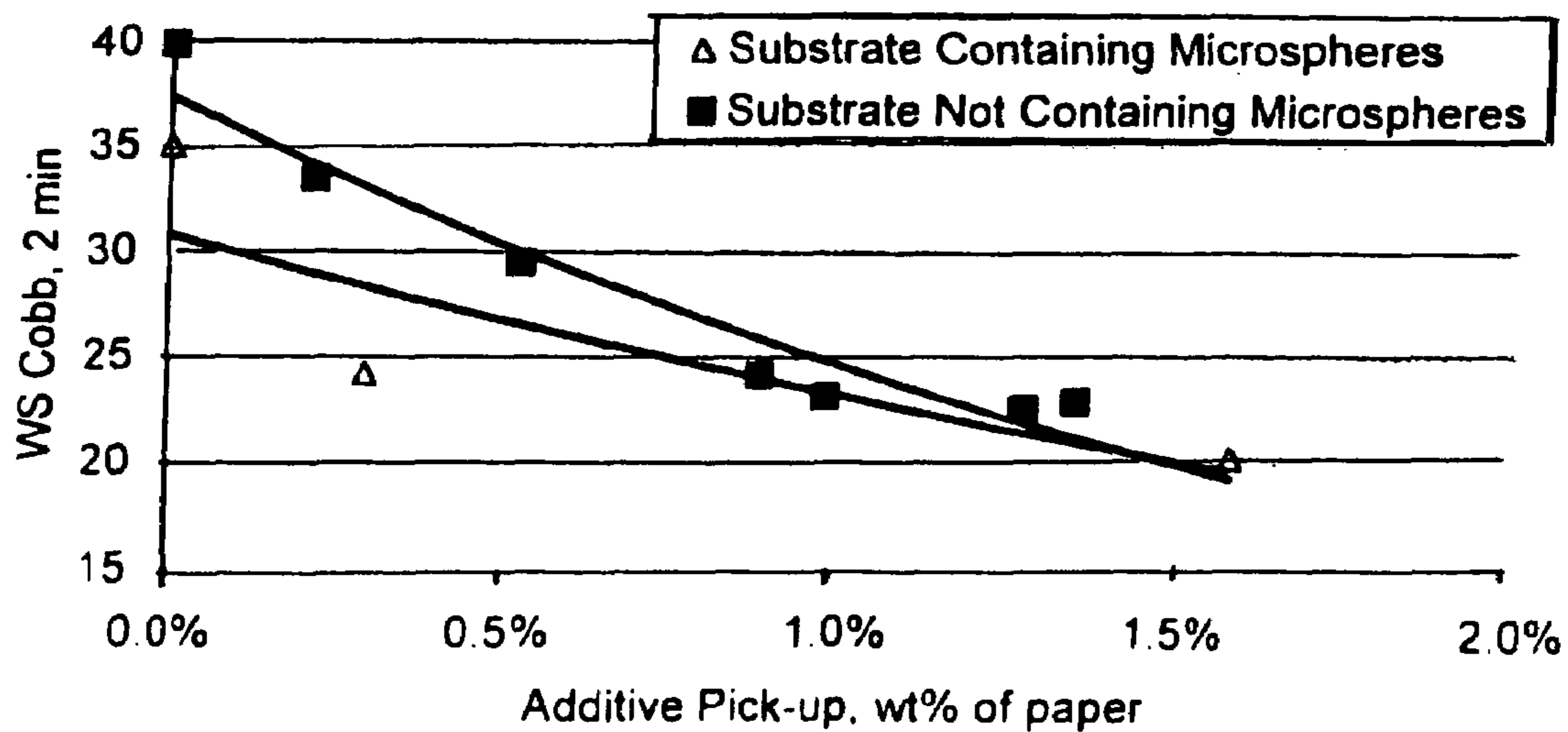
Fig. 2. Wire Side Cobb Size Test
