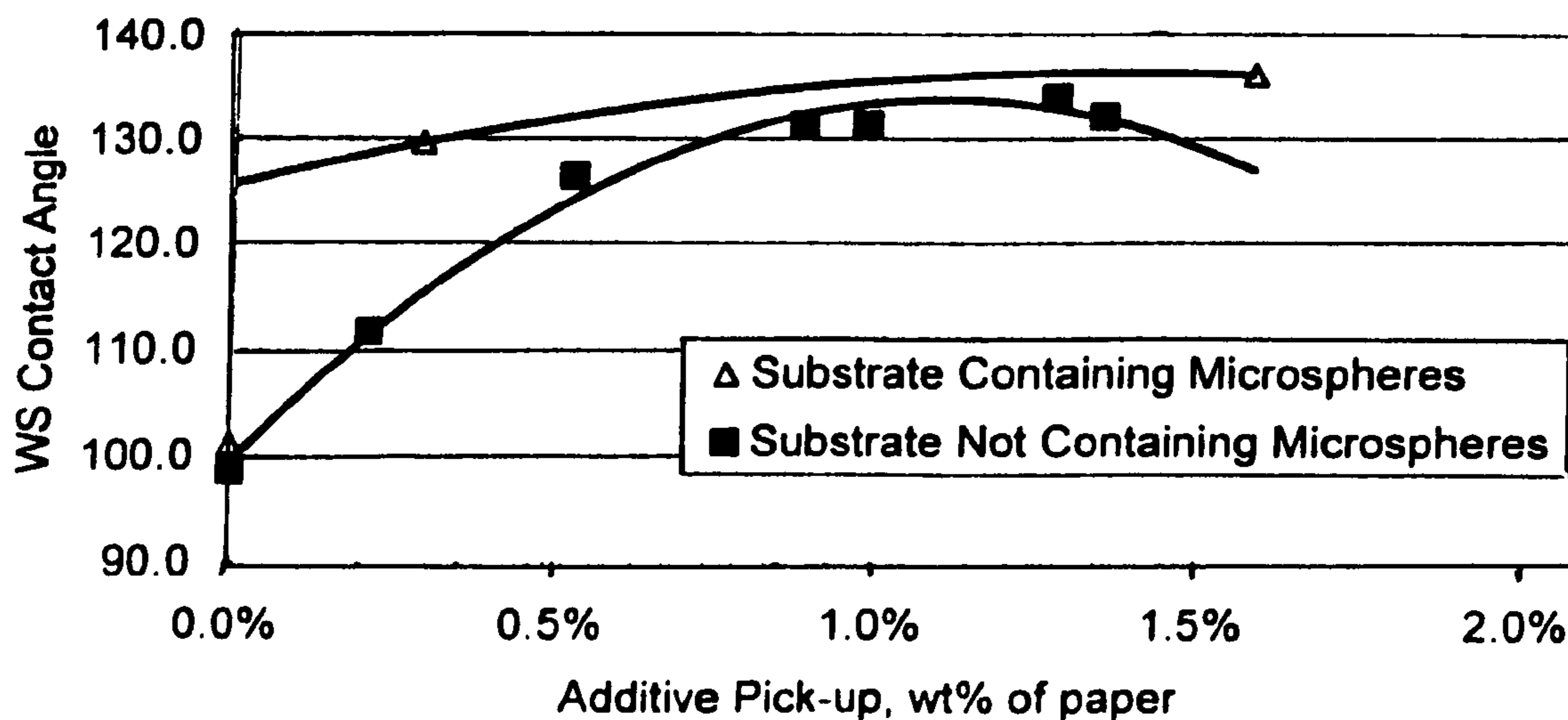
Fig. 4. Wire Side Contact Angle
