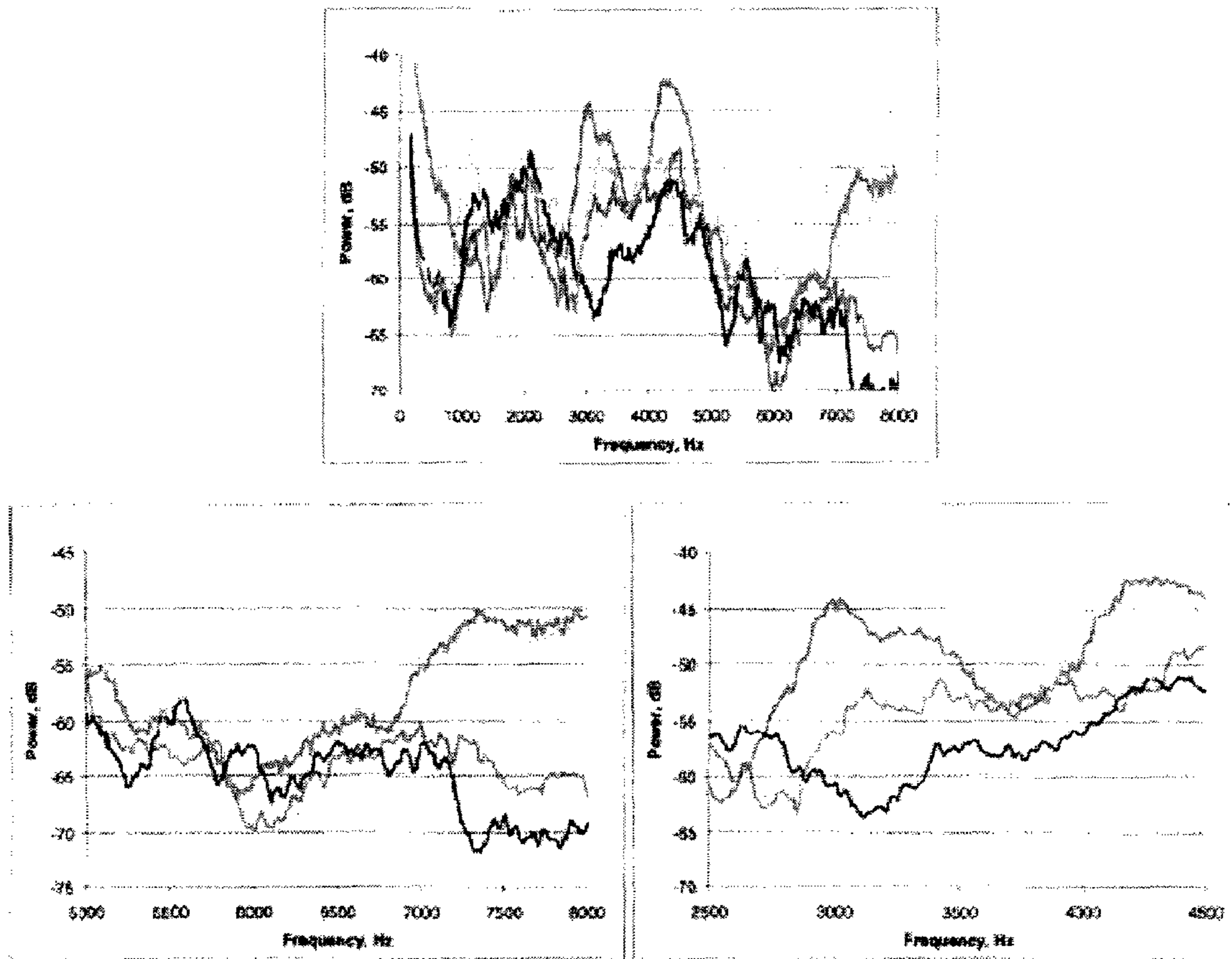
Power spectra of liquid flow through an XR11004 fan nozzle @ 40 psi. Legend: Blue = water Red = syrup Black = water+detergent
