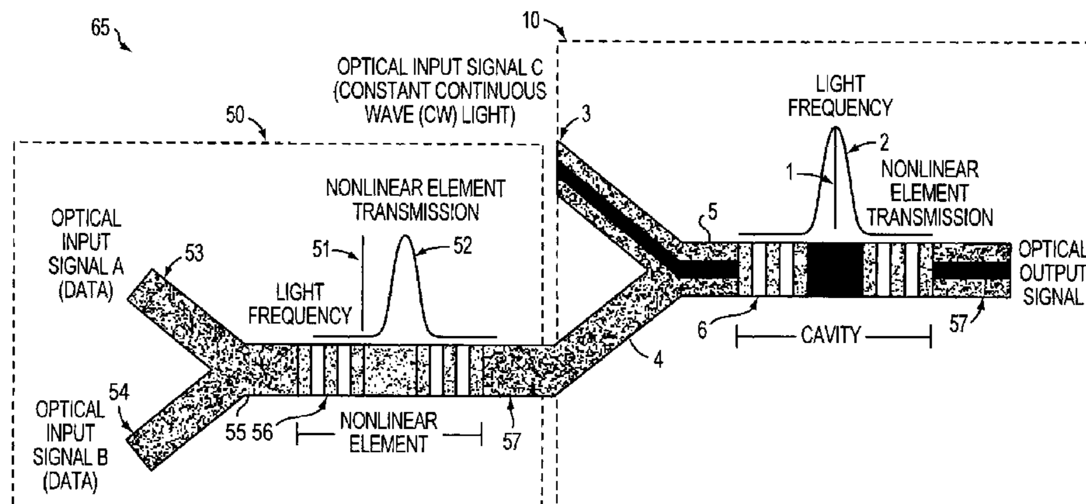
ALL-OPTICAL XNOR GATE WITH LOGIC LEVEL RESTORATION
