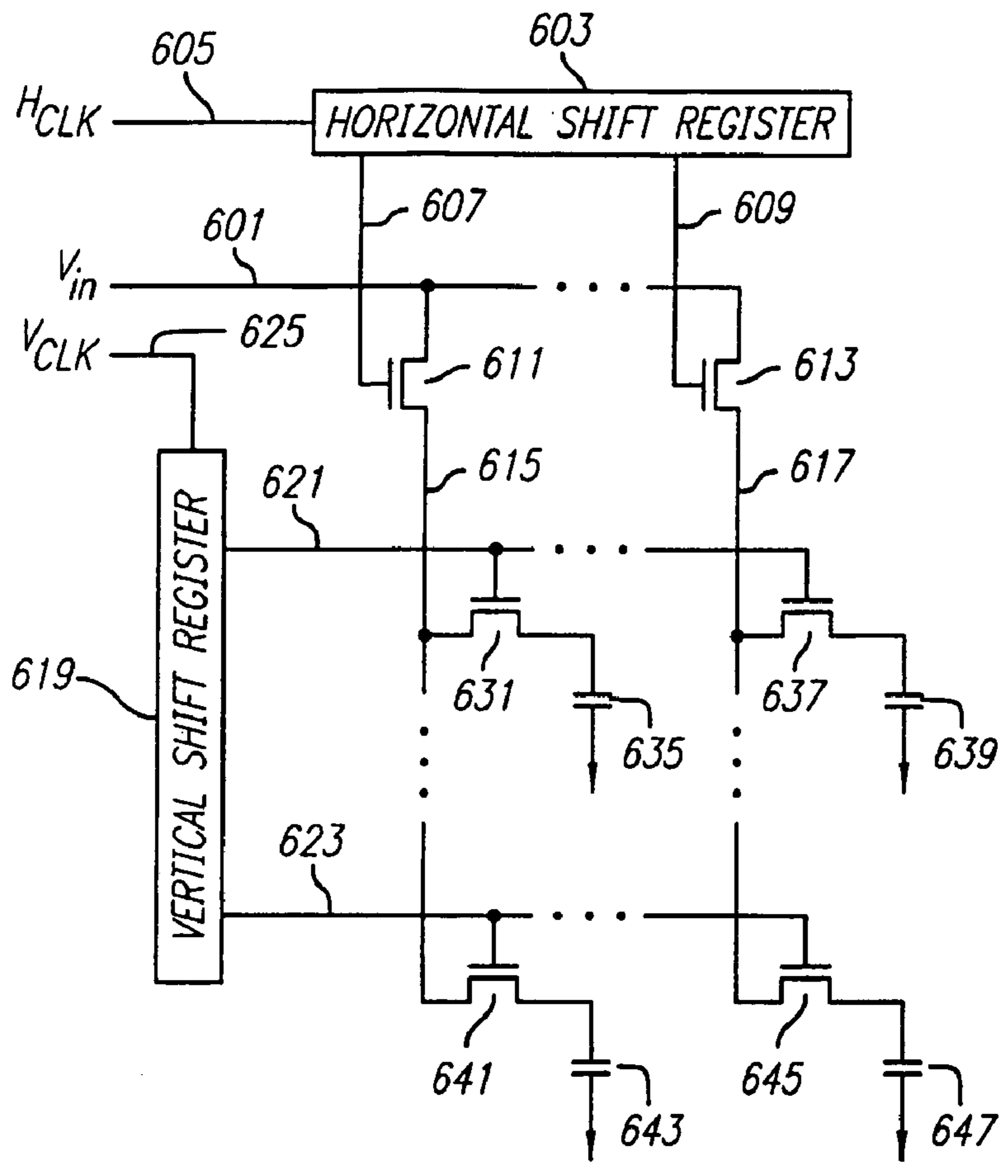
FIG. 12 PRIOR ART
