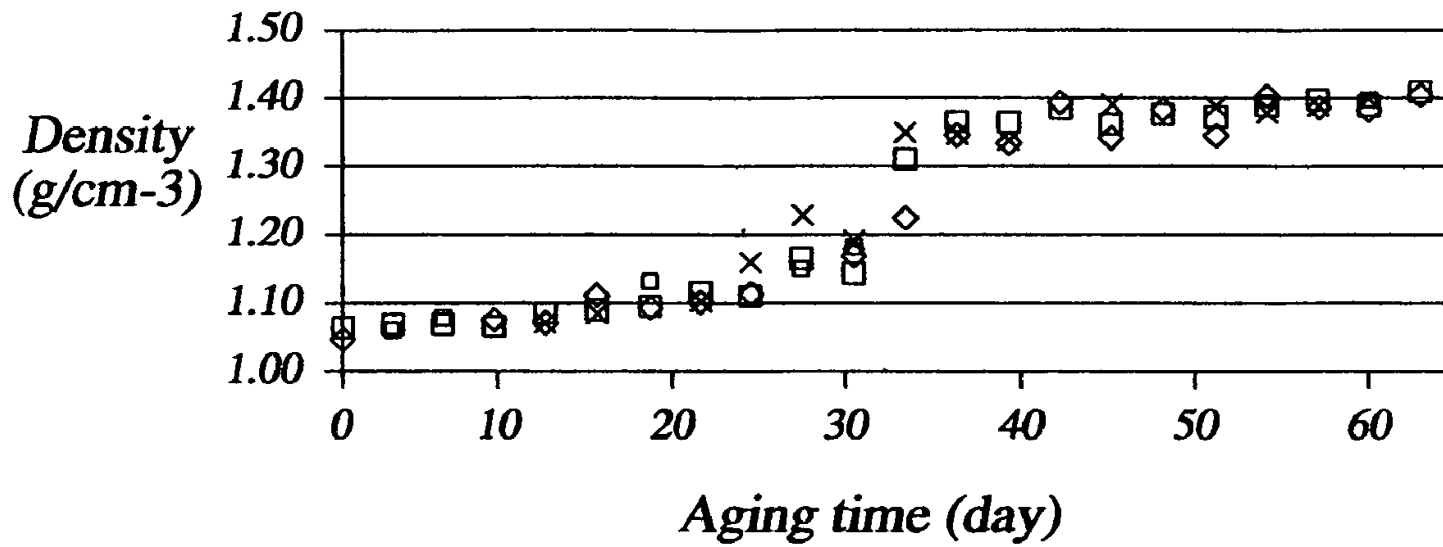
Density of sample with 25% carbon black versus aging time at 125C
