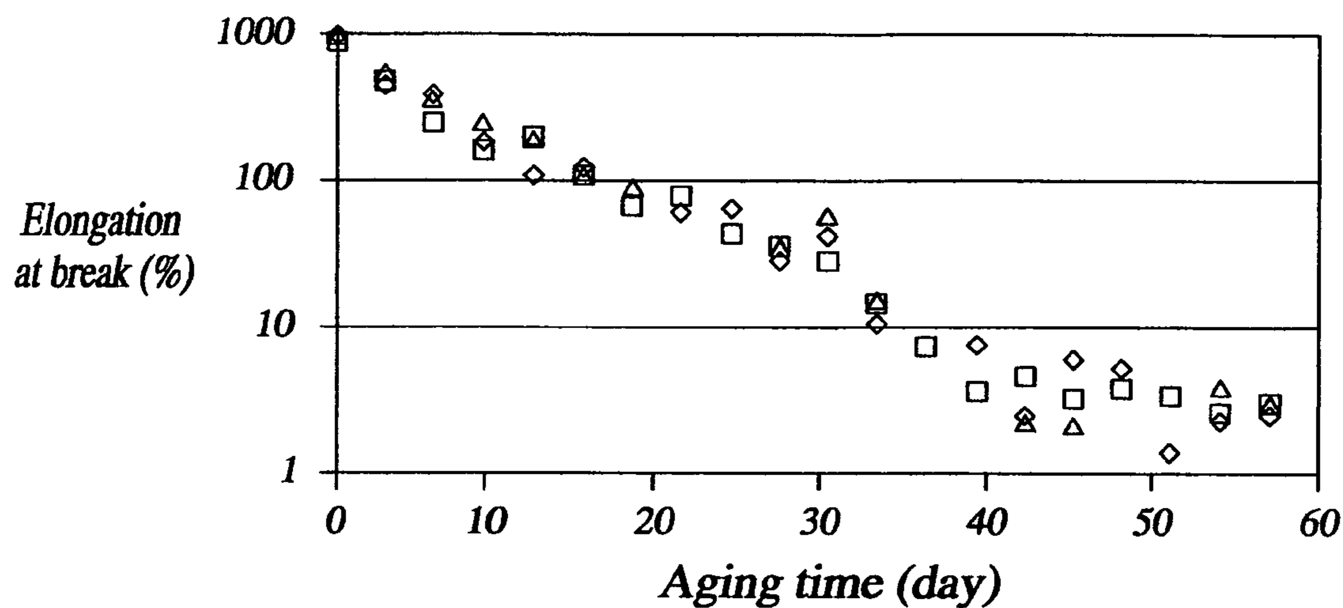
Elongation at break versus aging time for sample with 25% carbon black
