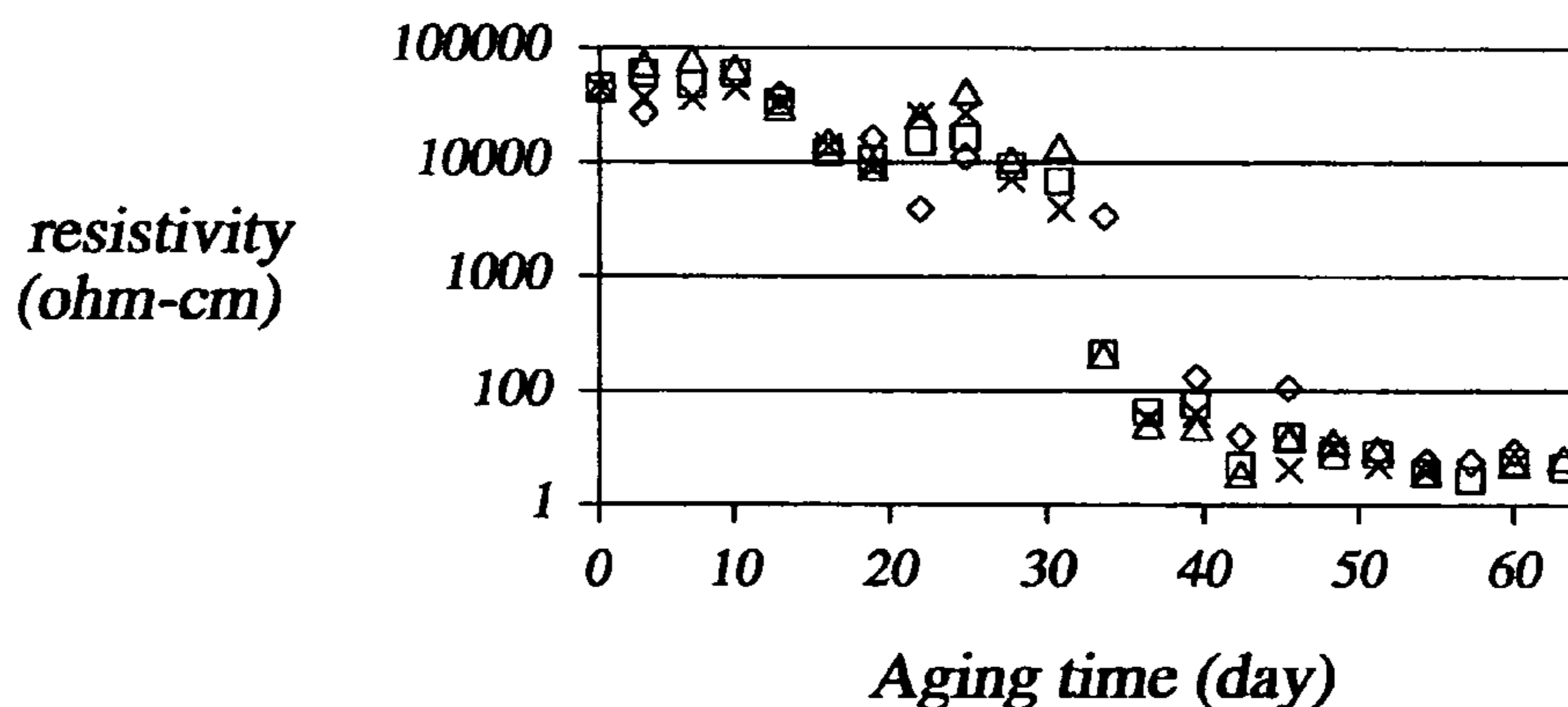
Restivity versus aging time for sample with 25% carbon black loading (aging temperature: 125C, measured one day after the sample was taken out)
