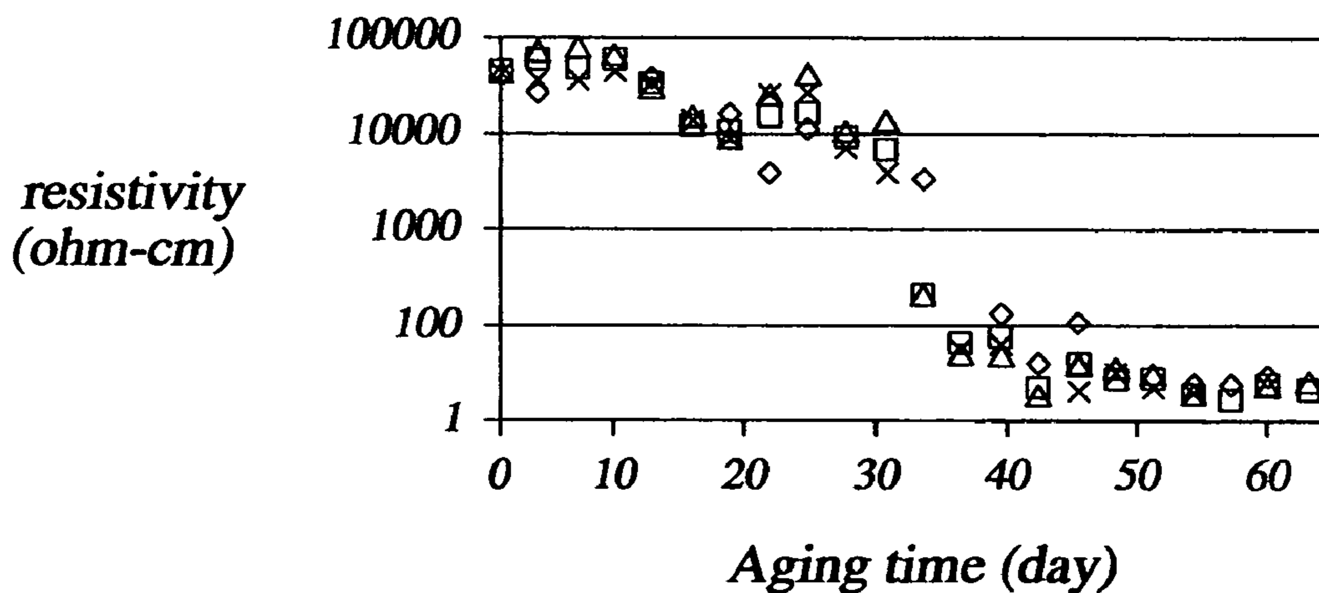
Restivitivity versus aging time for sample with 25% carbon black loading (aging temperature: 125C, measured one day after the sample was taken out)
