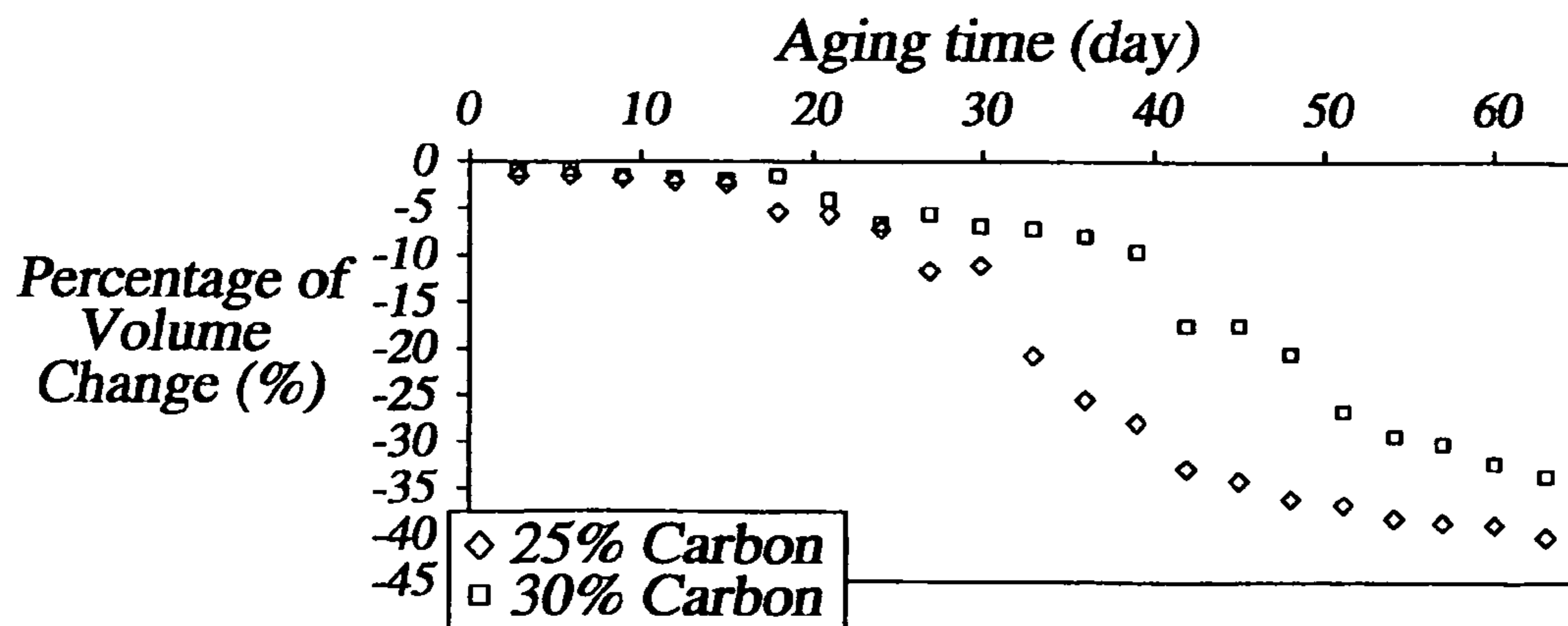
Volume Change versus Aging time
