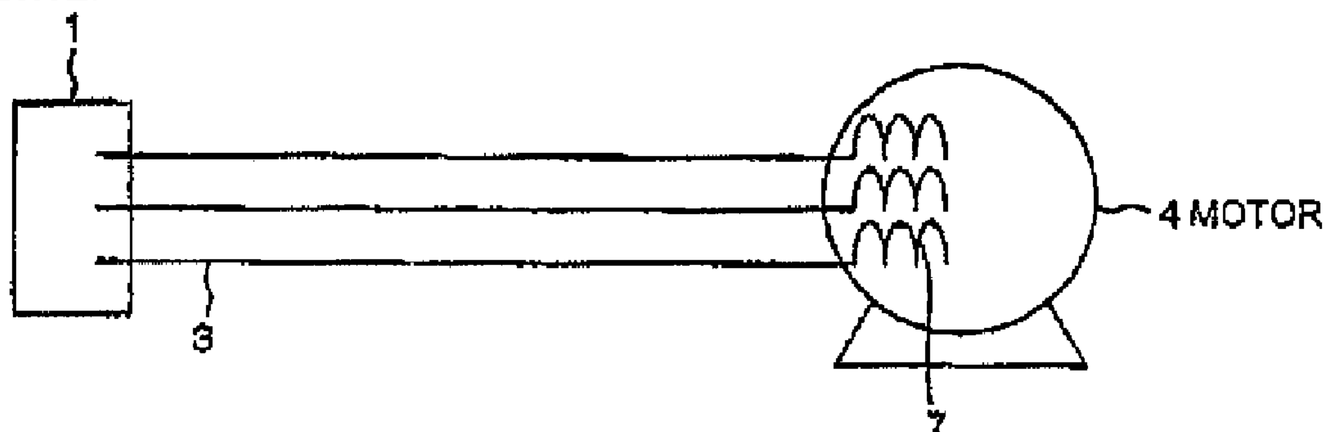
FREQUENCY CONVERTER
