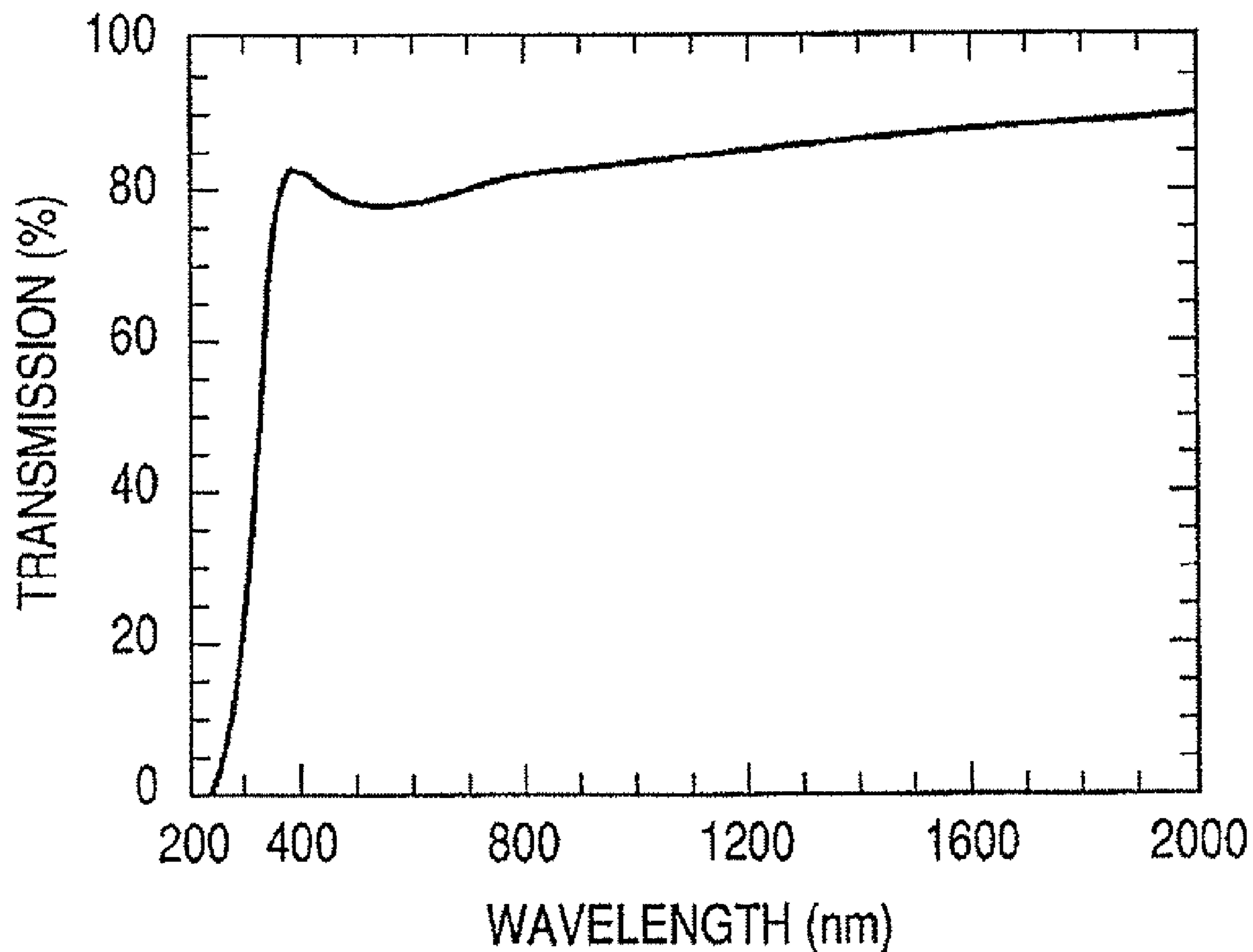
TRANSMISSION OF AMORPHOUS SEMICONDUCTOR LAYER (200nm) COMPRISED OF In-Ga-Zn-O
