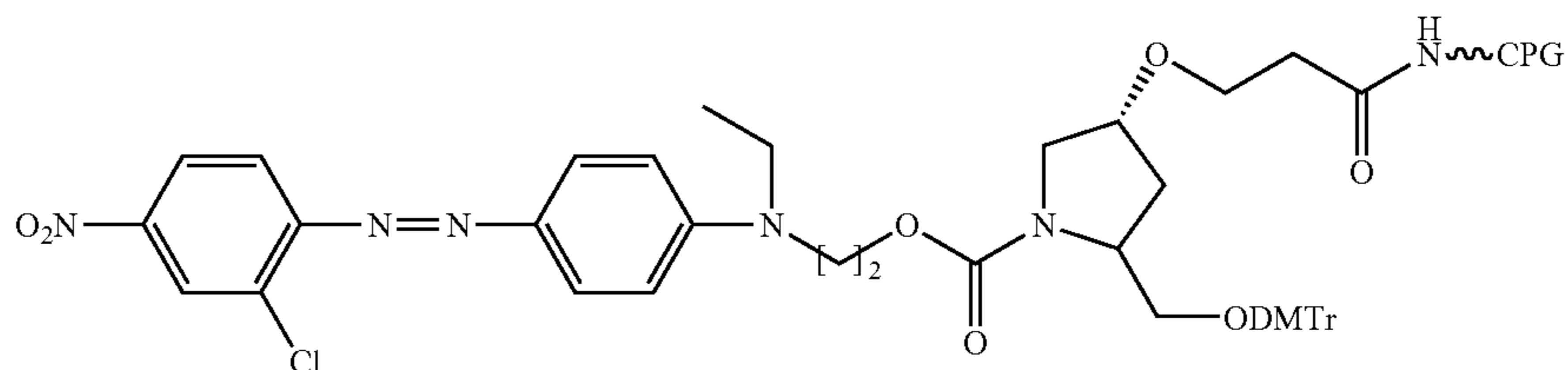
RED 13-pyrrolidine-DMTr-CPG, 12
