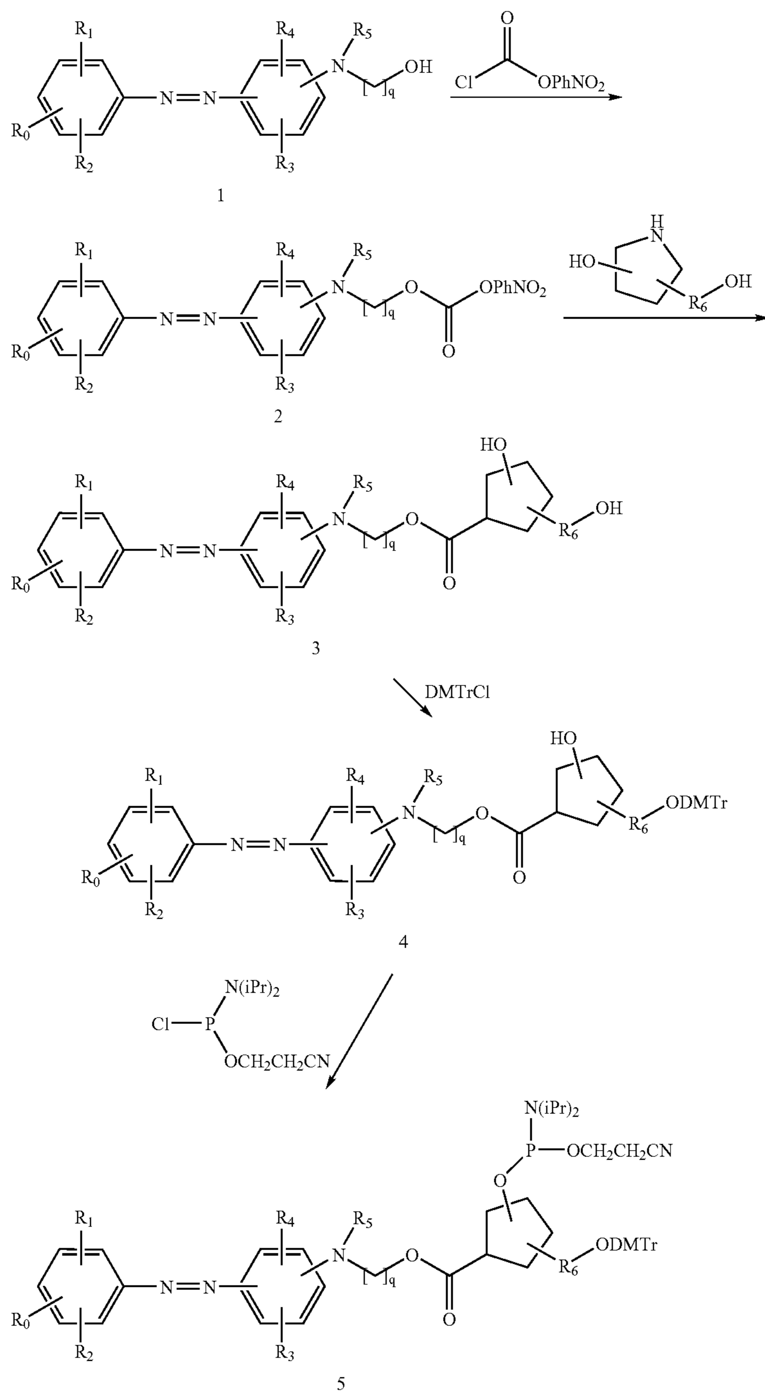
REACTION SCHEME 1
