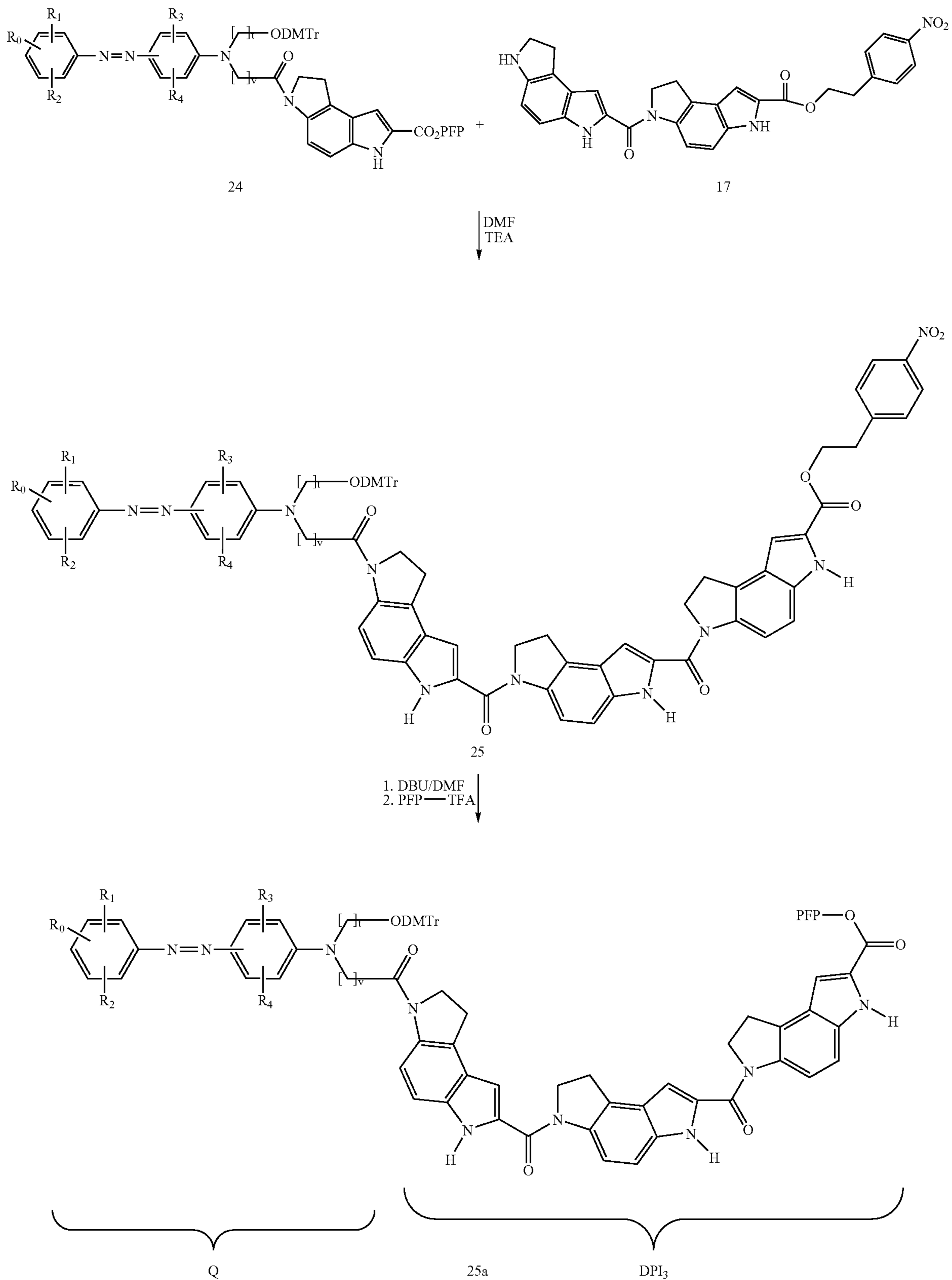
REACTION SCHEME 6
