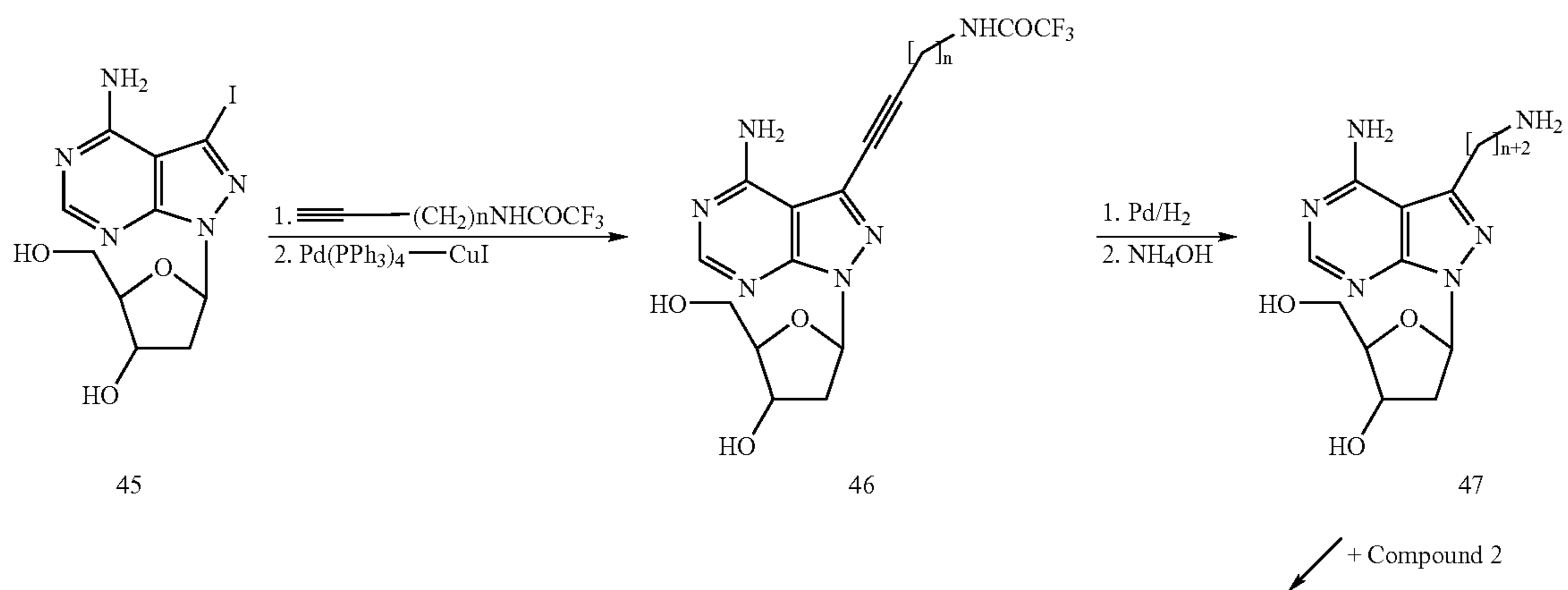
REACTION SCHEME 11
