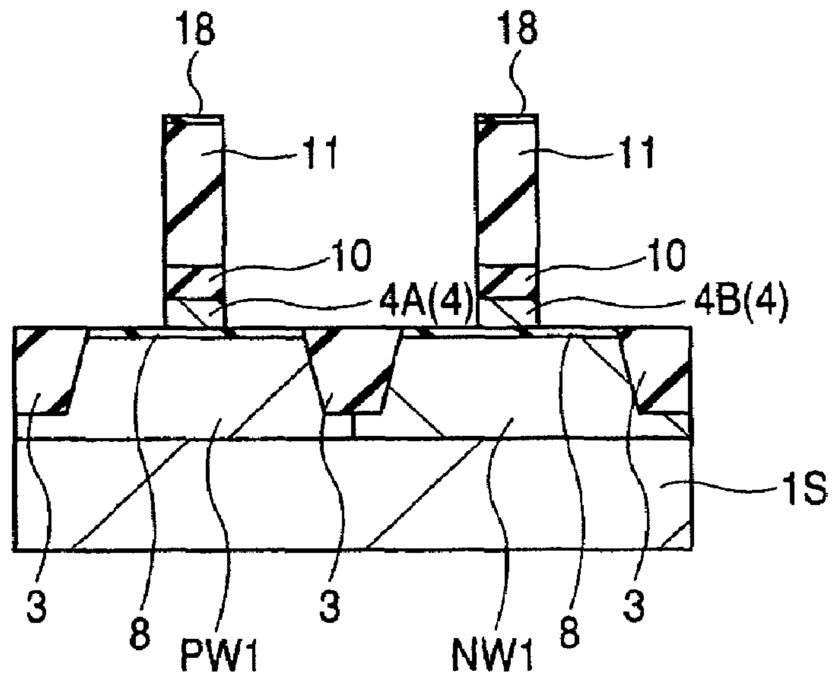
FIG. 71 PERIPHERAL CIRCUIT REGION
