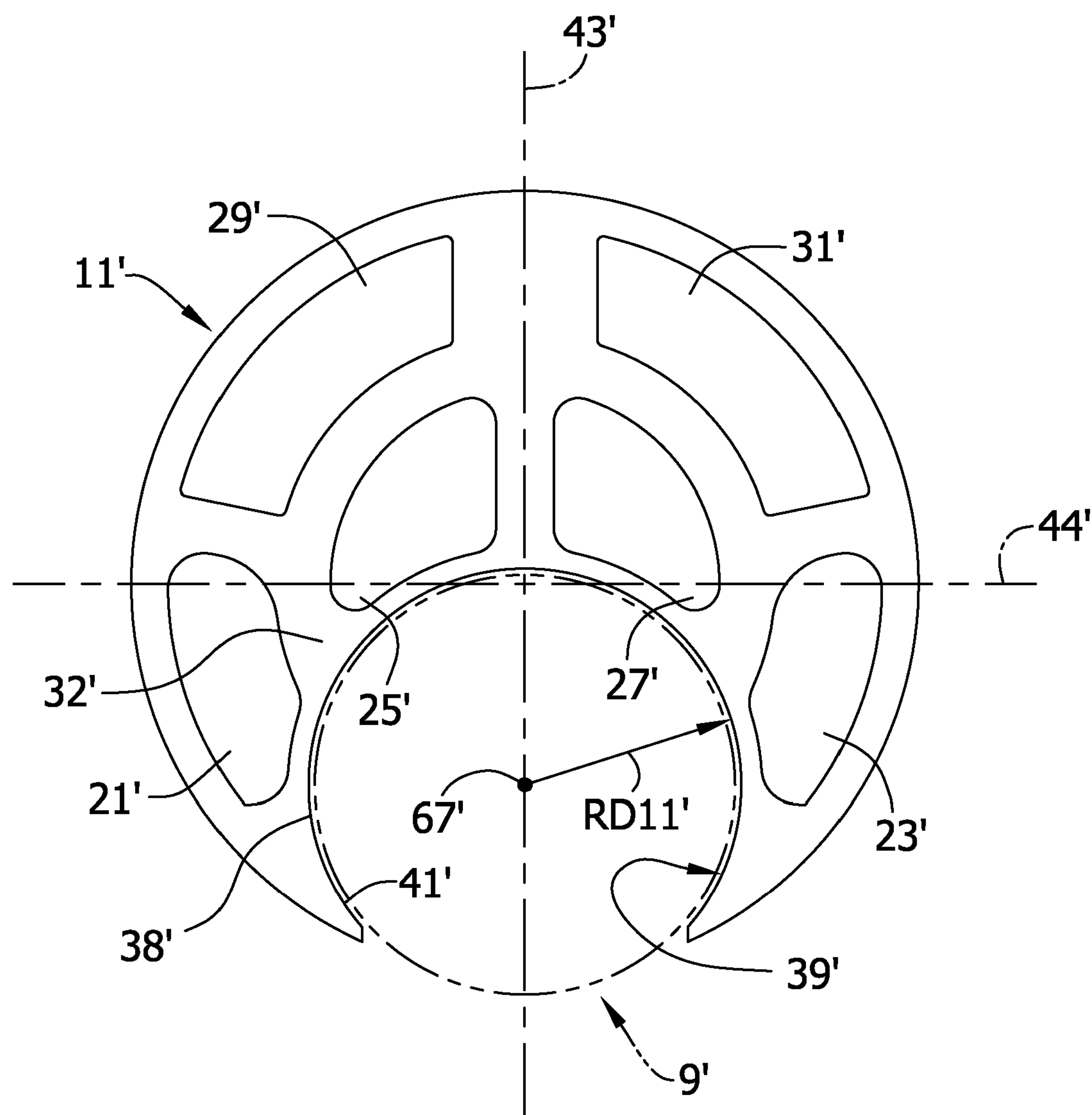
FIG. 4 PRIOR ART
