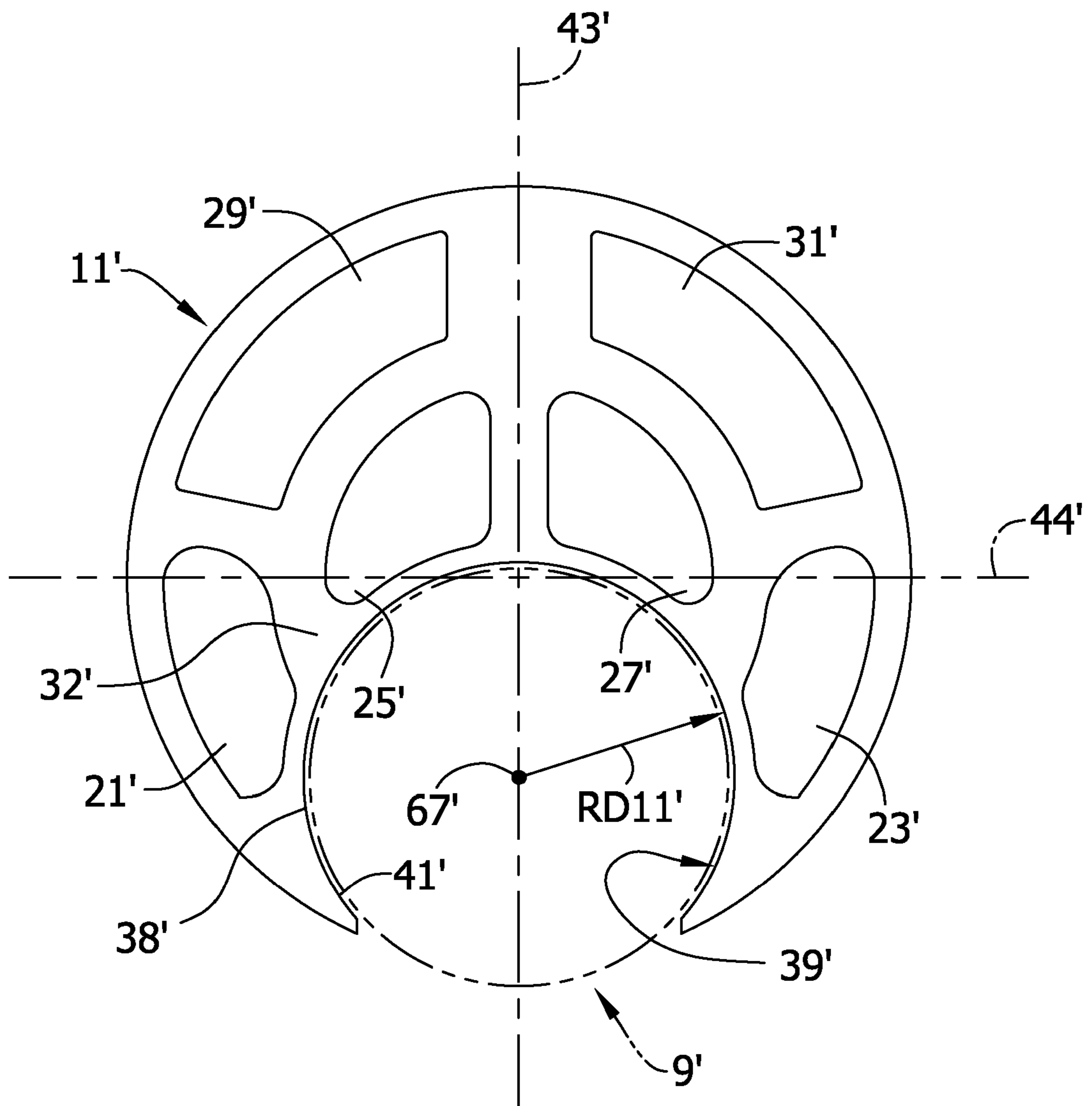
FIG. 4 PRIOR ART
