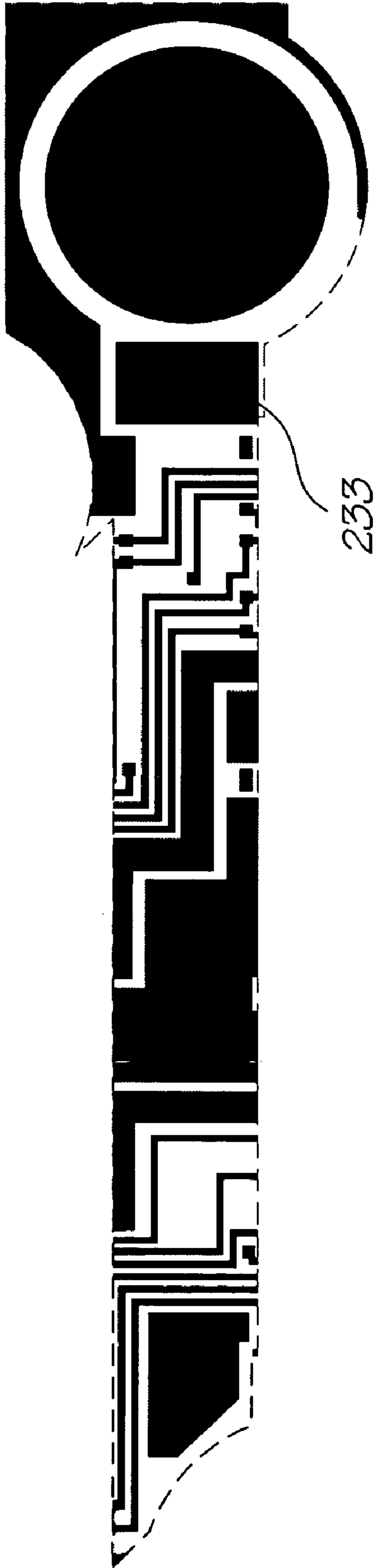
Metal 2 mask
