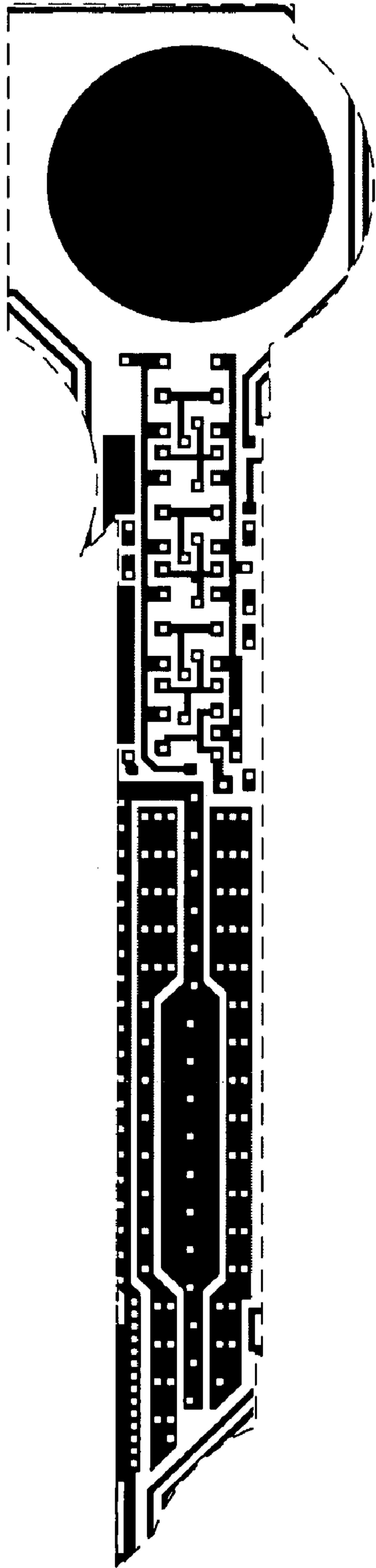
Metal 1 mask
