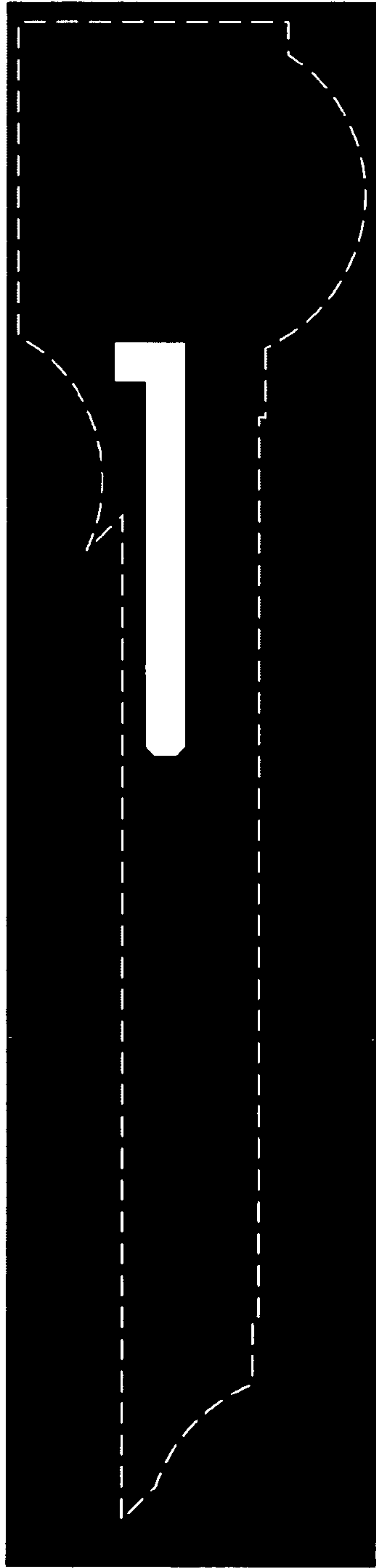
N-Well mask
