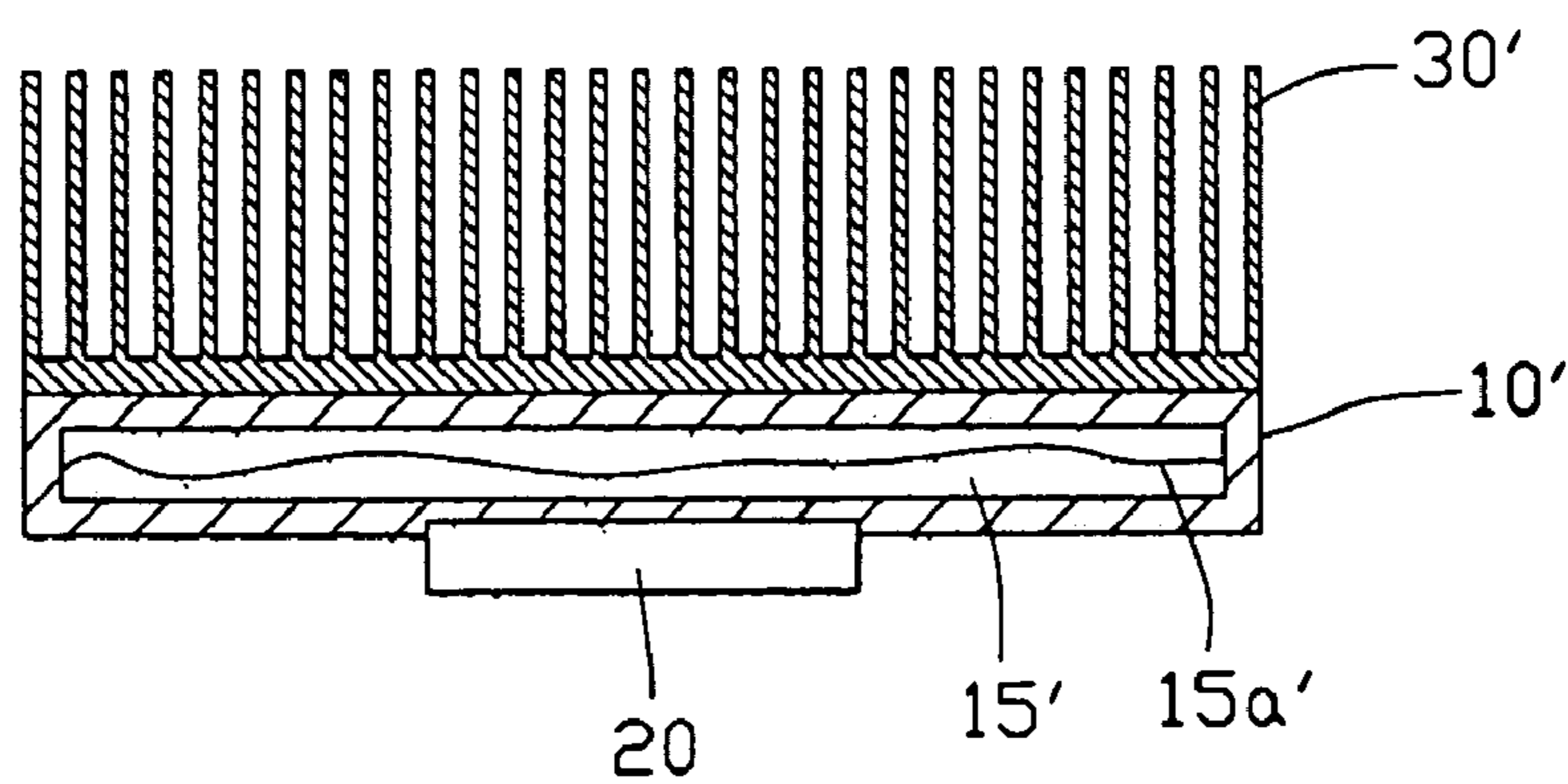
FIG. 14 (RELATED ART)
