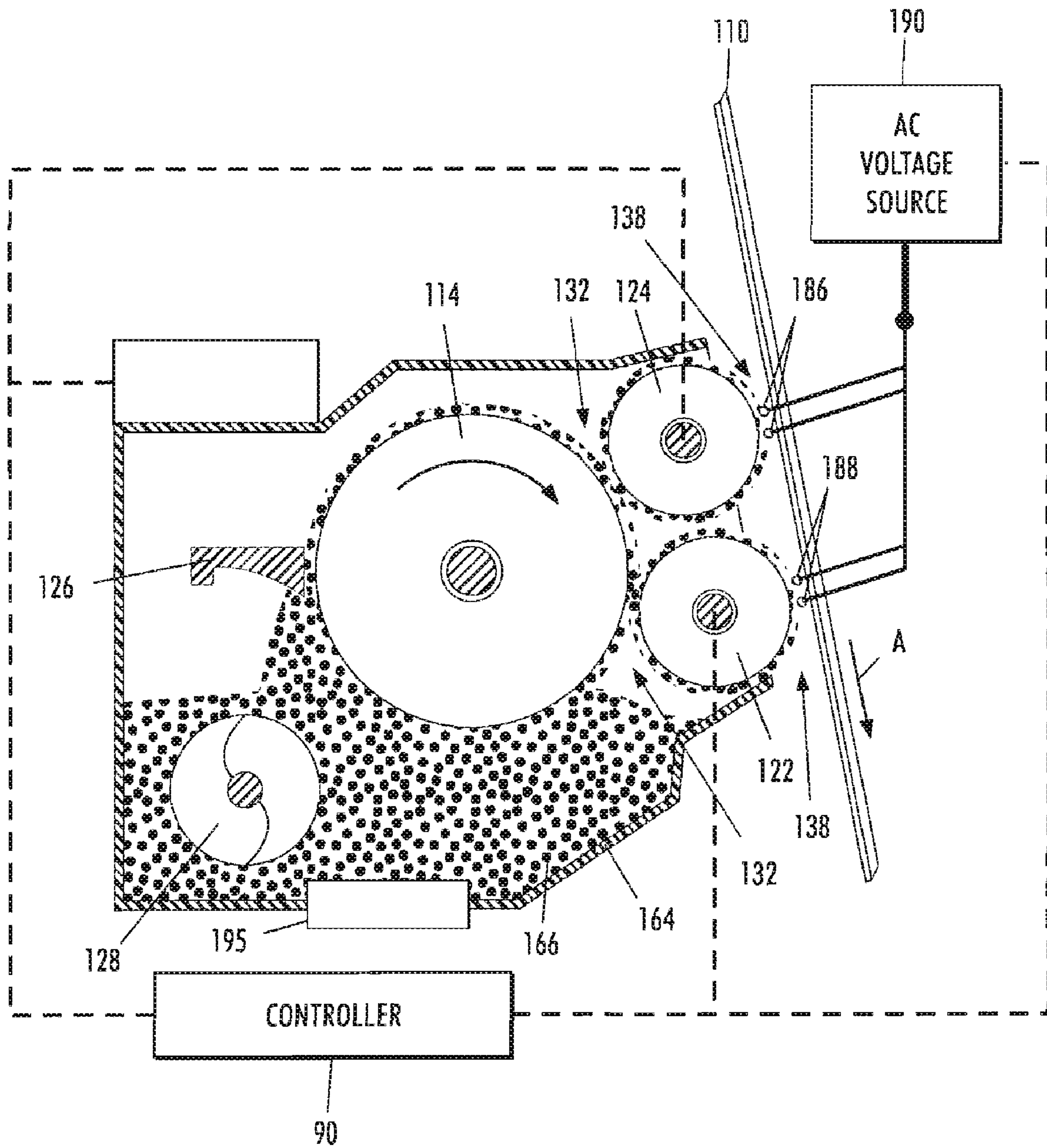
FIG. 1 PRIOR ART
