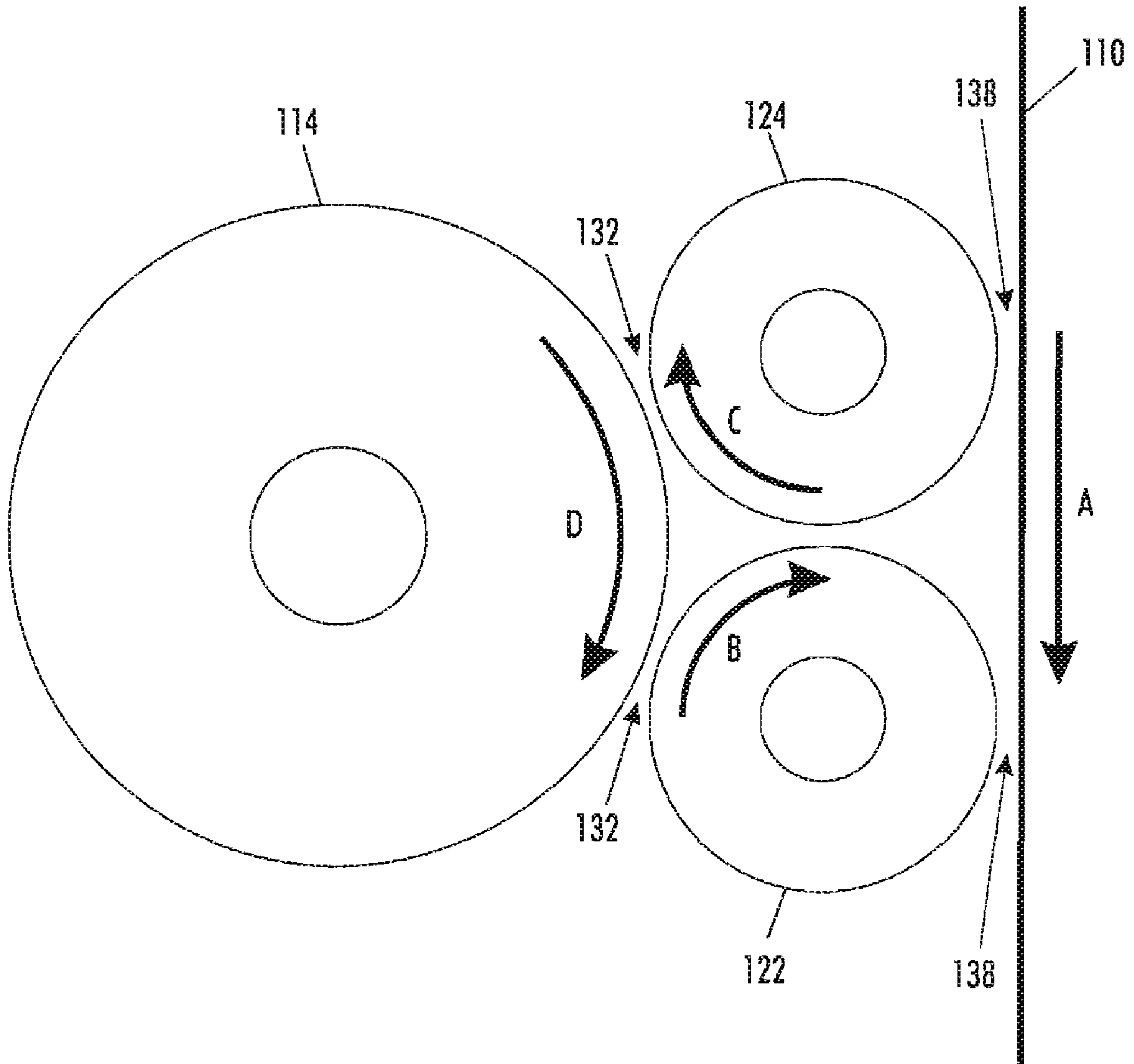
FIG. 2 PRIOR ART
