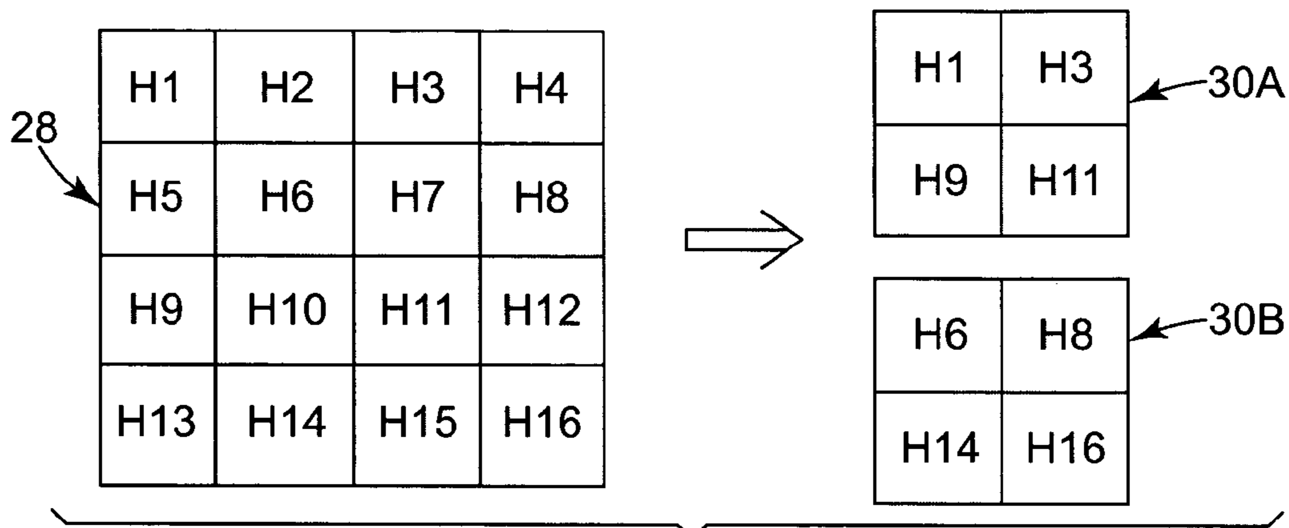
Fig. 5 (NEAREST NEIGHBOR)
