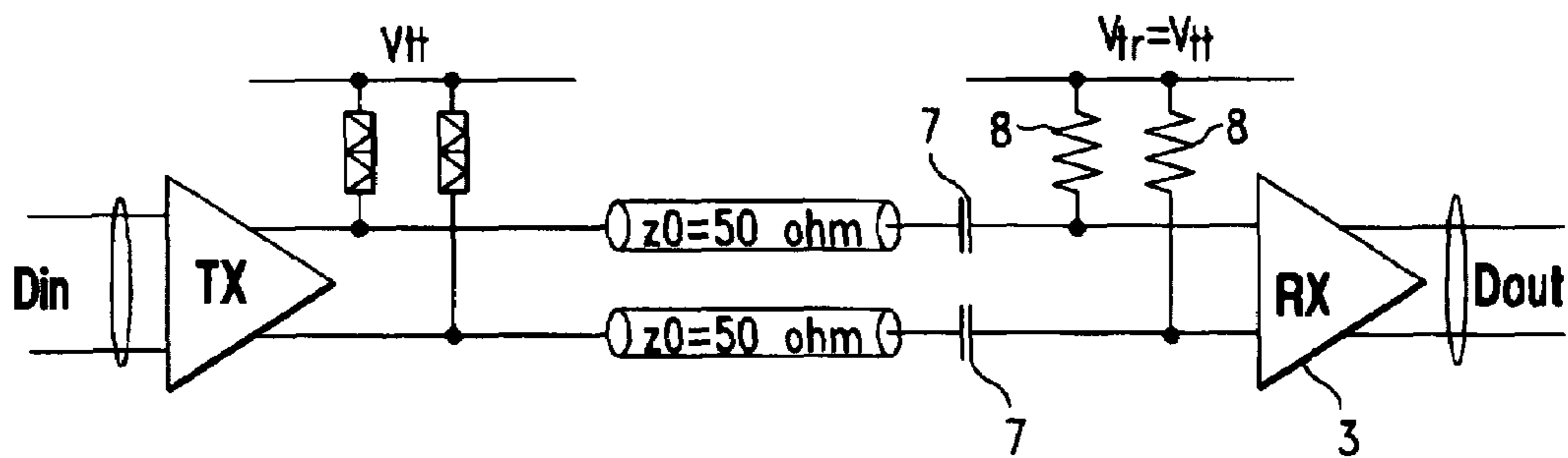
AC Coupling
