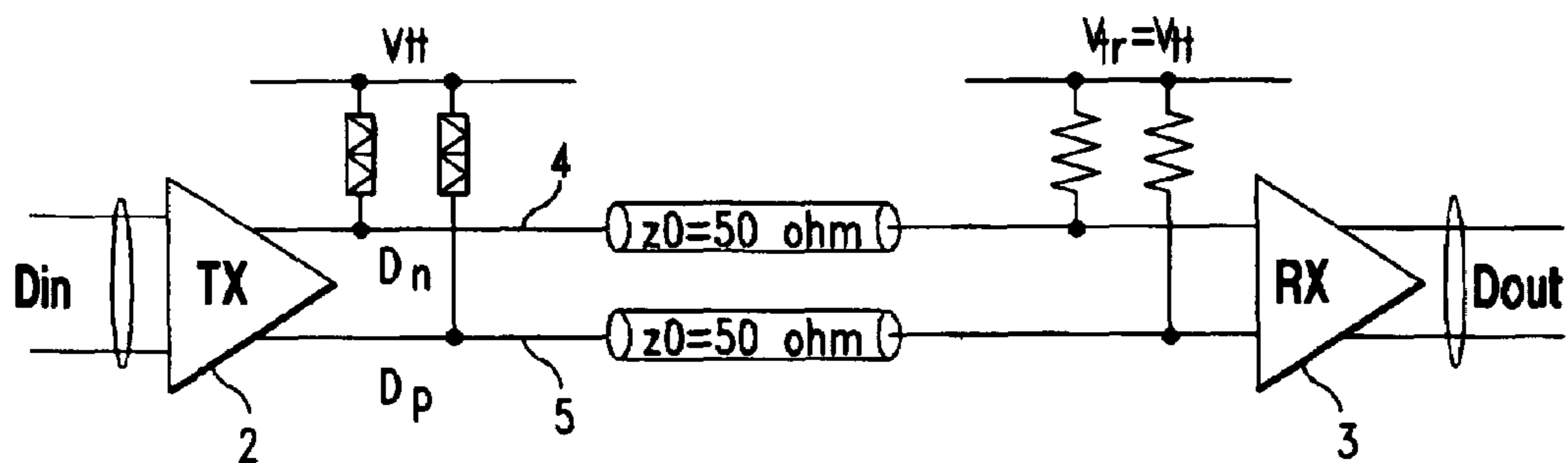
DC Coupling
